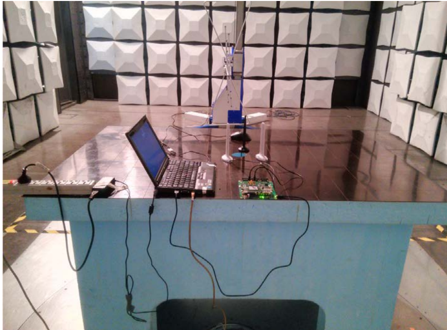
Radiated Disturbance Emissions (below 1GHz)
