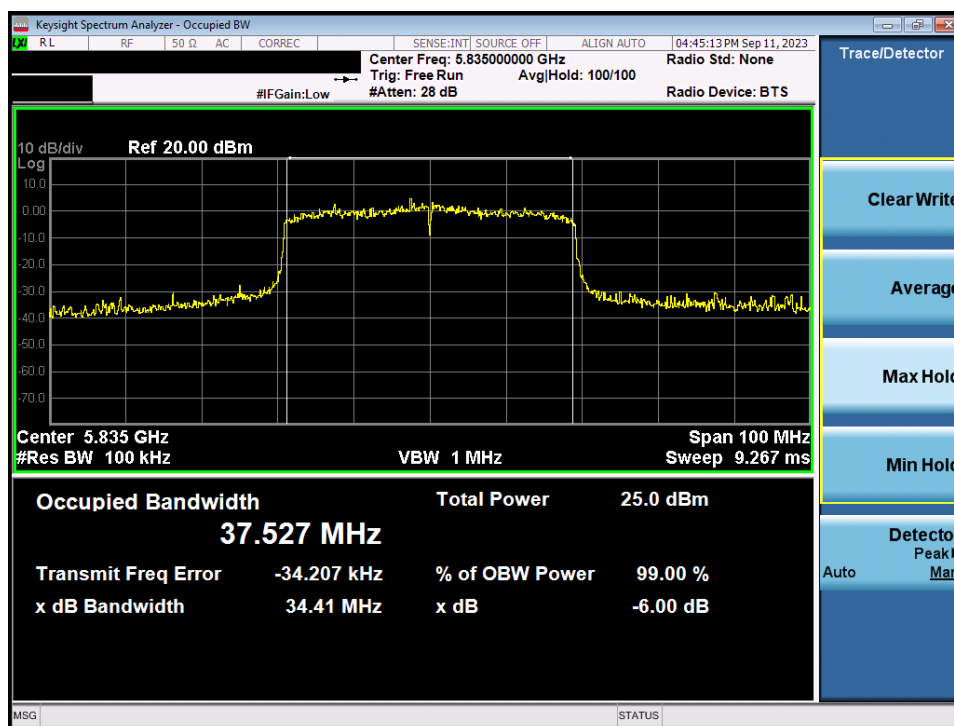
Plot 7-78. 6dB Bandwidth Plot MIMO ANT2 (40MHz BW 802.11ax/be (UNII Band 3/4) – Ch. 167)
