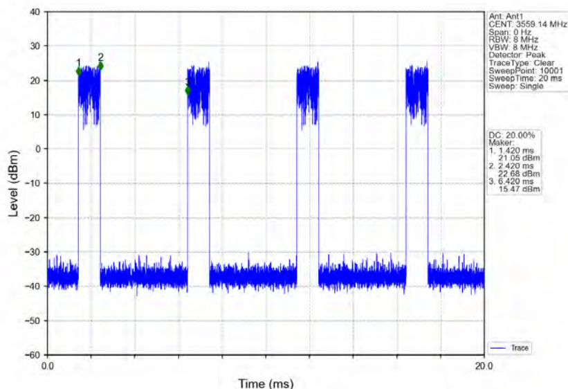
n48_30kHz_MIMO_NTNV_10MHz_CP-OFDM_256_QAM_3555MHz_Edge_1RB_Right
