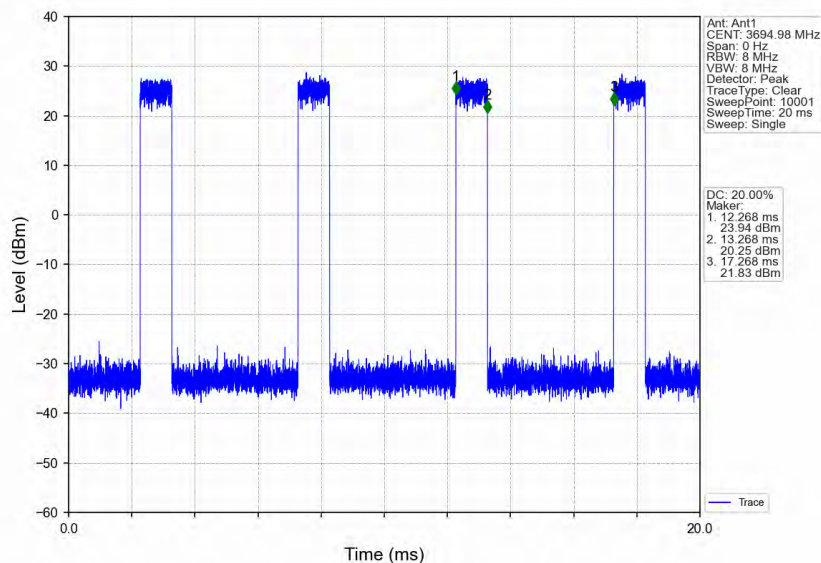
n48_30kHz_MIMO_NTNV_10MHz_CP-OFDM_64_QAM_3694.98MHz_Inner_Full
