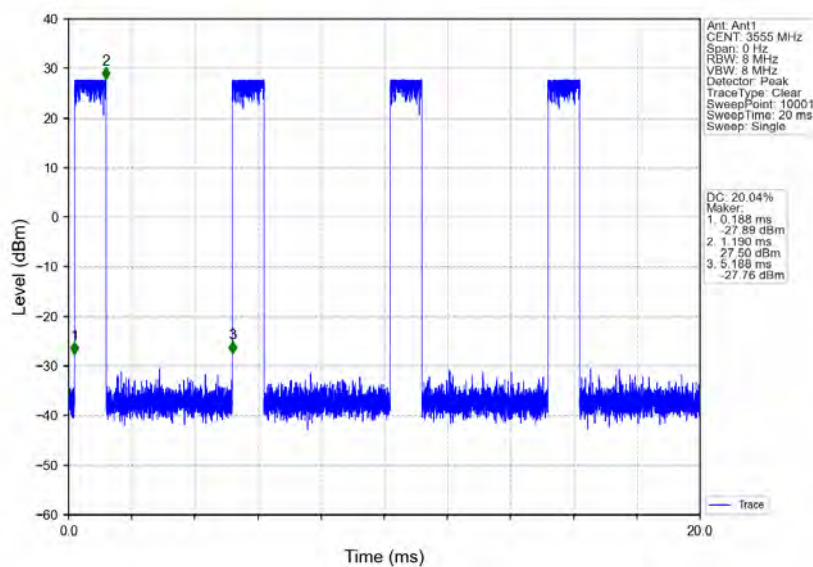
n48_30kHz_MIMO_NTNV_10MHz_CP-OFDM_QPSK_3555MHz_Inner_Full
