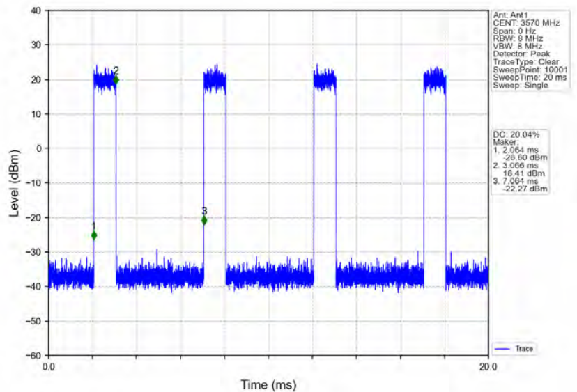
n48_30kHz_MIMO_NTNV_40MHz_CP-OFDM_64_QAM_3570MHz_Inner_Full
