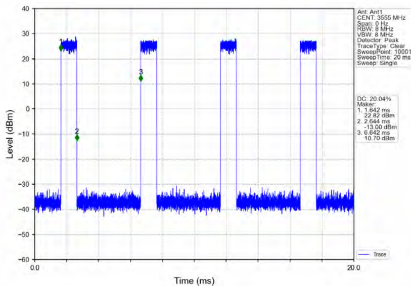
n48_30kHz_MIMO_NTNV_10MHz_CP-OFDM_QPSK_3555MHz_Inner_Full
