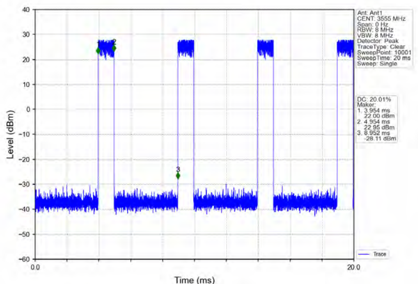
n48_30kHz_MIMO_NTNV_10MHz_CP-OFDM_64_QAM_3555MHz_Inner_Full
