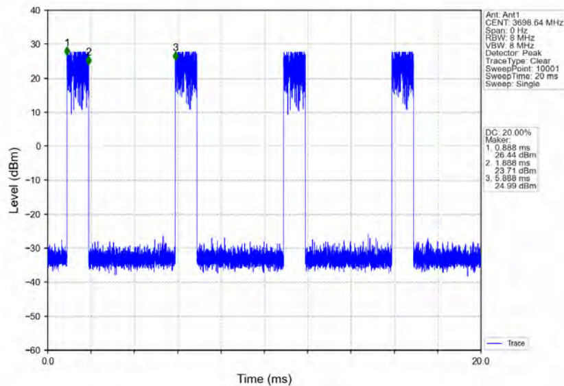
n48_30kHz_MIMO_NTNV_20MHz_CP-OFDM_QPSK_3690MHz_Inner_1RB_Right
