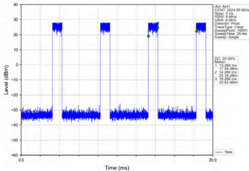
n48_30kHz_MIMO_NTNV_10MHz_CP-OFDM_64_QAM_3624.99MHz_Inner_Full
