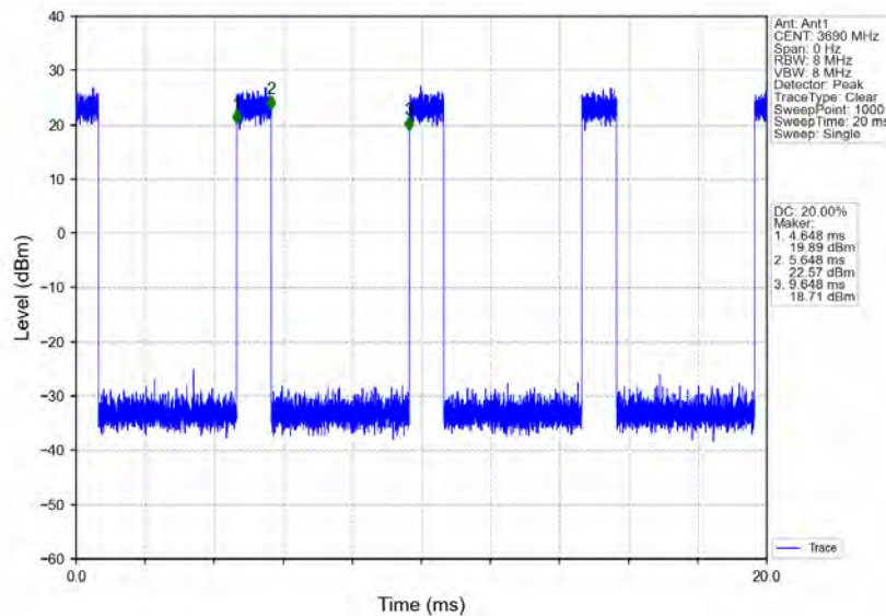
n48_30kHz_MIMO_NTNV_20MHz_CP-OFDM_16_QAM_3690MHz_Inner_Full
