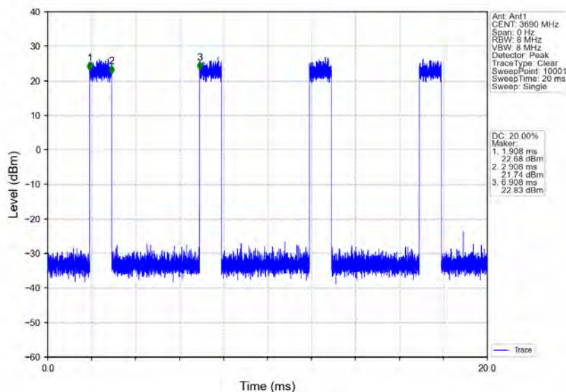
n48_30kHz_MIMO_NTNV_20MHz_CP-OFDM_64_QAM_3690MHz_Inner_Full
