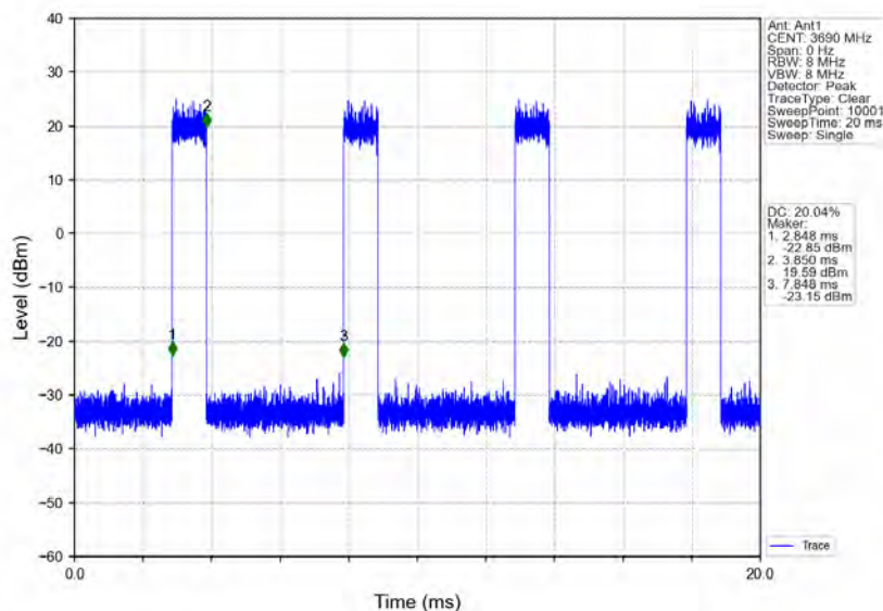
n48_30kHz_MIMO_NTNV_20MHz_CP-OFDM_256_QAM_3690MHz_Inner_Full
