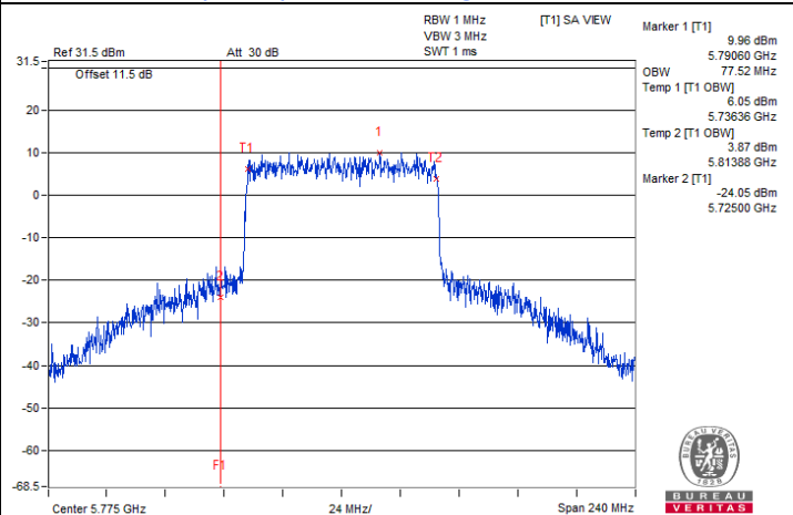
802.11ax (HE80) Beamforming / Chain 3 : CH 155
