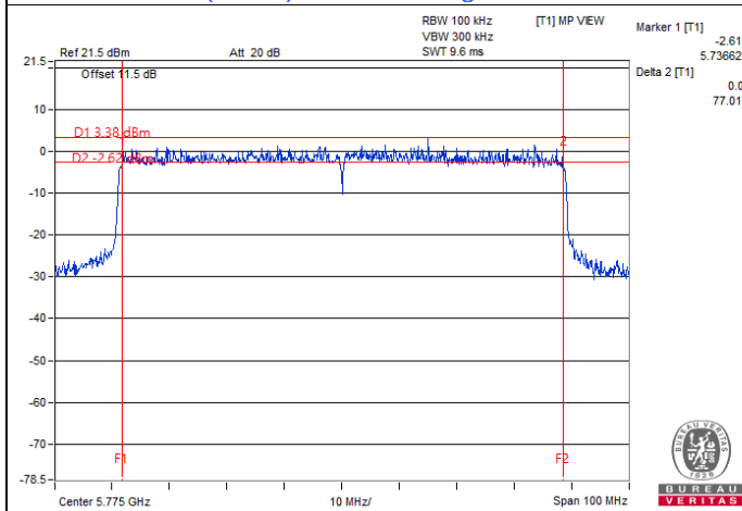
802.11ax (HE80) Beamforming / Chain0 : CH 155
