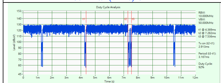
802.11ax (HE20) Beamforming
