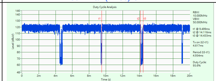
802.11ax (HE40) Beamforming
