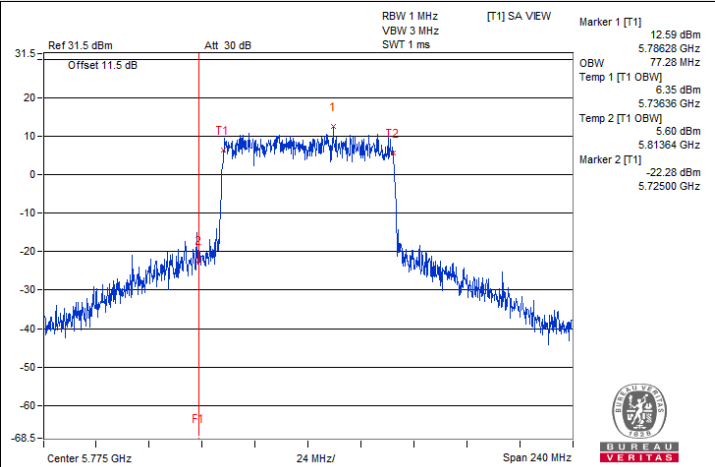
802.11ax (HE80) Beamforming / Chain 1 : CH 155
