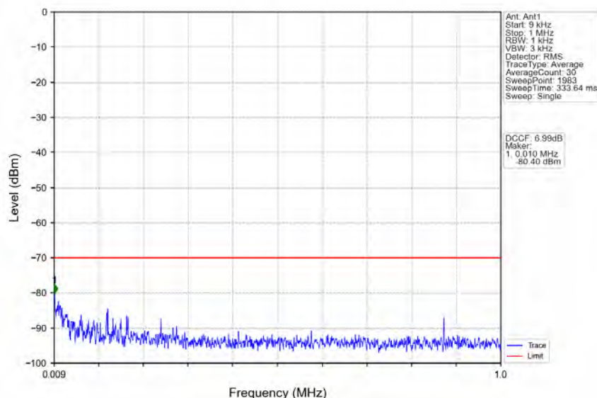
n48_30kHz_MIMO_NTNV_20MHz_CP-OFDM_QPSK_3560.01MHz_Inner_1RB_Left
