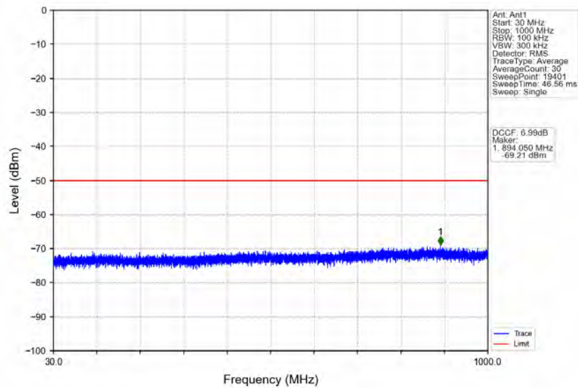
n48_30kHz_MIMO_NTNV_40MHz_CP-OFDM_QPSK_3679.98MHz_Edge_1RB_Right
