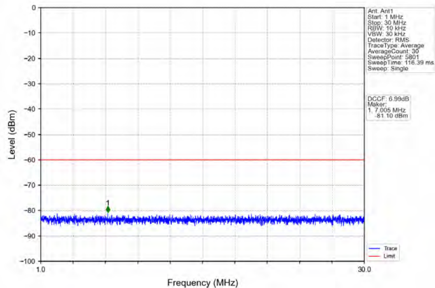
n48_30kHz_MIMO_NTNV_40MHz_CP-OFDM_QPSK_3570MHz_Outer_Full
