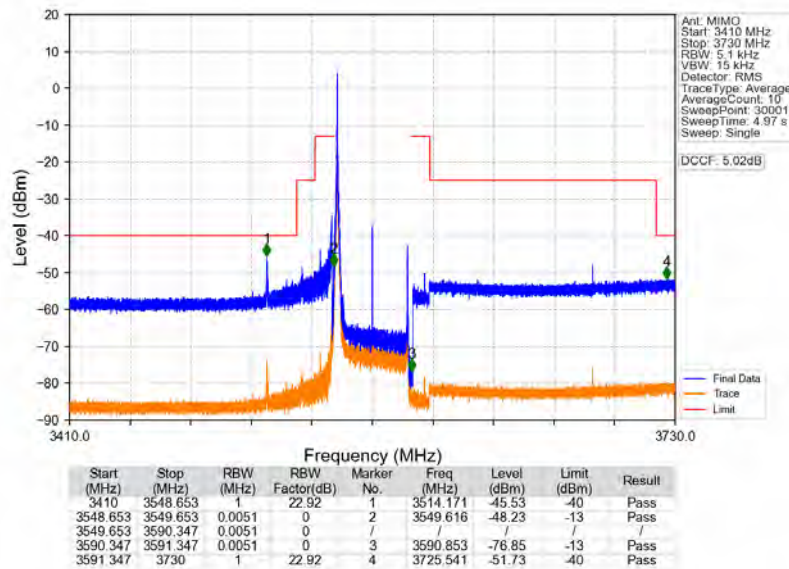
n48_30kHz_MIMO_NTNV_40MHz_CP-OFDM_QPSK_3570MHz_Inner_1RB_Left
