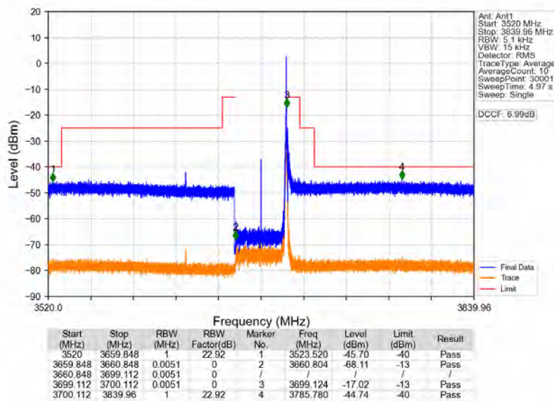
n48_30kHz_MIMO_NTNV_40MHz_CP-OFDM_QPSK_3679.98MHz_Edge_1RB_Right
