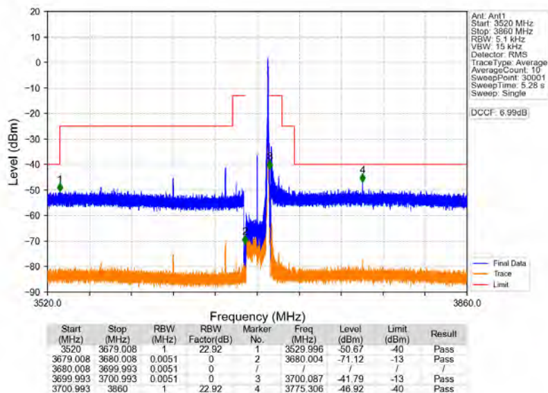
n48_30kHz_MIMO_NTNV_20MHz_CP-OFDM_QPSK_3690MHz_Inner_1RB_Right
