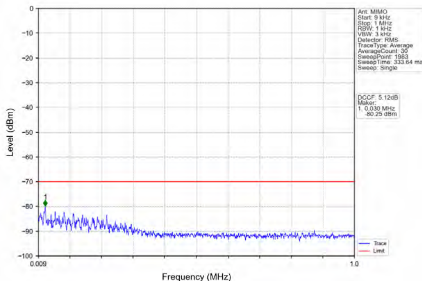
n48_30kHz_MIMO_NTNV_40MHz_CP-OFDM_QPSK_3679.98MHz_Inner_1RB_Right
