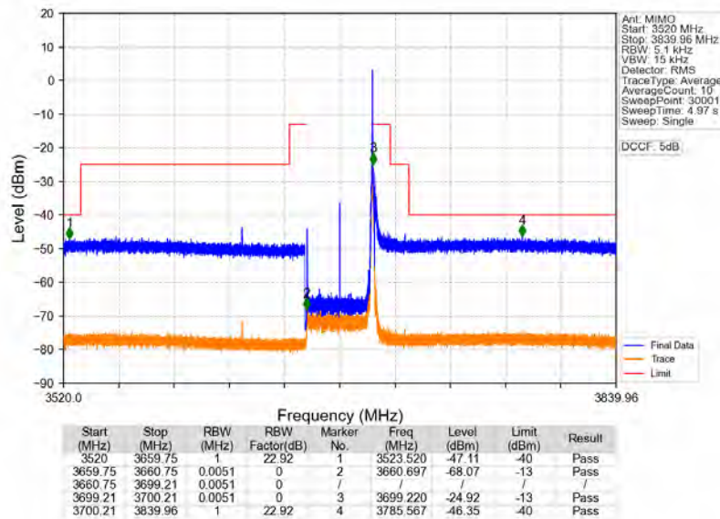
n48_30kHz_MIMO_NTNV_40MHz_CP-OFDM_QPSK_3679.98MHz_Edge_1RB_Right
