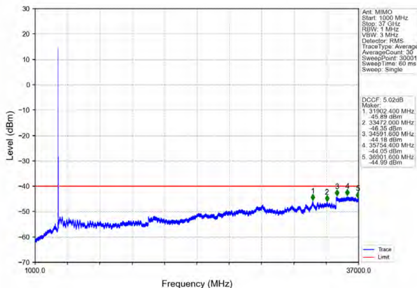
n48_30kHz_MIMO_NTNV_40MHz_CP-OFDM_QPSK_3679.98MHz_Edge_1RB_Right
