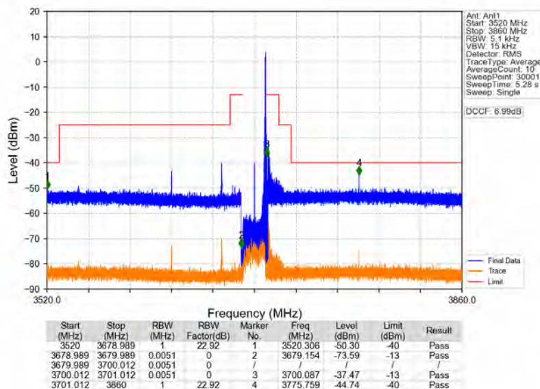
n48_30kHz_MIMO_NTNV_20MHz_CP-OFDM QPSK_3690MHz_Edge_1RB_Right
