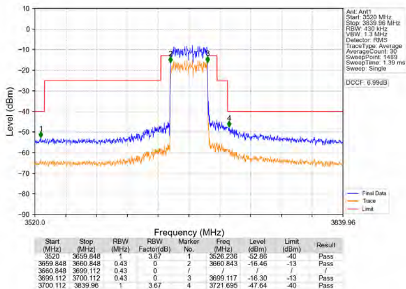
n48_30kHz_MIMO_NTNV_40MHz_CP-OFDM_QPSK_3679.98MHz_Outer_Full
