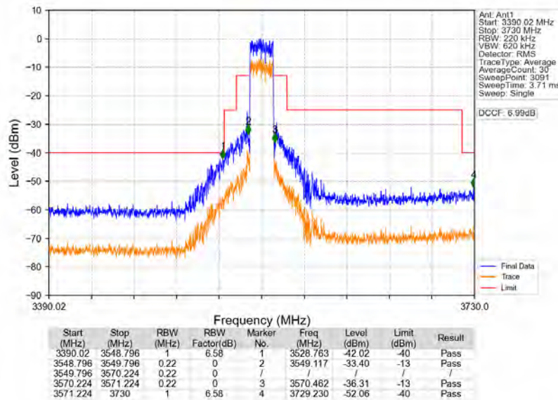
n48_30kHz_MIMO_NTNV_20MHz_CP-OFDM_QPSK_3560.01MHz_Outer_Full
