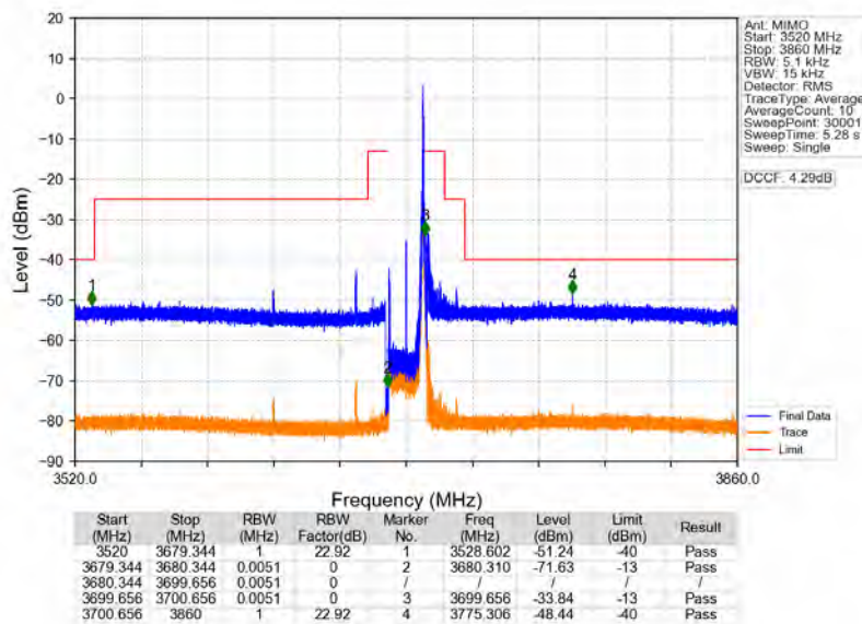
n48_30kHz_MIMO_NTNV_20MHz_CP-OFDM_QPSK_3690MHz_Inner_1RB_Right
