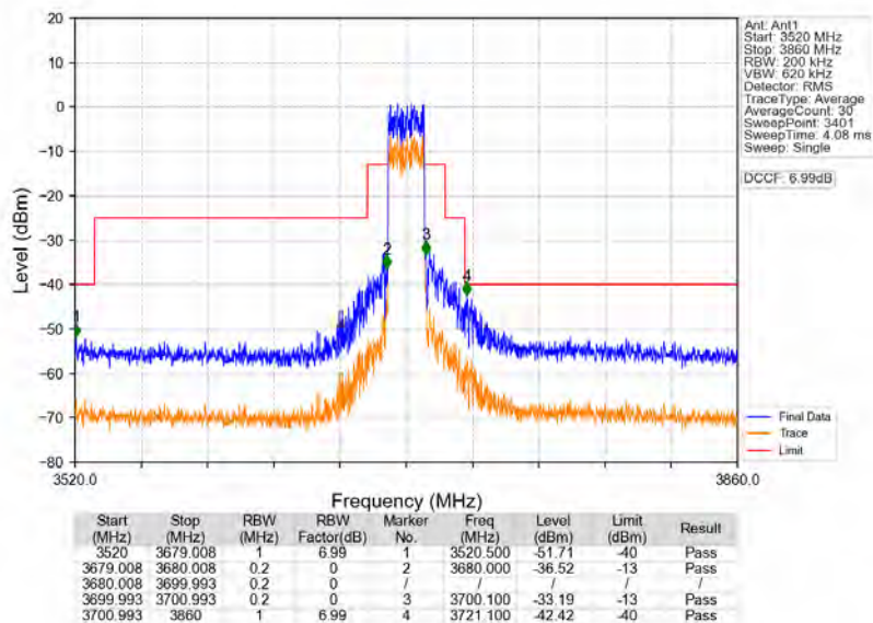
n48_30kHz_MIMO_NTNV_20MHz_CP-OFDM_QPSK_3690MHz_Outer_Full
