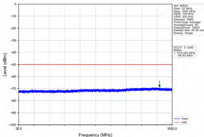
n48_30kHz_MIMO_NTNV_40MHz_CP-OFDM_QPSK_3679.98MHz_Inner_1RB_Right
