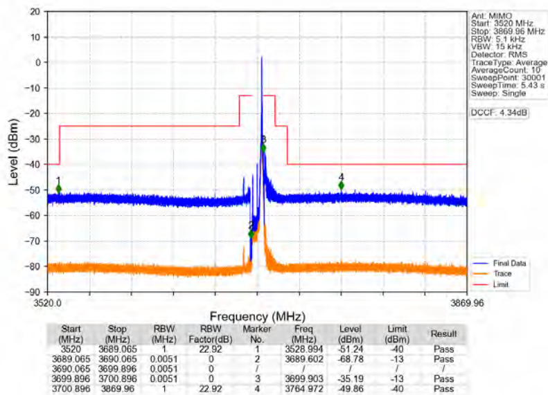
n48_30kHz_MIMO_NTNV_10MHz_CP-OFDM_QPSK_3694.98MHz_Inner_1RB_Right
