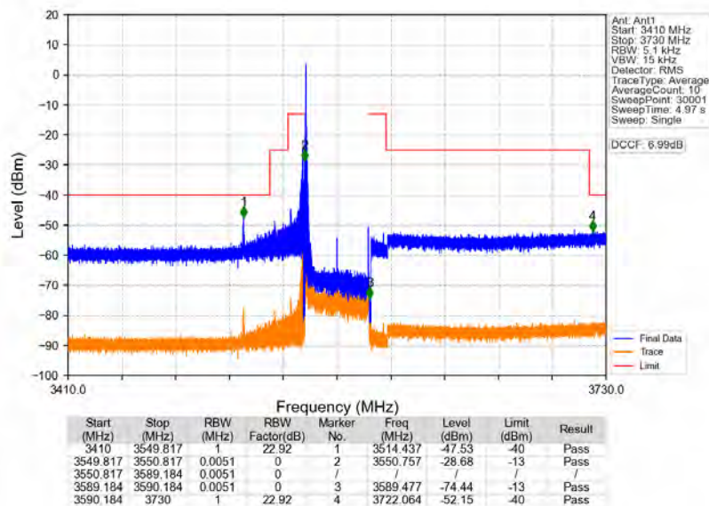
n48_30kHz_MIMO_NTNV_40MHz_CP-OFDM_QPSK_3570MHz_Inner_1RB_Left
