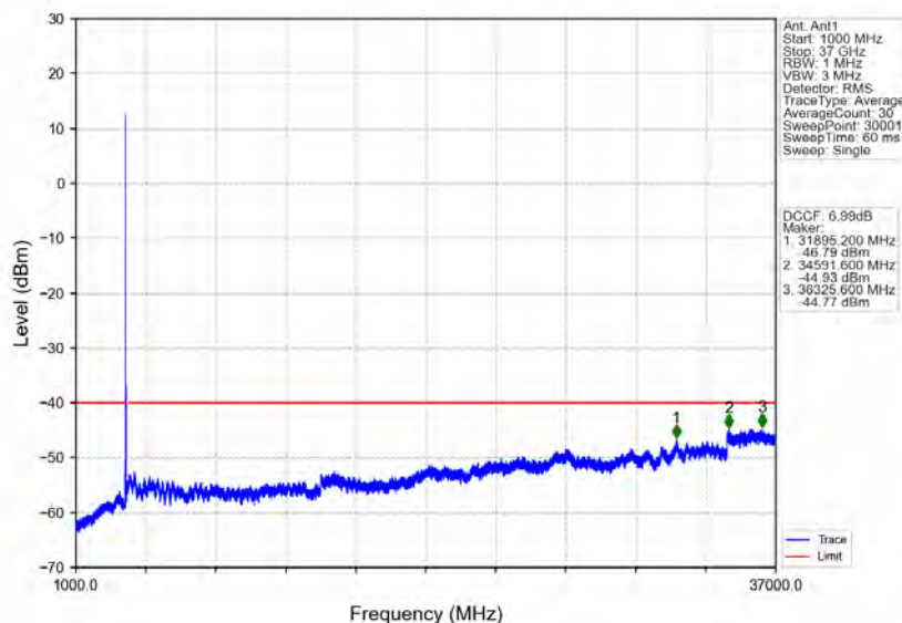
n48_30kHz_MIMO_NTNV_40MHz_CP-OFDM_QPSK_3570MHz_Inner_1RB_Left
