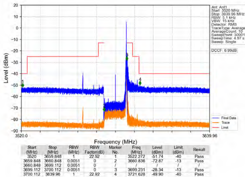
n48_30kHz_MIMO_NTNV_40MHz_CP-OFDM_QPSK_3679.98MHz_Inner_1RB_Right
