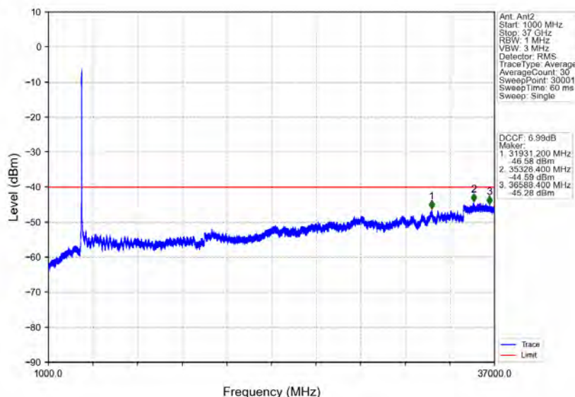
n48_30kHz_MIMO_NTNV_40MHz_CP-OFDM_QPSK_3679.98MHz_Outer_Full
