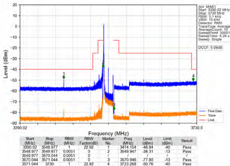
n48_30kHz_MIMO_NTNV_20MHz_CP-OFDM_QPSK_3560.01MHz_Edge_1RB_Left
