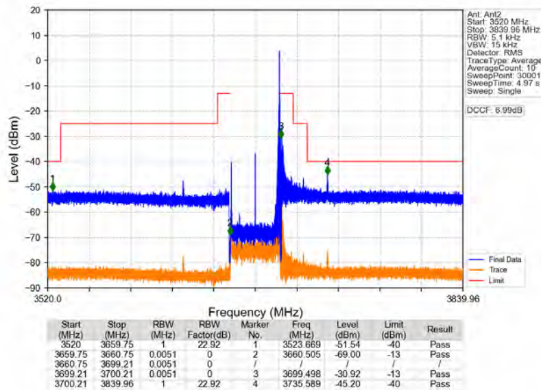
n48_30kHz_MIMO_NTNV_40MHz_CP-OFDM_QPSK_3679.98MHz_Inner_1RB_Right
