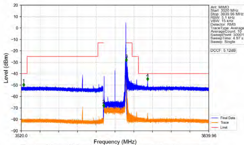
n48_30kHz_MIMO_NTNV_40MHz_CP-OFDM_QPSK_3679.98MHz_Inner_1RB_Right
