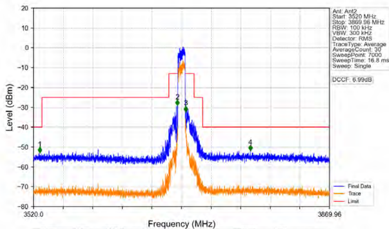
n48_30kHz_MIMO_NTNV_10MHz_CP-OFDM_QPSK_3694.98MHz_Outer_Full
