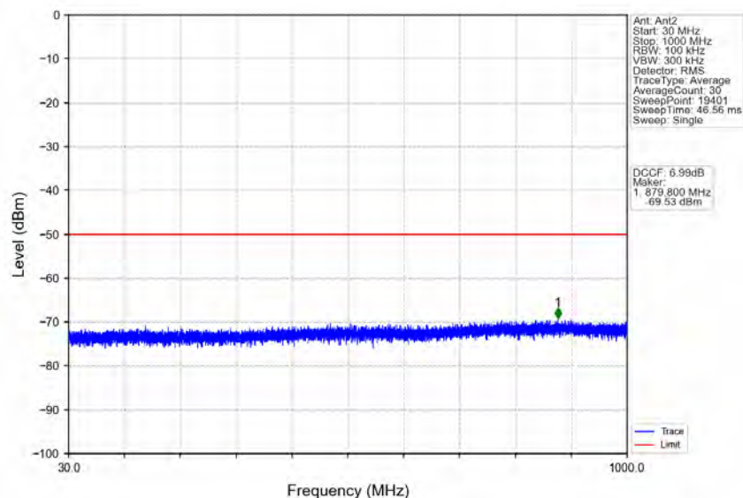
n48_30kHz_MIMO_NTNV_40MHz_CP-OFDM_QPSK_3679.98MHz_Outer_Full
