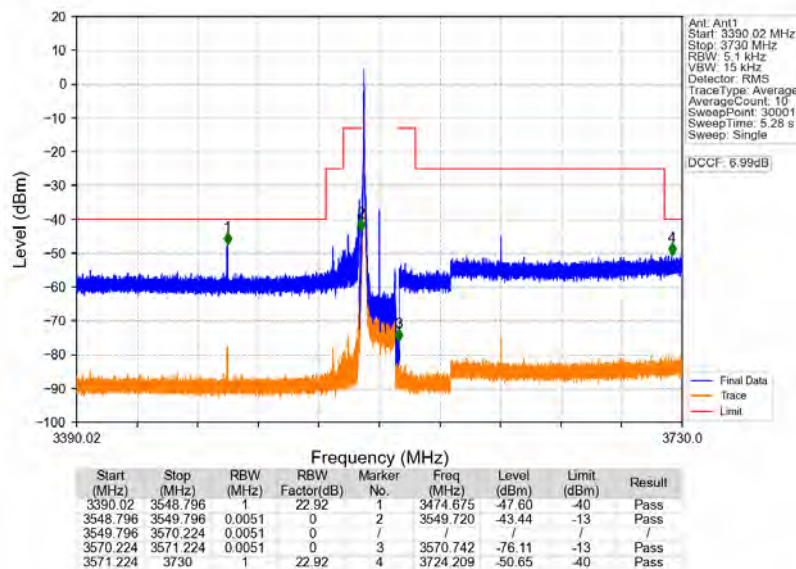
n48_30kHz_MIMO_NTNV_20MHz_CP-OFDM_QPSK_3560.01MHz_Inner_1RB_Left
