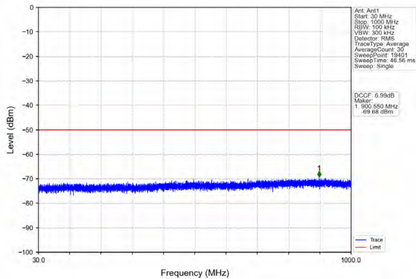
n48_30kHz_MIMO_NTNV_40MHz_CP-OFDM_QPSK_3570MHz_Outer_Full
