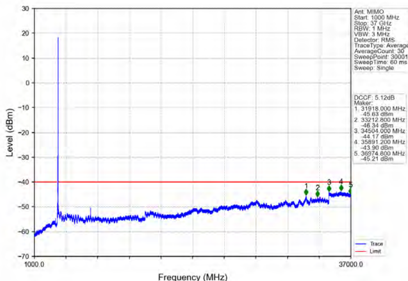
n48_30kHz_MIMO_NTNV_40MHz_CP-OFDM_QPSK_3679.98MHz_Inner_1RB_Right
