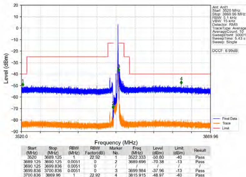
n48_30kHz_MIMO_NTNV_10MHz_CP-OFDM_QPSK_3694.98MHz_Inner_1RB_Right
