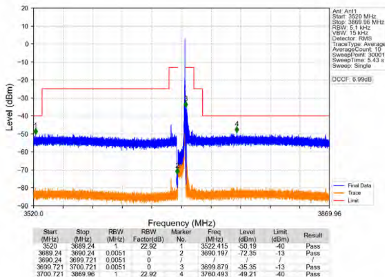
n48_30kHz_MIMO_NTNV_10MHz_CP-OFDM_QPSK_3694.98MHz_Edge_1RB_Right
