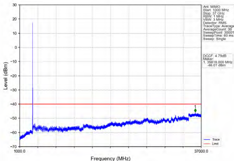
n48_30kHz_MIMO_NTNV_40MHz_CP-OFDM_QPSK_3570MHz_Outer_Full
