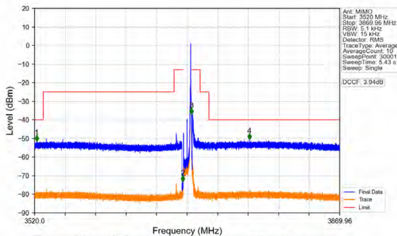
n48_30kHz_MIMO_NTNV_10MHz_CP-OFDM_QPSK_3694.98MHz_Edge_1RB_Right
