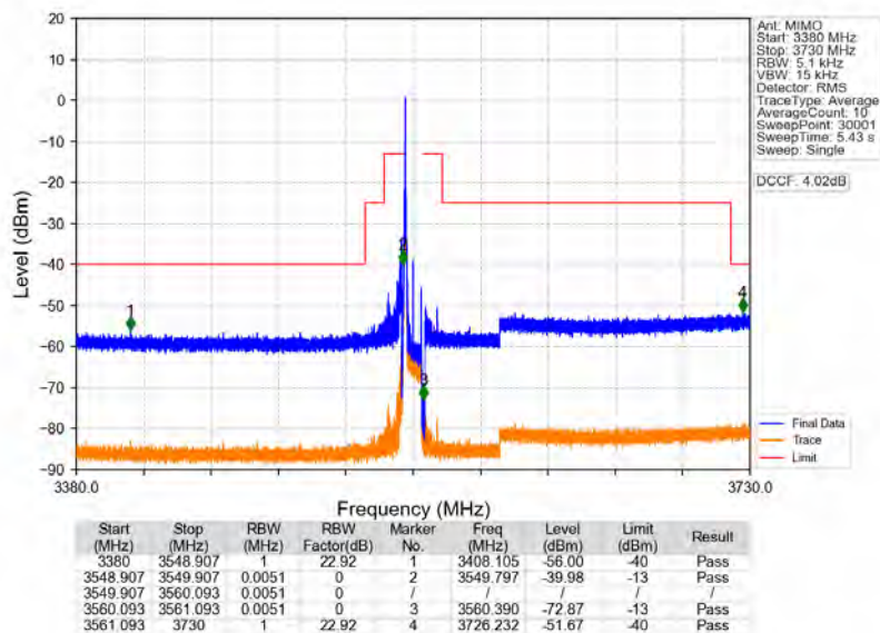
n48_30kHz_MIMO_NTNV_10MHz_CP-OFDM_QPSK_3555MHz_Edge_1RB_Left
