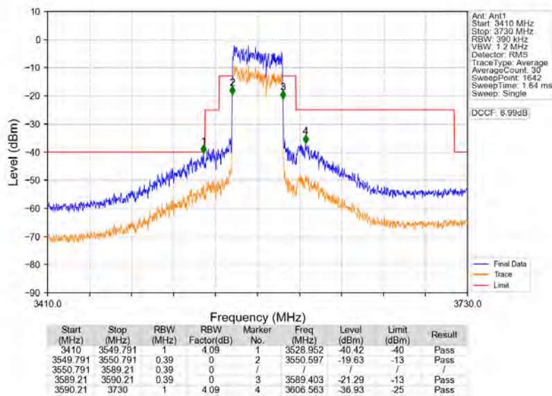
n48_30kHz_MIMO_NTNV_40MHz_CP-OFDM_QPSK_3570MHz_Outer_Full
