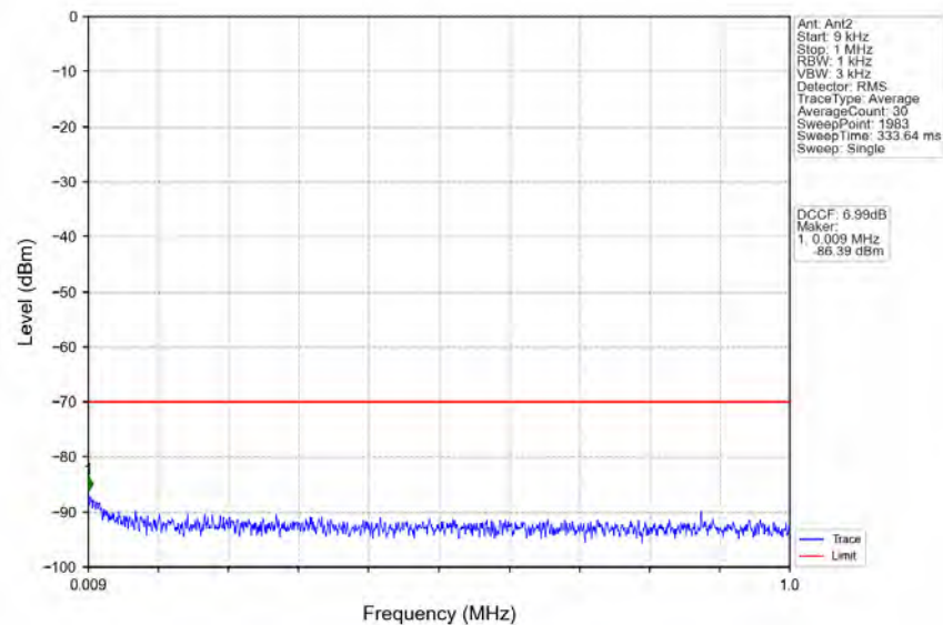
n48_30kHz_MIMO_NTNV_40MHz_CP-OFDM_QPSK_3679.98MHz_Outer_Full
