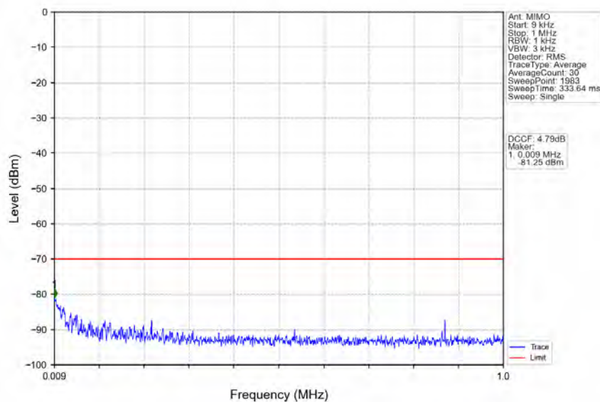
n48_30kHz_MIMO_NTNV_40MHz_CP-OFDM_QPSK_3570MHz_Edge_1RB_Left
