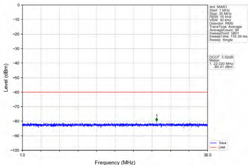
n48_30kHz_MIMO_NTNV_40MHz_CP-OFDM_QPSK_3570MHz_Inner_1RB_Left
