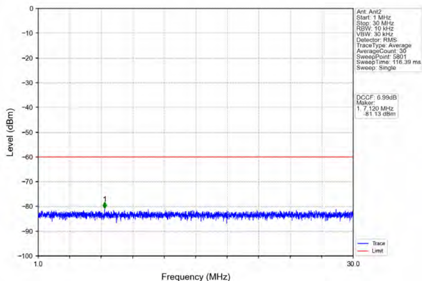
n48_30kHz_MIMO_NTNV_40MHz_CP-OFDM_QPSK_3679.98MHz_Inner_1RB_Right
