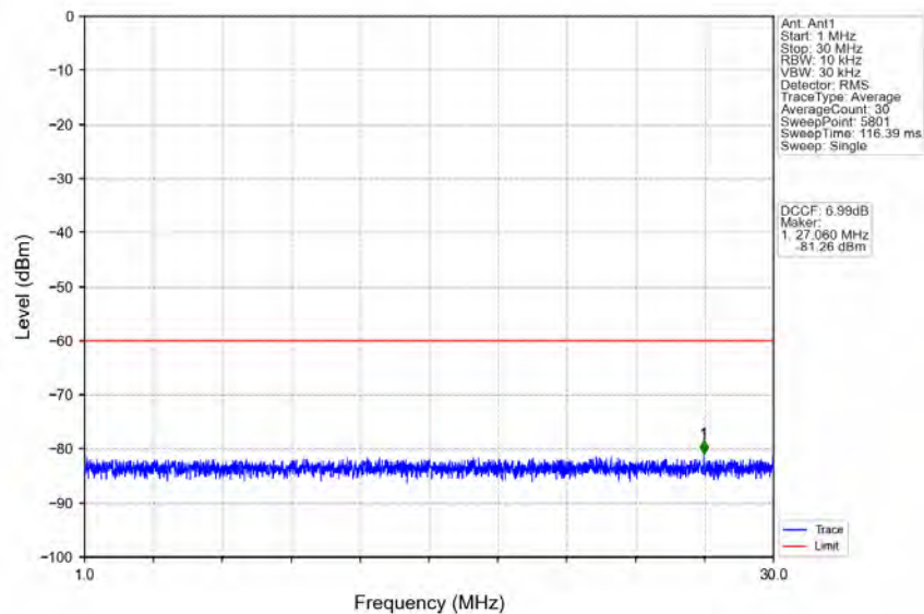
n48_30kHz_MIMO_NTNV_40MHz_CP-OFDM_QPSK_3679.98MHz_Edge_1RB_Right
