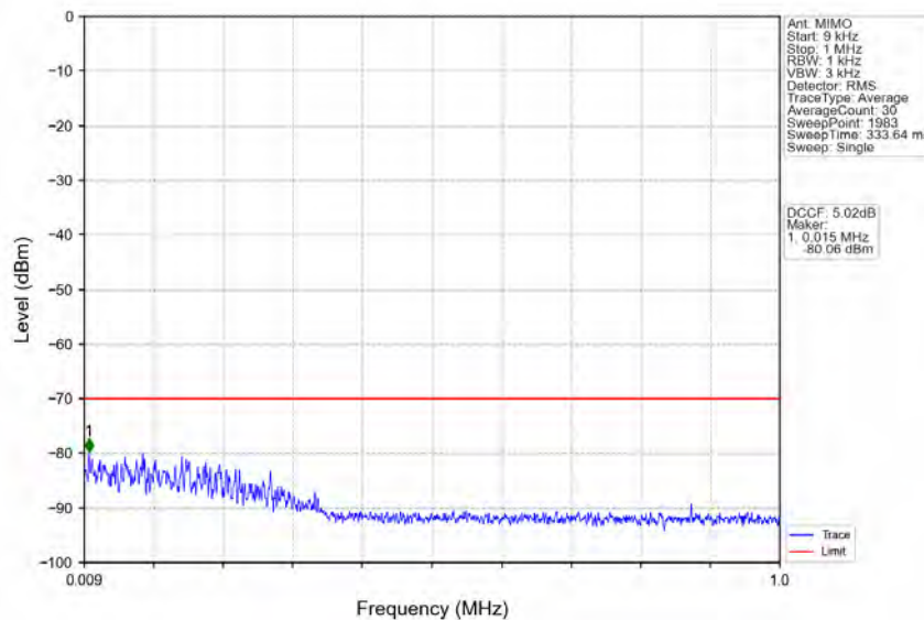
n48_30kHz_MIMO_NTNV_40MHz_CP-OFDM_QPSK_3570MHz_Inner_1RB_Left
