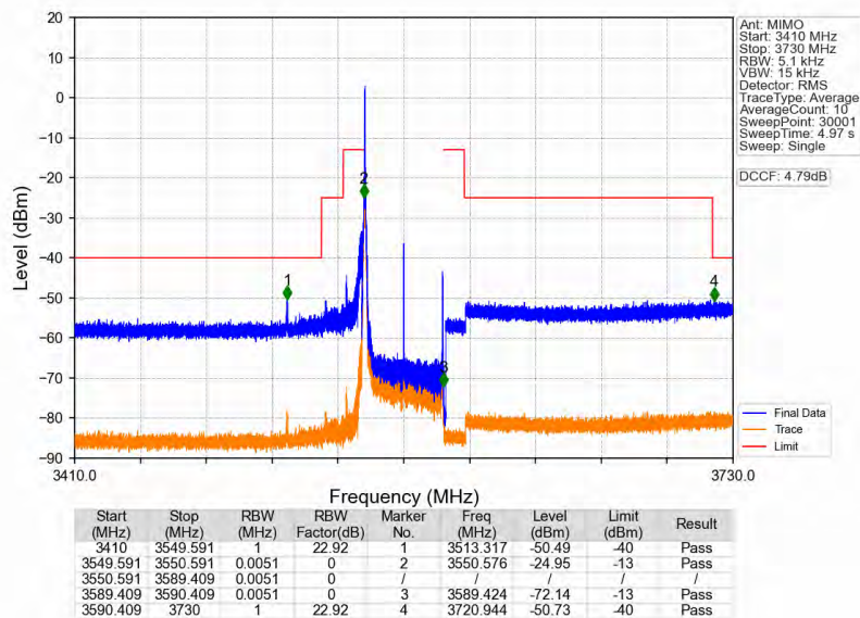
n48_30kHz_MIMO_NTNV_40MHz_CP-OFDM_QPSK_3570MHz_Edge_1RB_Left
