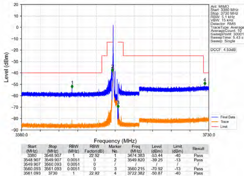
n48_30kHz_MIMO_NTNV_10MHz_CP-OFDM_QPSK_3555MHz_Inner_1RB_Left
