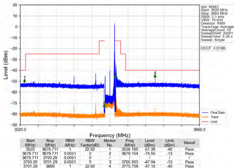
n48_30kHz_MIMO_NTNV_20MHz_CP-OFDM_QPSK_3690MHz_Edge_1RB_Right
