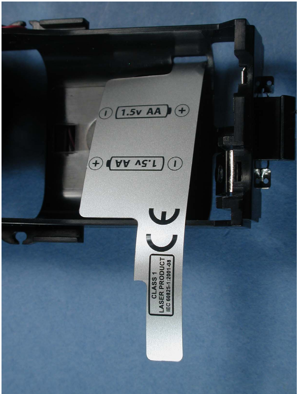
Photograph 4: Side 1 Label of M-RAZ105
