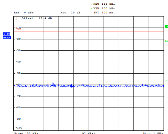
LTE Band 4 1.4MHz CH-Middle 30MHz~1GHz
