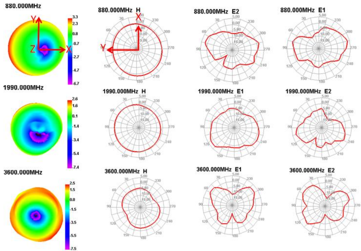
天线3D&2D方向图Antenna 3D & 2D pattern:
