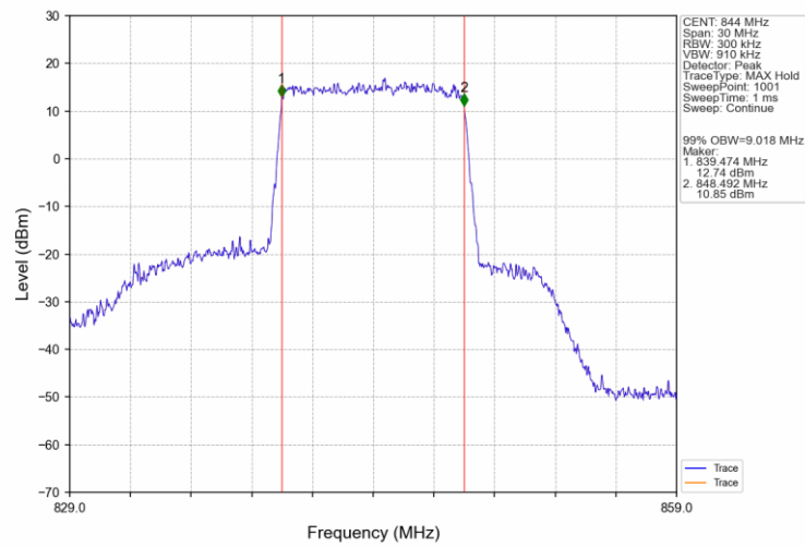
Band26b_10MHz_16QAM_HCH_844MHz_RB_50_0_NTNV
