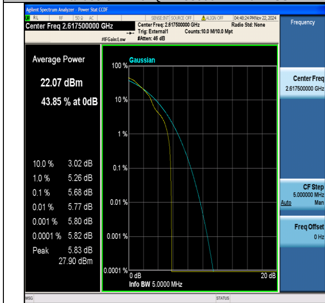
Band38-5MHz-64QAM-38225-1RB#0-PASS
