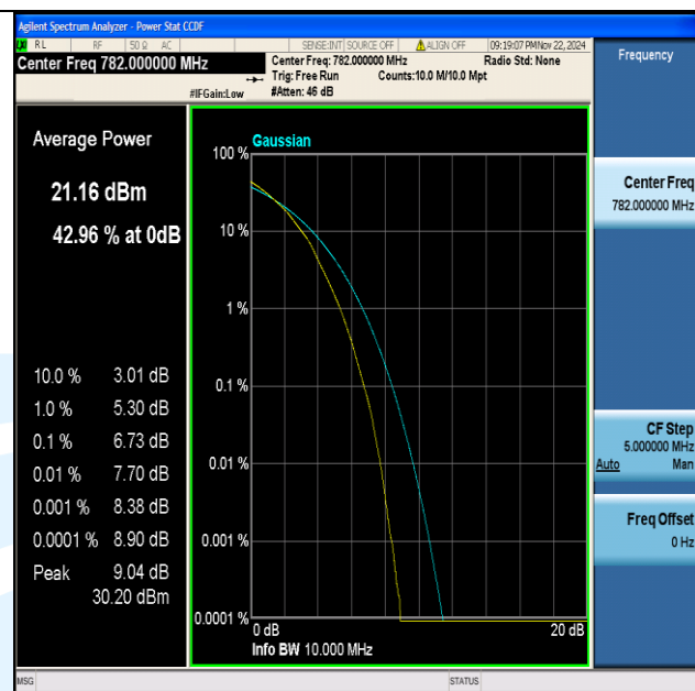
Band13-10MHz-64QAM-23230-50RB#0-PASS
