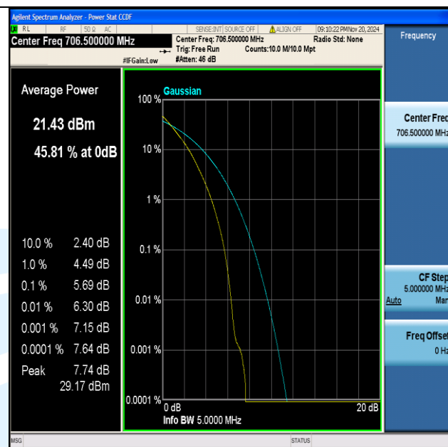
Band17-5MHz-QPSK-23755-25RB#0-PASS
