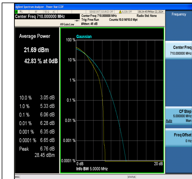
Band17-5MHz-64QAM-23790-1RB#0-PASS
