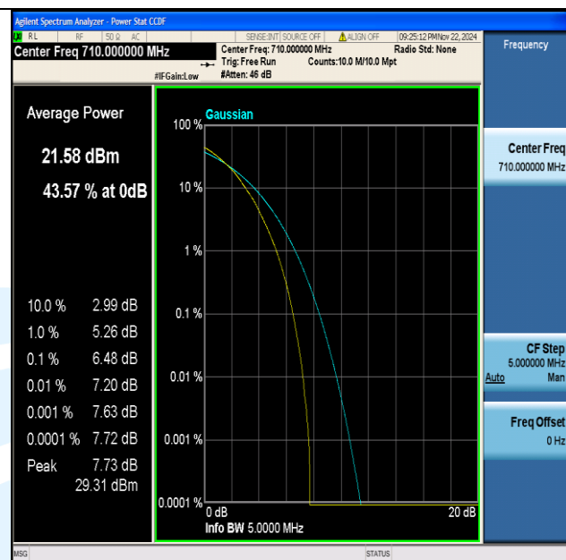
Band17-5MHz-64QAM-23790-25RB#0-PASS
