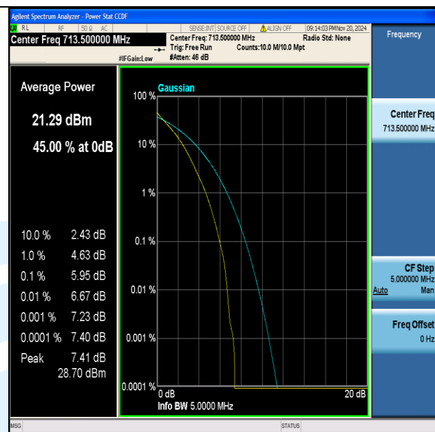
Band17-5MHz-QPSK-23825-25RB#0-PASS
