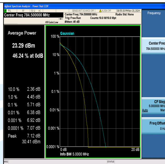
Band13-5MHz-QPSK-23255-25RB#0-PASS
