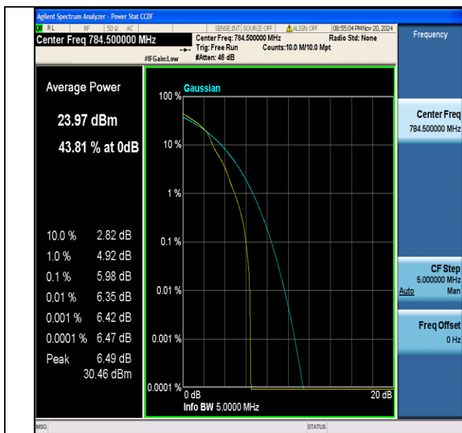
Band13-5MHz-16QAM-23255-1RB#0-PASS
