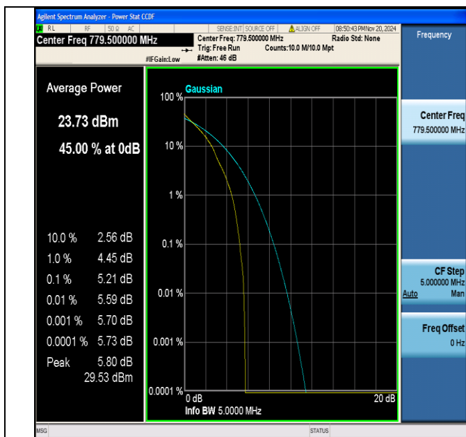
Band13-5MHz-QPSK-23205-1RB#0-PASS
