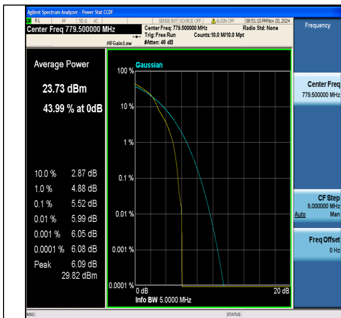
Band13-5MHz-16QAM-23205-1RB#0-PASS
