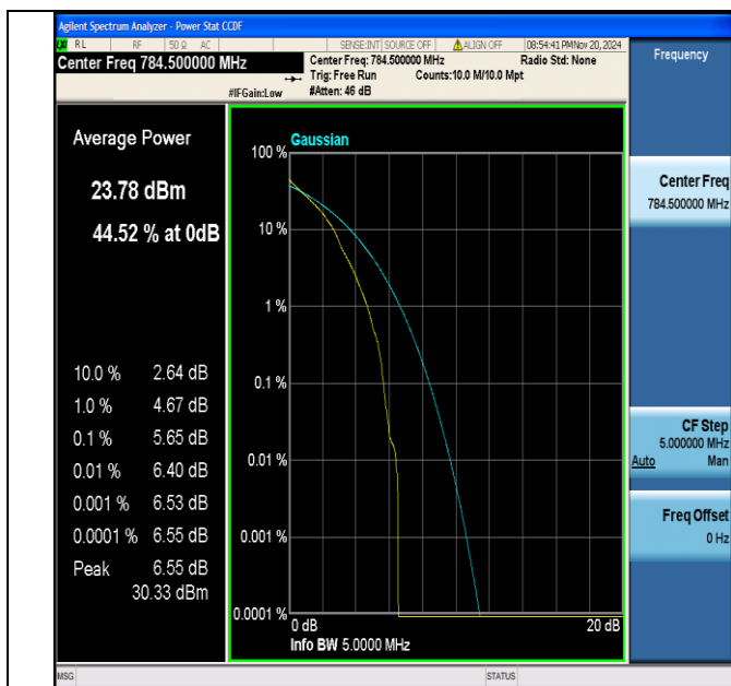
Band13-5MHz-QPSK-23255-1RB#0-PASS
