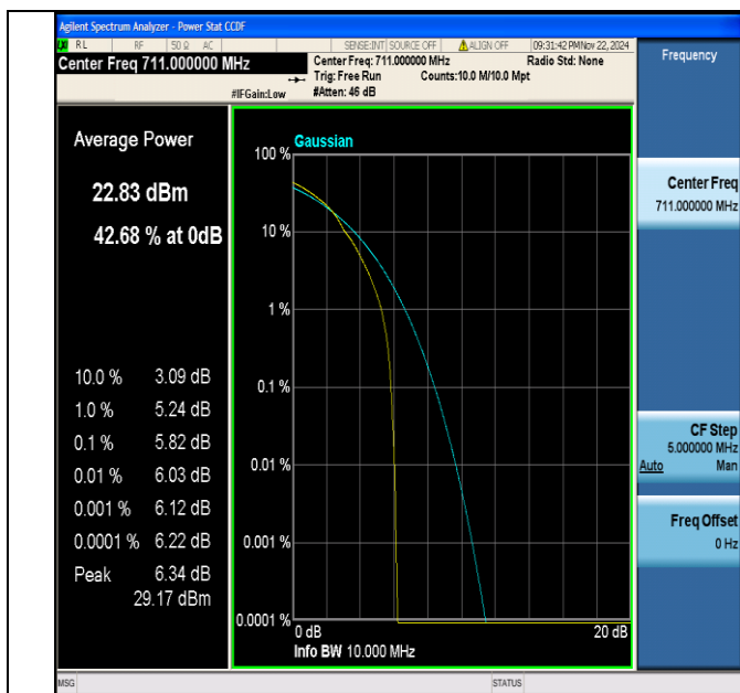
Band17-10MHz-64QAM-23800-1RB#0-PASS
