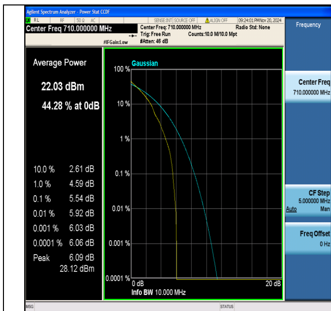
Band17-10MHz-QPSK-23790-1RB#0-PASS
