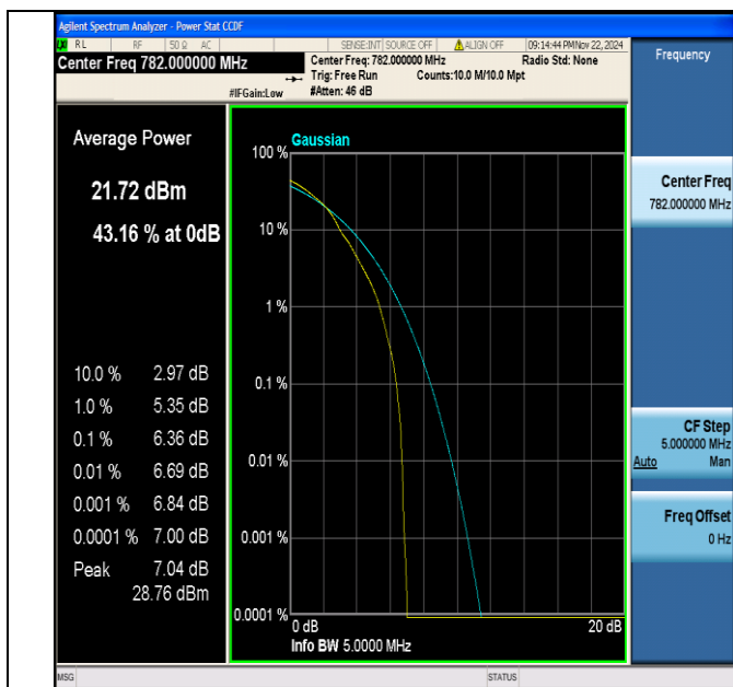
Band13-5MHz-64QAM-23230-1RB#0-PASS
