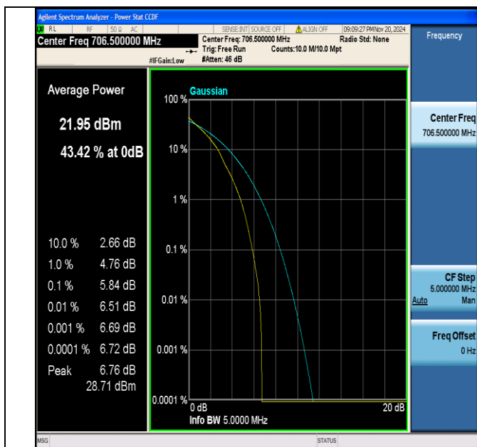
Band17-5MHz-QPSK-23755-1RB#0-PASS
