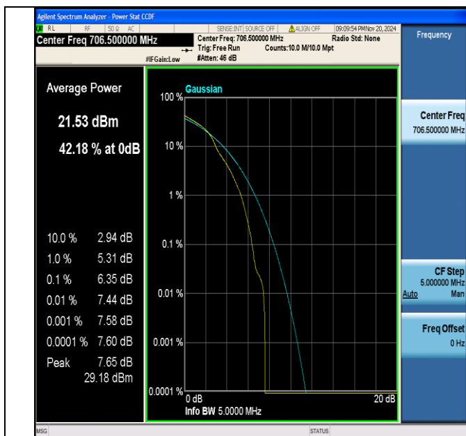
Band17-5MHz-16QAM-23755-1RB#0-PASS
