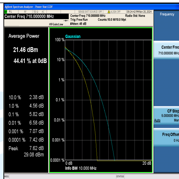
Band17-10MHz-QPSK-23790-50RB#0-PASS
