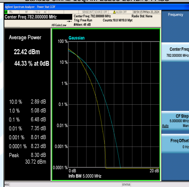
Band13-5MHz-16QAM-23230-25RB#0-PASS
