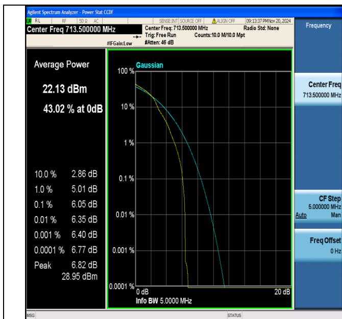
Band17-5MHz-16QAM-23825-1RB#0-PASS
