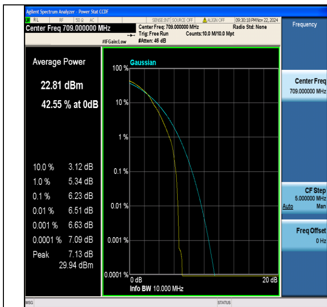
Band17-10MHz-64QAM-23780-1RB#0-PASS
