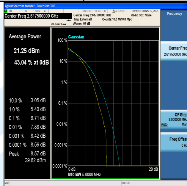
Band38-5MHz-64QAM-38225-25RB#0-PASS
