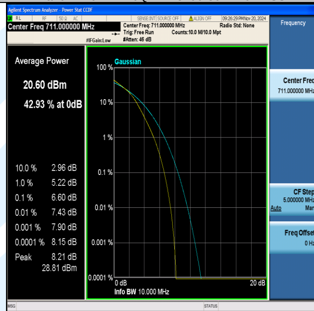
Band17-10MHz-16QAM-23800-50RB#0-PASS
