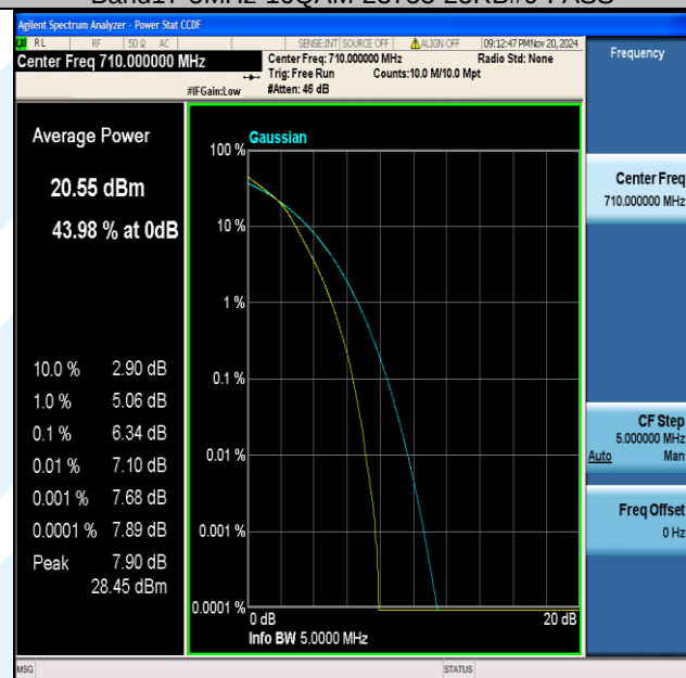
Band17-5MHz-16QAM-23790-25RB#0-PASS
