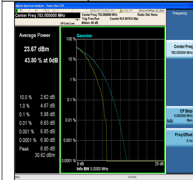
Band13-5MHz-QPSK-23230-1RB#0-PASS
