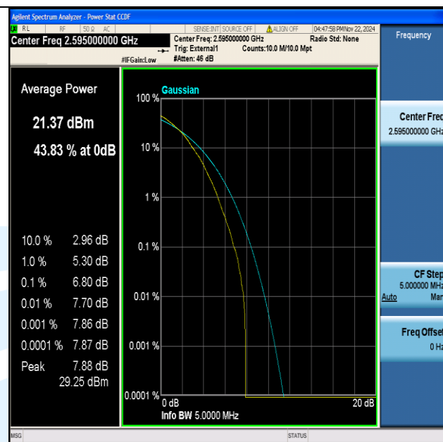
Band38-5MHz-64QAM-38000-25RB#0-PASS
