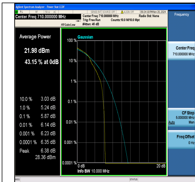
Band17-10MHz-16QAM-23790-1RB#0-PASS
