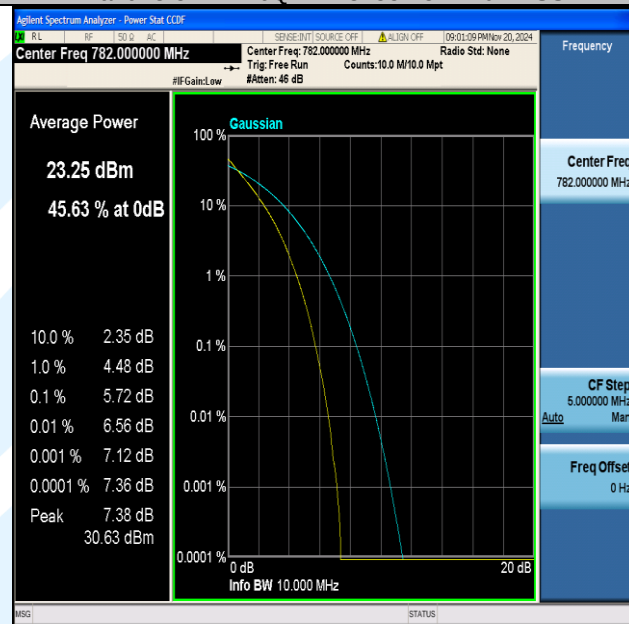
Band13-10MHz-QPSK-23230-50RB#0-PASS
