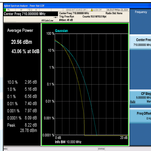
Band17-10MHz-16QAM-23790-50RB#0-PASS
