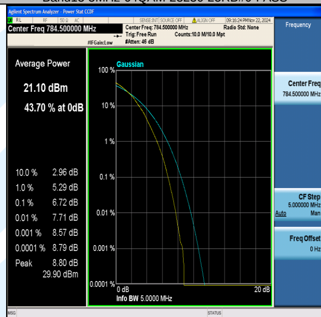
Band13-5MHz-64QAM-23255-25RB#0-PASS
