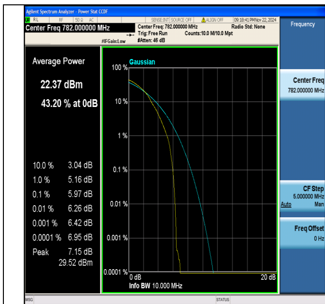
Band13-10MHz-64QAM-23230-1RB#0-PASS
