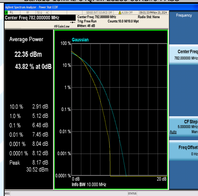
Band13-10MHz-16QAM-23230-50RB#0-PASS
