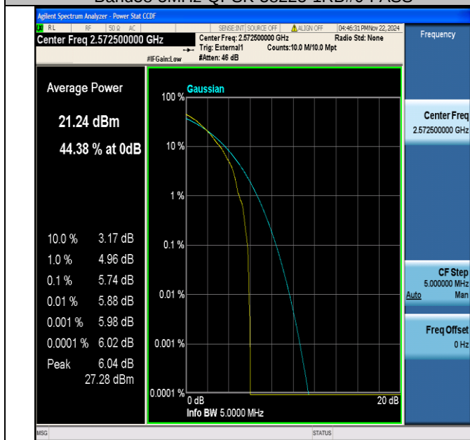
Band38-5MHz-64QAM-37775-1RB#0-PASS
