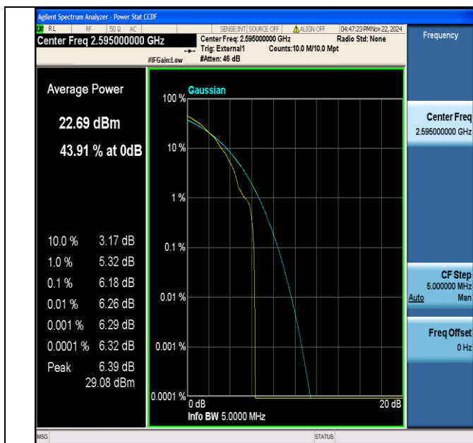
Band38-5MHz-64QAM-38000-1RB#0-PASS
