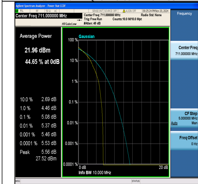
Band17-10MHz-QPSK-23800-1RB#0-PASS
