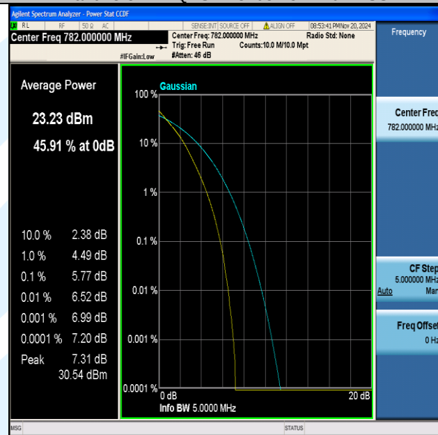
Band13-5MHz-QPSK-23230-25RB#0-PASS
