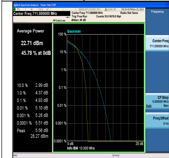
Band17-10MHz-16QAM-23800-1RB#0-PASS
