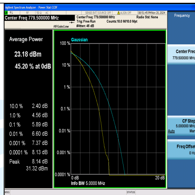
Band13-5MHz-QPSK-23205-25RB#0-PASS
