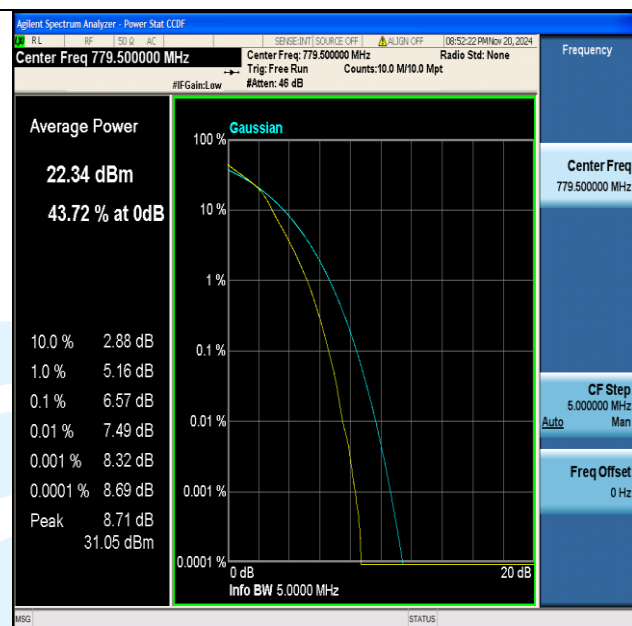
Band13-5MHz-16QAM-23205-25RB#0-PASS
