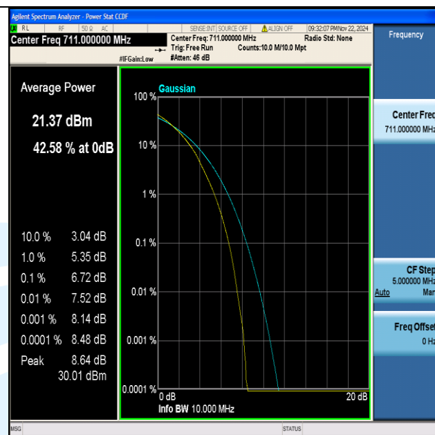
Band17-10MHz-64QAM-23800-50RB#0-PASS
