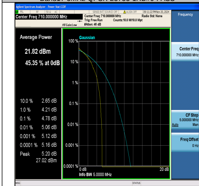
Band17-5MHz-QPSK-23790-1RB#0-PASS
