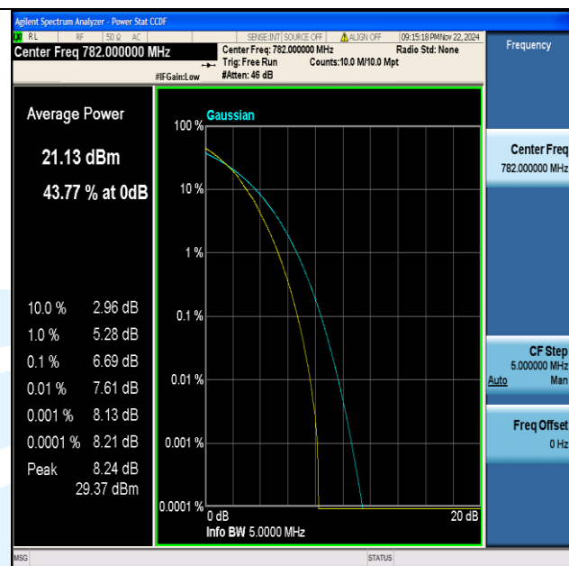
Band13-5MHz-64QAM-23230-25RB#0-PASS
