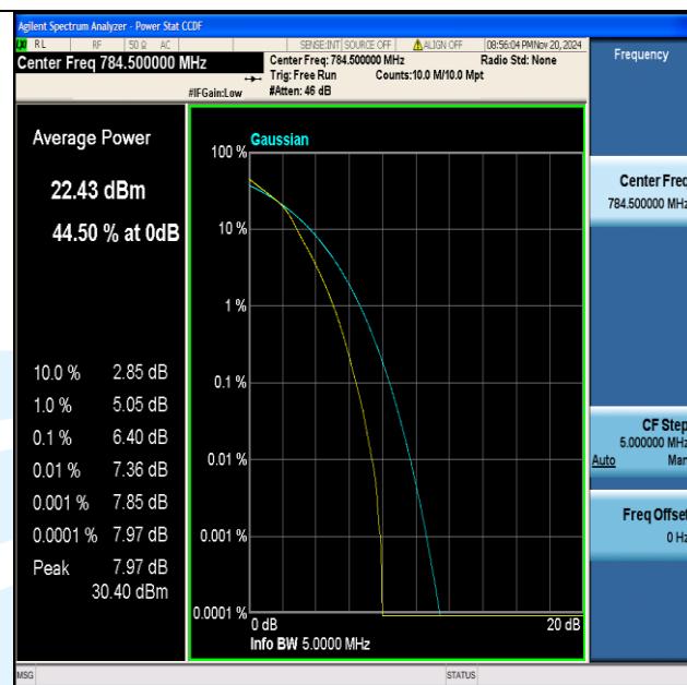
Band13-5MHz-16QAM-23255-25RB#0-PASS
