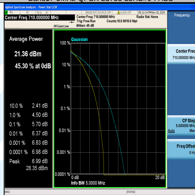
Band17-5MHz-QPSK-23790-25RB#0-PASS
