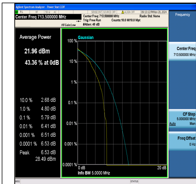
Band17-5MHz-QPSK-23825-1RB#0-PASS
