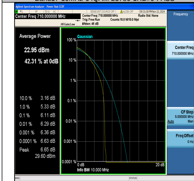
Band17-10MHz-64QAM-23790-1RB#0-PASS
