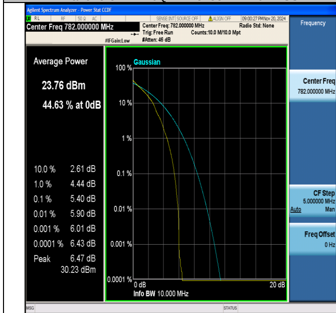
Band13-10MHz-QPSK-23230-1RB#0-PASS
