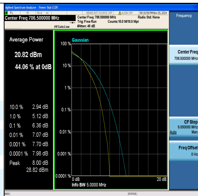
Band17-5MHz-16QAM-23755-25RB#0-PASS
