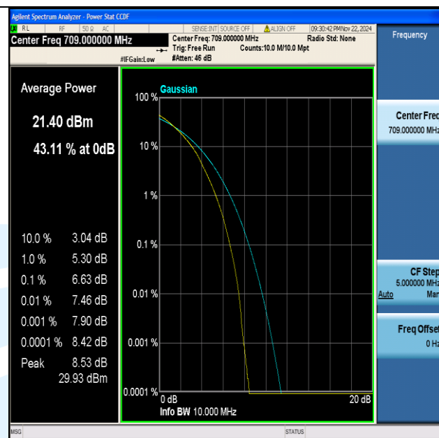
Band17-10MHz-64QAM-23780-50RB#0-PASS
