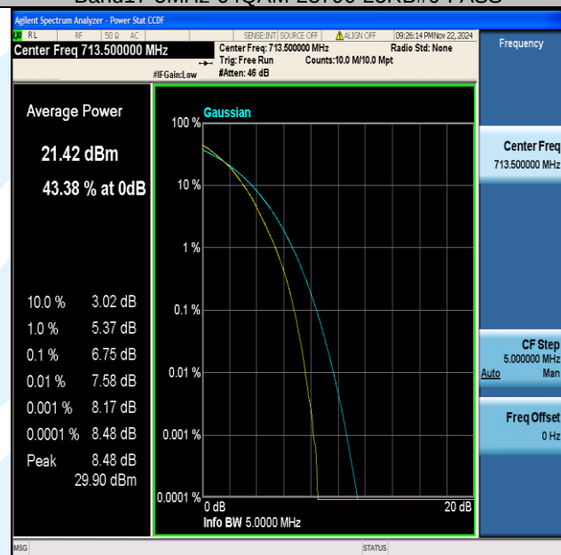
Band17-5MHz-64QAM-23825-25RB#0-PASS
