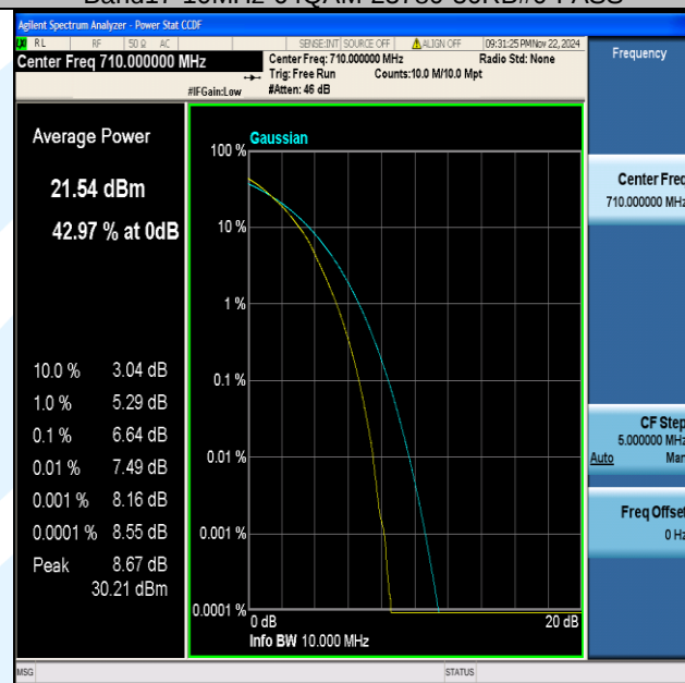
Band17-10MHz-64QAM-23790-50RB#0-PASS
