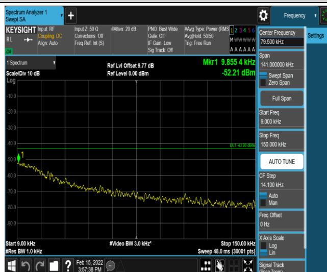
Band25-5MHz-QPSK-26065-1-0-Low-0.009-0.15--52.21-PASS
