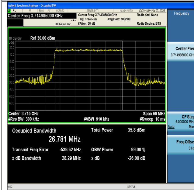
NTNV-n77(3700-3980)-PC2-30-30-L-DFT-BPSK- Outer_Full-Ant1-PASS
