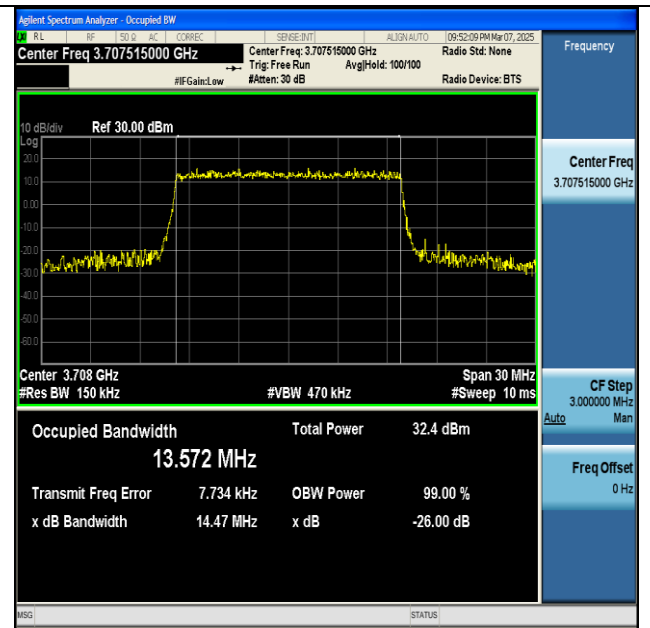
NTNV-n77(3700-3980)-PC2-30-15-L-CP-16QAM- Outer_Full-Ant1-PASS
