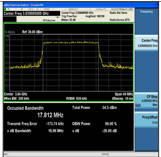
NTNV-n77(3700-3980)-PC2-30-20-M-DFT-16QAM- Outer_Full-Ant1-PASS
