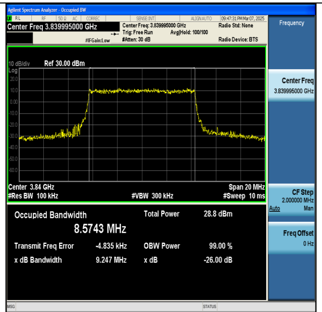
NTNV-n77(3700-3980)-PC2-30-10-M-CP-256QAM- Outer_Full-Ant1-PASS
