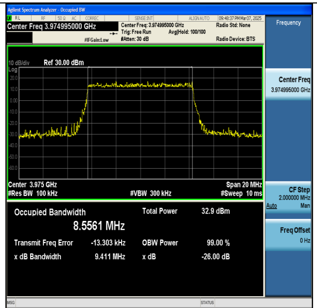
NTNV-n77(3700-3980)-PC2-30-10-H-DFT-64QAM-Outer_Full-Ant1-PASS
