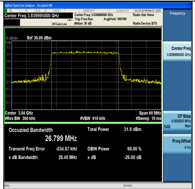
NTNV-n77(3700-3980)-PC2-30-30-M-DFT-256QAM- Outer_Full-Ant1-PASS
