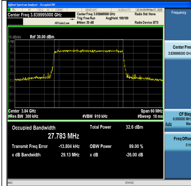
NTNV-n77(3700-3980)-PC2-30-30-M-CP-64QAM-Outer_Full-Ant1-PASS
