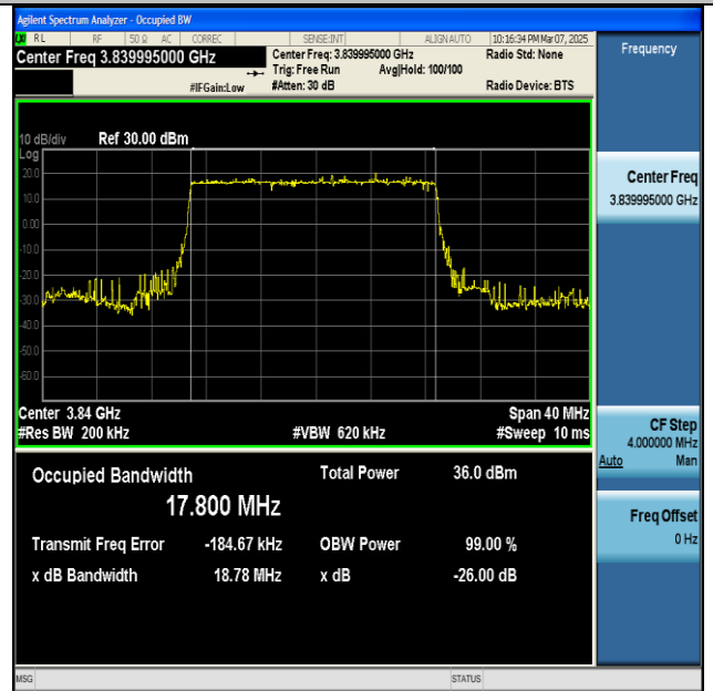
NTNV-n77(3700-3980)-PC2-30-20-M-DFT-BPSK- Outer_Full-Ant1-PASS
