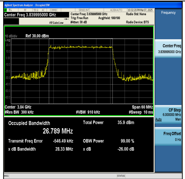
NTNV-n77(3700-3980)-PC2-30-30-M-DFT-BPSK- Outer_Full-Ant1-PASS
