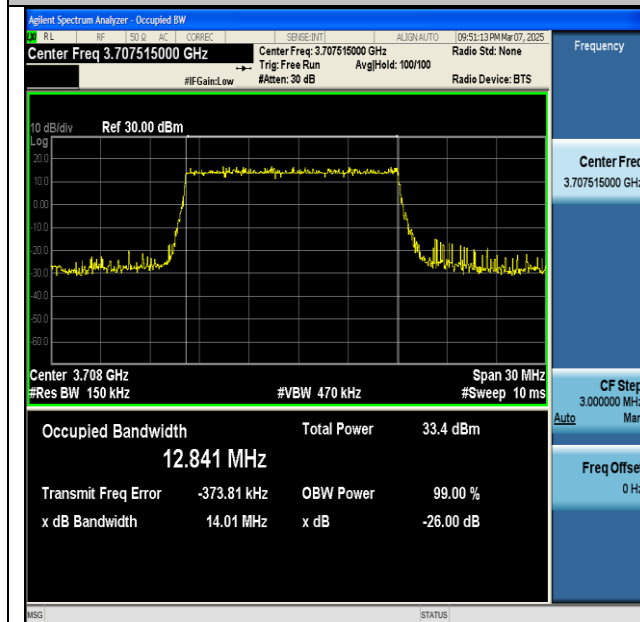
NTNV-n77(3700-3980)-PC2-30-15-L-DFT-64QAM-Outer_Full-Ant1-PASS
