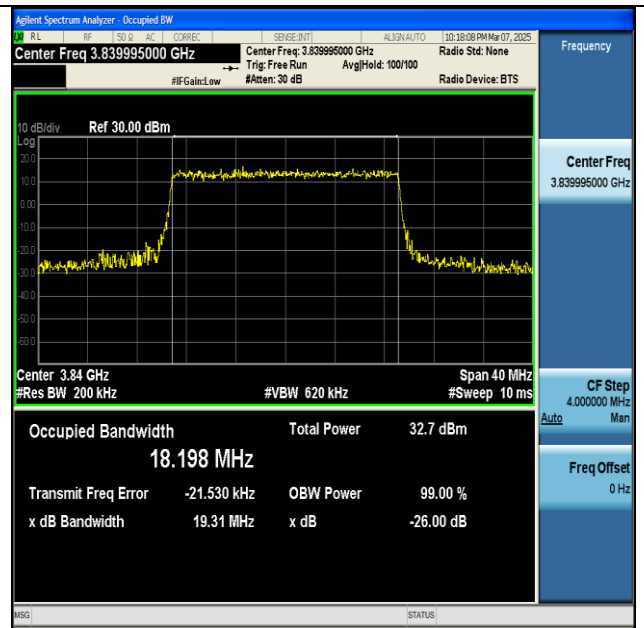
NTNV-n77(3700-3980)-PC2-30-20-M-CP-16QAM- Outer_Full-Ant1-PASS
