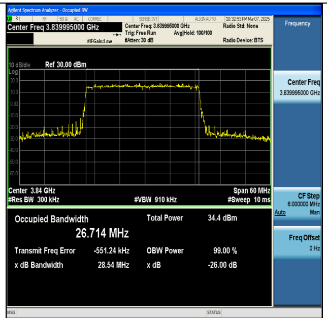
NTNV-n77(3700-3980)-PC2-30-30-M-DFT-16QAM- Outer_Full-Ant1-PASS
