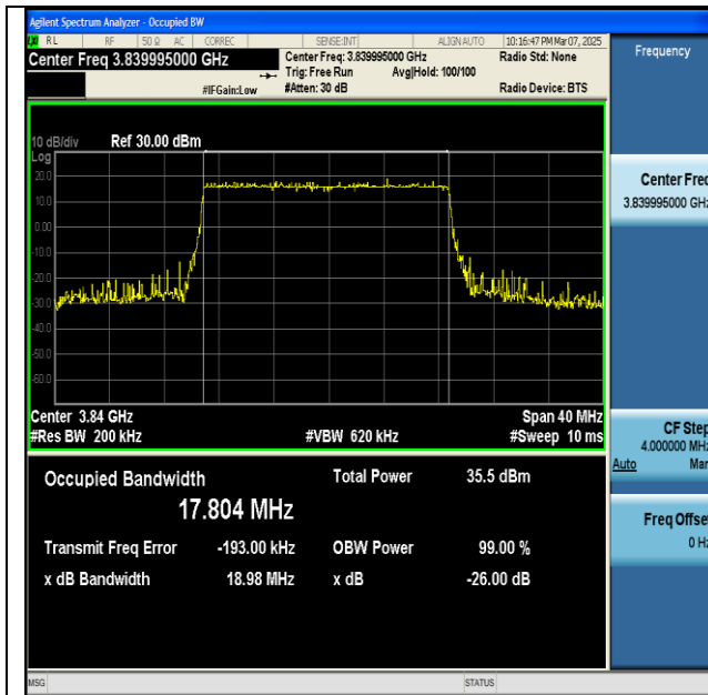
NTNV-n77(3700-3980)-PC2-30-20-M-DFT-QPSK- Outer_Full-Ant1-PASS
