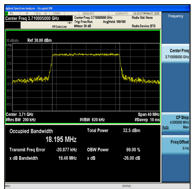
NTNV-n77(3700-3980)-PC2-30-20-L-CP-QPSK- Outer_Full-Ant1-PASS
