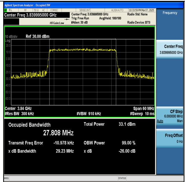
NTNV-n77(3700-3980)-PC2-30-30-M-CP-16QAM-Outer_Full-Ant1-PASS
