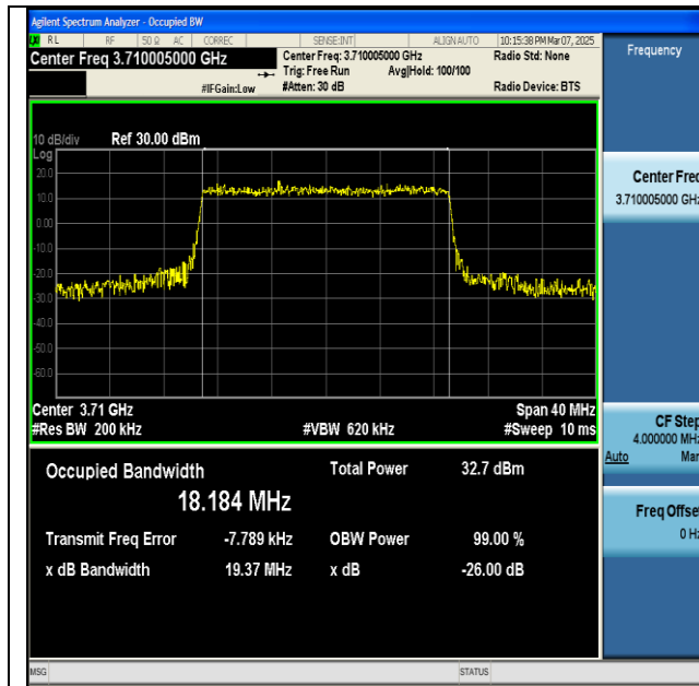
NTNV-n77(3700-3980)-PC2-30-20-L-CP-16QAM- Outer_Full-Ant1-PASS
