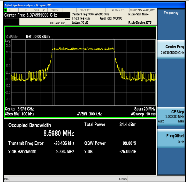
NTNV-n77(3700-3980)-PC2-30-10-H-DFT-QPSK- Outer_Full-Ant1-PASS
