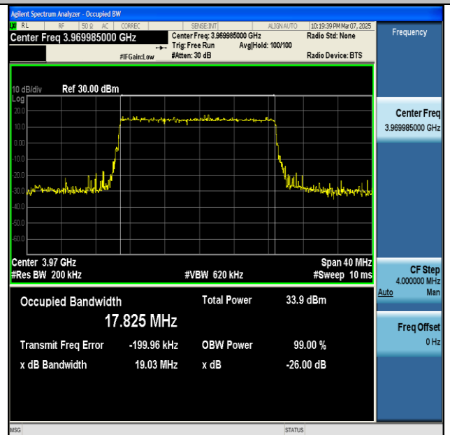
NTNV-n77(3700-3980)-PC2-30-20-H-DFT-64QAM- Outer_Full-Ant1-PASS
