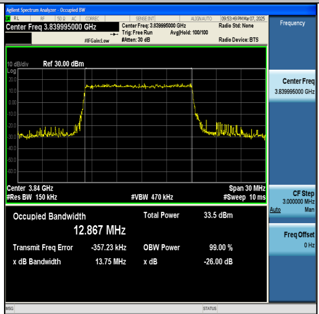
NTNV-n77(3700-3980)-PC2-30-15-M-DFT-64QAM-Outer_Full-Ant1-PASS
