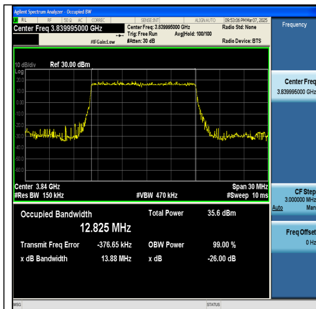
NTNV-n77(3700-3980)-PC2-30-15-M-DFT-BPSK-Outer_Full-Ant1-PASS
