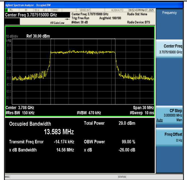
NTNV-n77(3700-3980)-PC2-30-15-L-CP-256QAM- Outer_Full-Ant1-PASS
