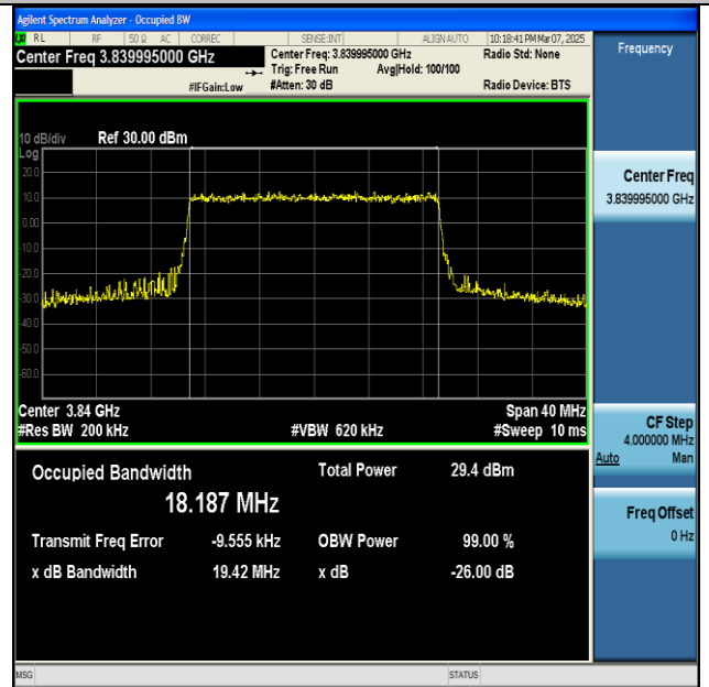
NTNV-n77(3700-3980)-PC2-30-20-M-CP-256QAM- Outer_Full-Ant1-PASS
