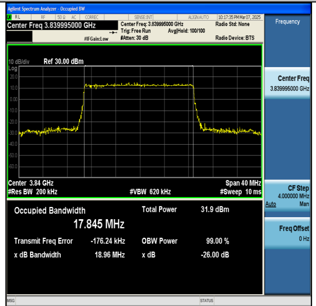
NTNV-n77(3700-3980)-PC2-30-20-M-DFT-256QAM- Outer_Full-Ant1-PASS
