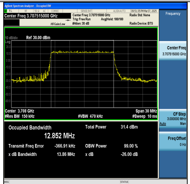
NTNV-n77(3700-3980)-PC2-30-15-L-DFT-256QAM-Outer_Full-Ant1-PASS
