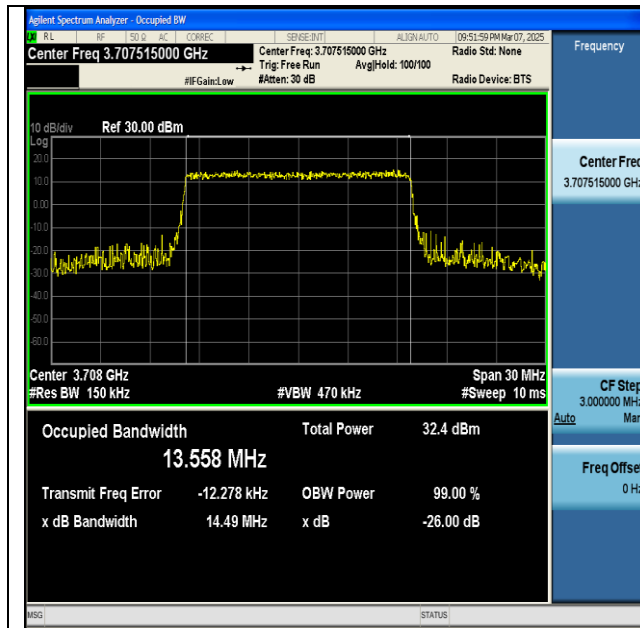
NTNV-n77(3700-3980)-PC2-30-15-L-CP-QPSK- Outer_Full-Ant1-PASS
