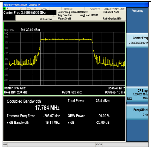
NTNV-n77(3700-3980)-PC2-30-20-H-DFT-QPSK- Outer_Full-Ant1-PASS
