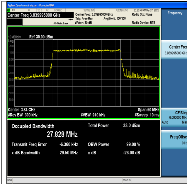
NTNV-n77(3700-3980)-PC2-30-30-M-CP-QPSK-Outer_Full-Ant1-PASS
