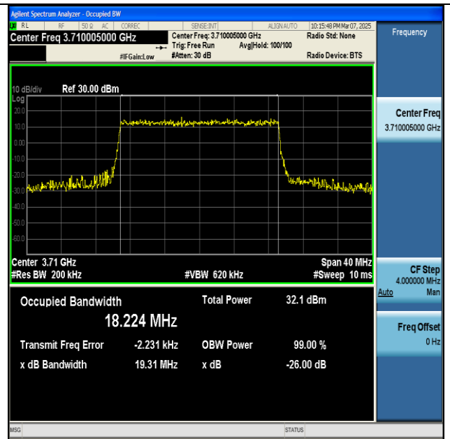
NTNV-n77(3700-3980)-PC2-30-20-L-CP-64QAM- Outer_Full-Ant1-PASS
