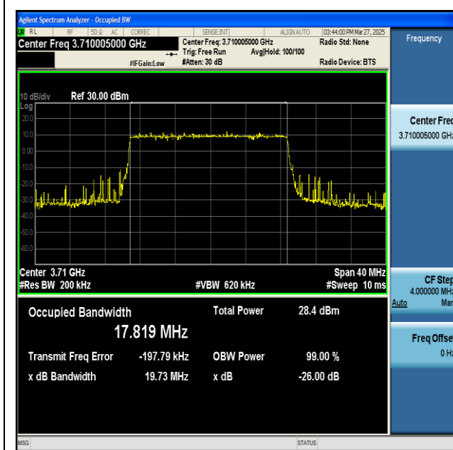
NTNV-n77(3700-3980)-PC2-30-20-L-DFT-256QAM- Outer_Full-Ant1-PASS
