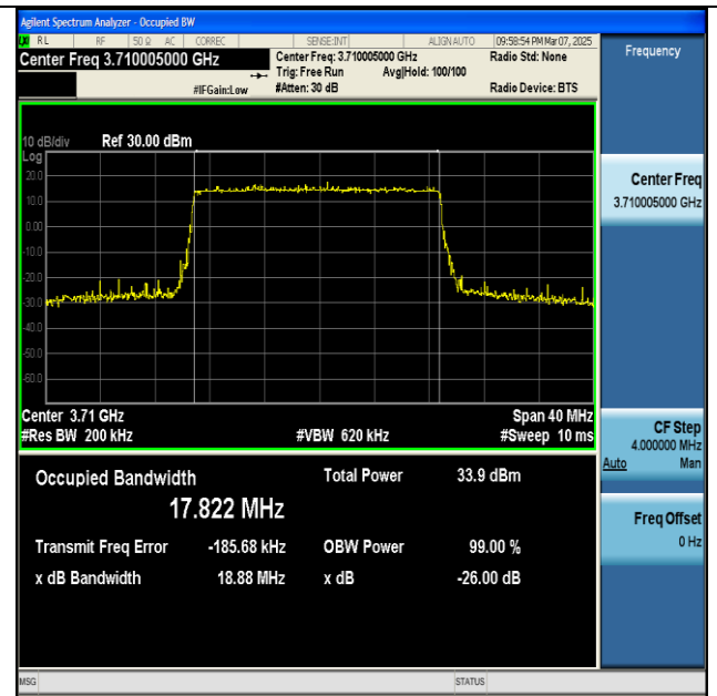
NTNV-n77(3700-3980)-PC2-30-20-L-DFT-64QAM- Outer_Full-Ant1-PASS
