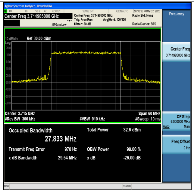
NTNV-n77(3700-3980)-PC2-30-30-L-CP-64QAM- Outer_Full-Ant1-PASS
