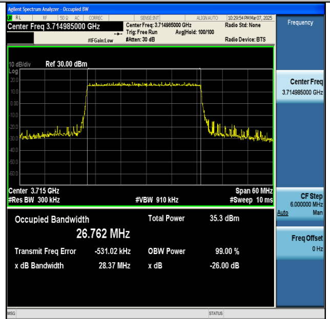
NTNV-n77(3700-3980)-PC2-30-30-L-DFT-QPSK- Outer_Full-Ant1-PASS
