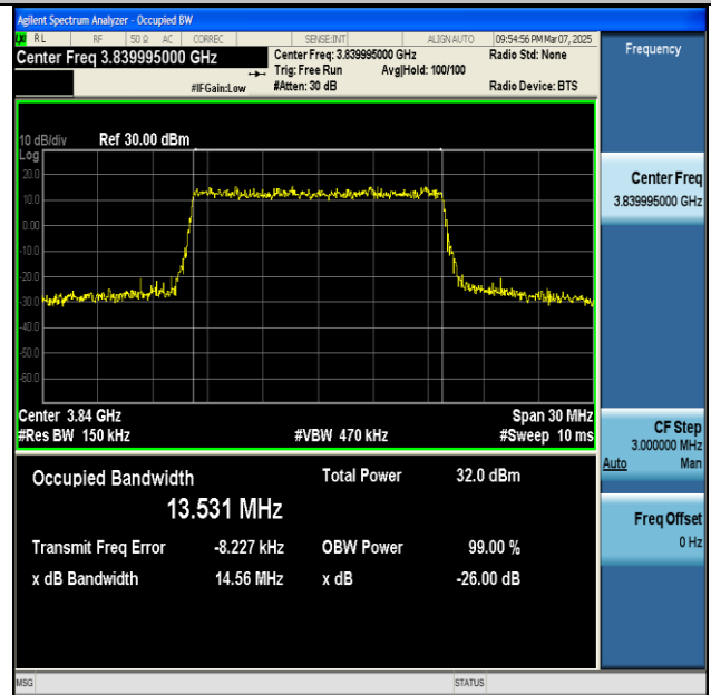
NTNV-n77(3700-3980)-PC2-30-15-M-CP-64QAM- Outer_Full-Ant1-PASS
