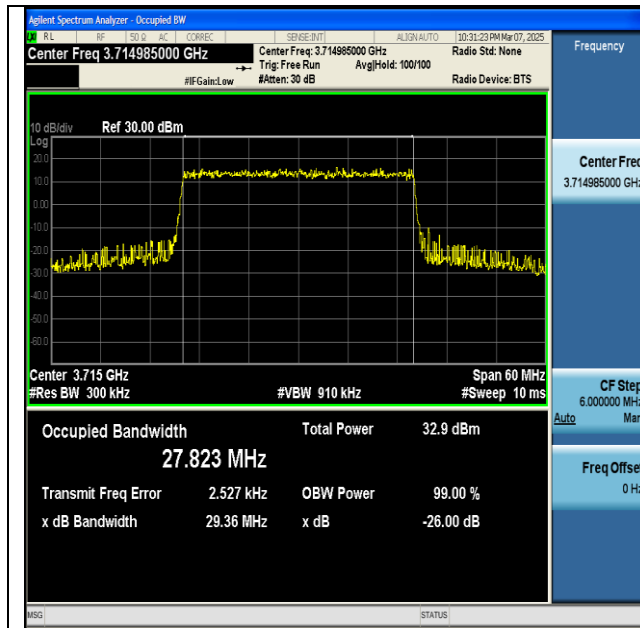
NTNV-n77(3700-3980)-PC2-30-30-L-CP-16QAM- Outer_Full-Ant1-PASS
