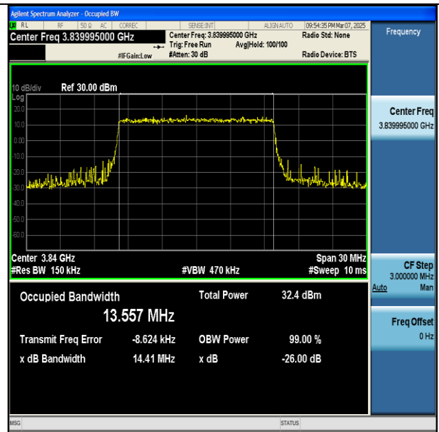
NTNV-n77(3700-3980)-PC2-30-15-M-CP-QPSK- Outer_Full-Ant1-PASS
