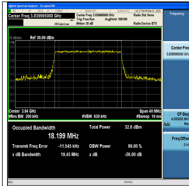
NTNV-n77(3700-3980)-PC2-30-20-M-CP-QPSK- Outer_Full-Ant1-PASS
