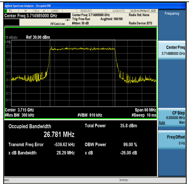
NTNV-n77(3700-3980)-PC2-30-30-L-DFT-BPSK- Outer_Full-Ant1-PASS
