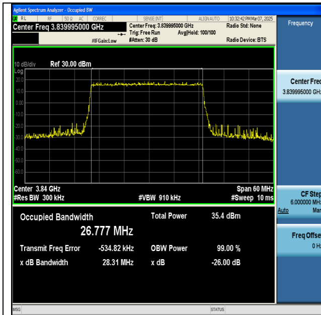
NTNV-n77(3700-3980)-PC2-30-30-M-DFT-QPSK- Outer_Full-Ant1-PASS
