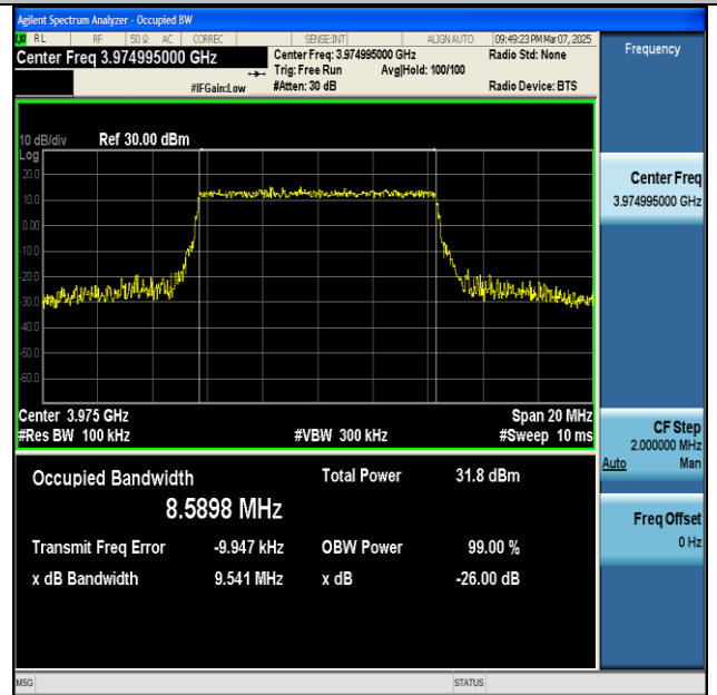
NTNV-n77(3700-3980)-PC2-30-10-H-CP-QPSK-Outer_Full-Ant1-PASS
