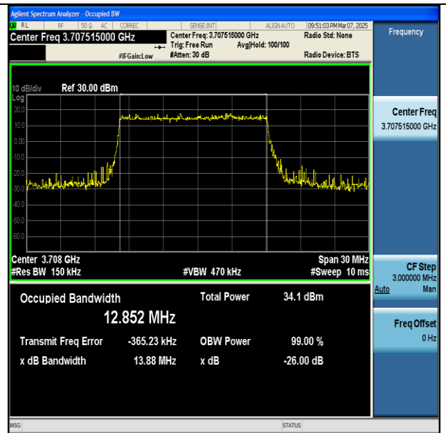
NTNV-n77(3700-3980)-PC2-30-15-L-DFT-16QAM-Outer_Full-Ant1-PASS
