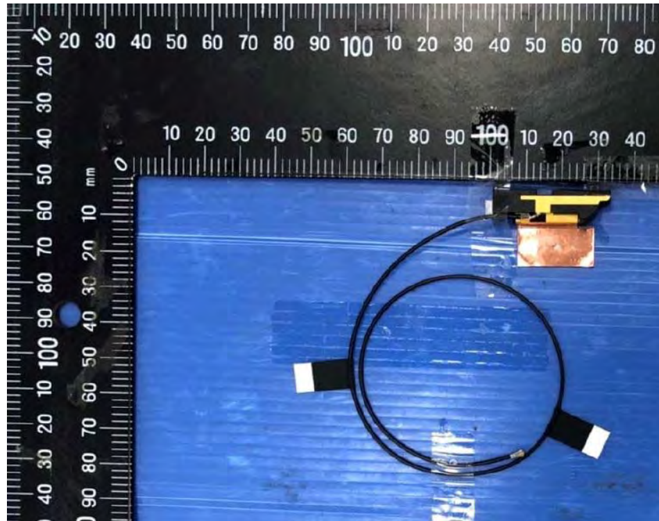
INPAQ Main Antenna Part No.: MDA-LB-02-022 ASUS No.: 14008-04050300
