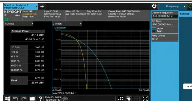
Band5-4233-4-PASS
