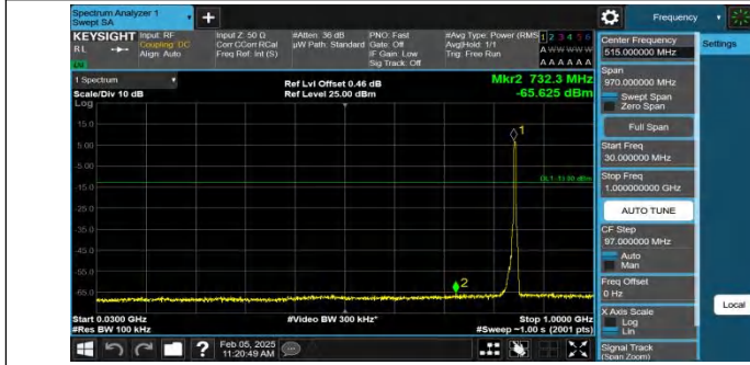
Band5-4233-30~1000MHz-PASS
