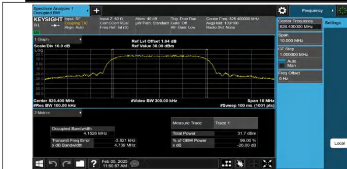
Band5-4132-1-PASS
