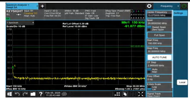
Band5-4233-0.15~30MHz-PASS
