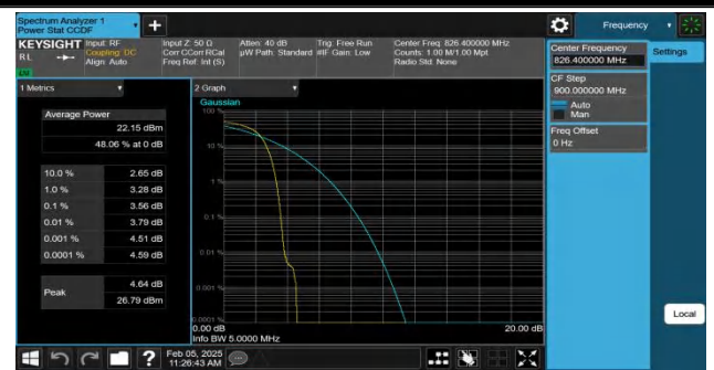
Band5-4132-2-PASS
