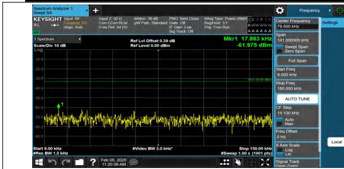
Band5-4233-0.009~0.15MHz-PASS
