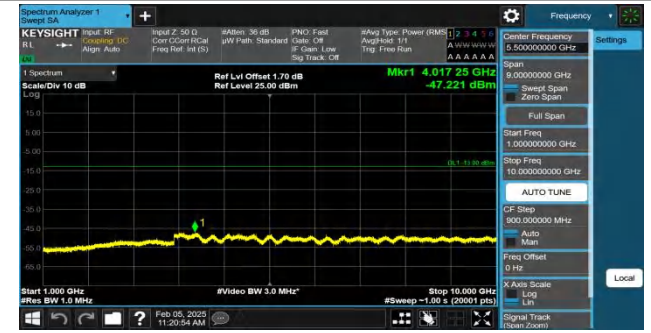
Band5-4233-1000~10000MHz-PASS
