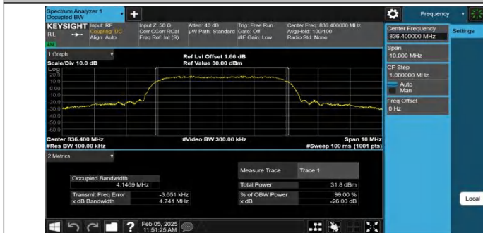
Band5-4182-1-PASS
