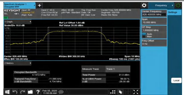
Band5-4132-4-PASS
