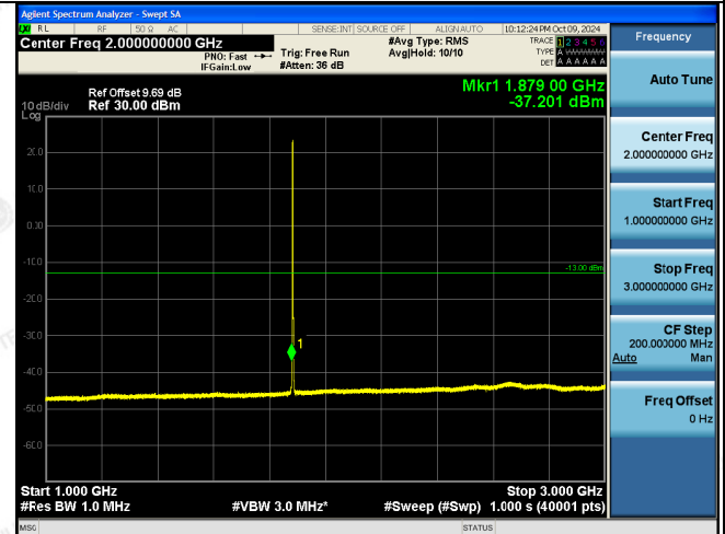
1GHz~3GHz
