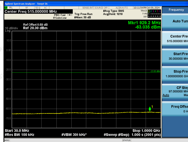
30MHz~1GHz
