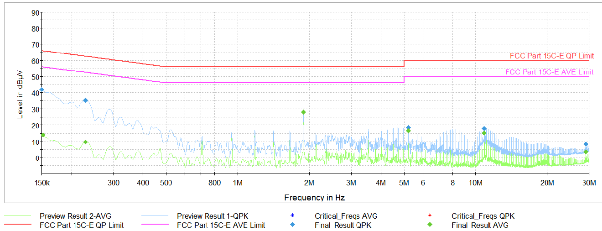
Plot 7-40. AC Line Conducted Plot with Bluetooth LE (N, 1Mbps ePA – Ch.19, with AC Power Cable)
