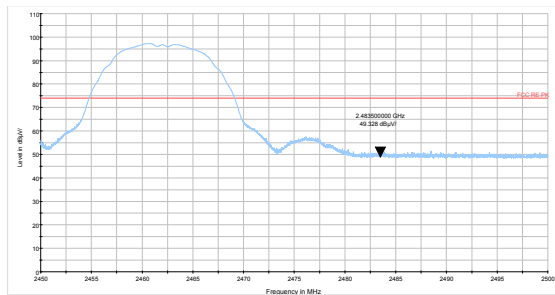
802.11b-Channel 11 Peak
