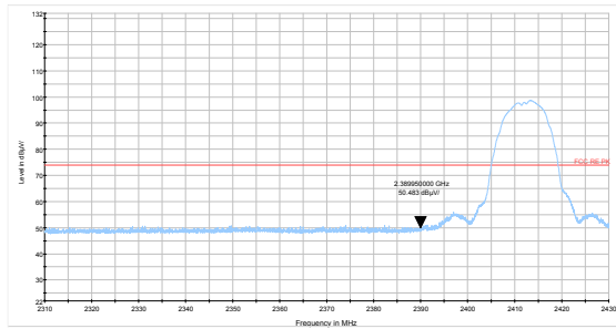
802.11b-Channel 1 Peak
