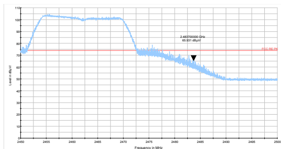
802.11g-Channel 11 Peak
