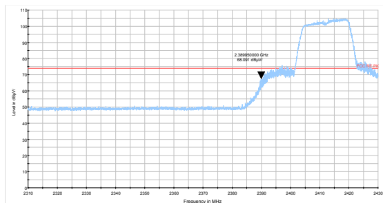
802.11g-Channel 1 Peak
