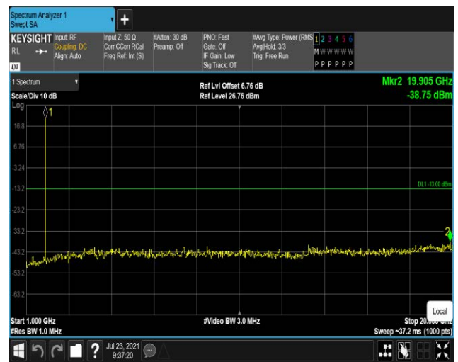
Band2-1.4MHz-16QAM-18900:1000~20000MHz
