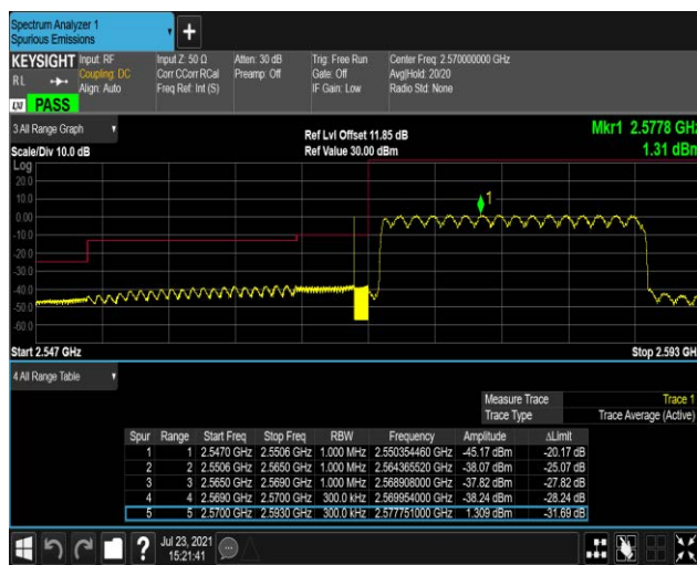
Band38-20MHz-16QAM-38150-1RB#99
