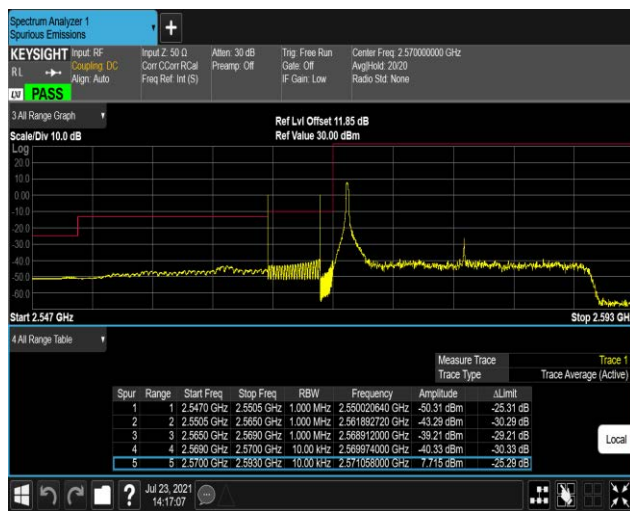
Band38-20MHz-QPSK-37850-100RB#0
