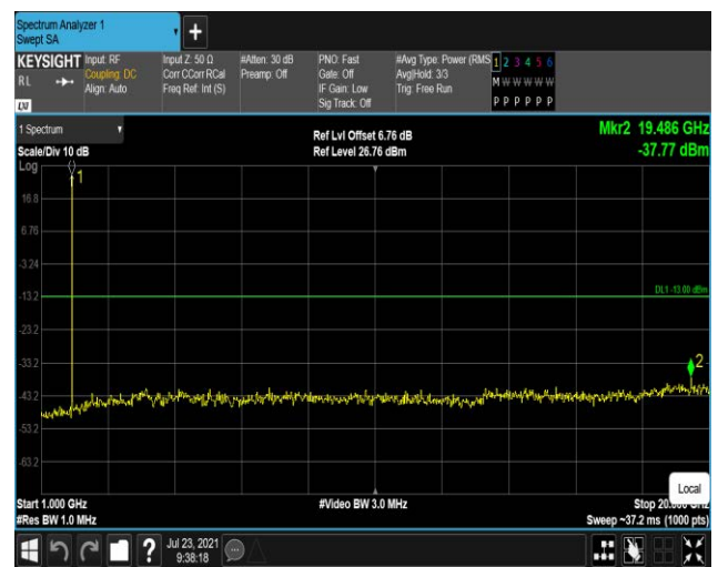
Band2-1.4MHz-16QAM-19193:1000~20000MHz
