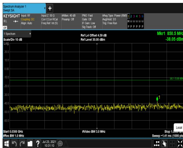
Band2-20MHz-QPSK-19100:30~1000MHz
