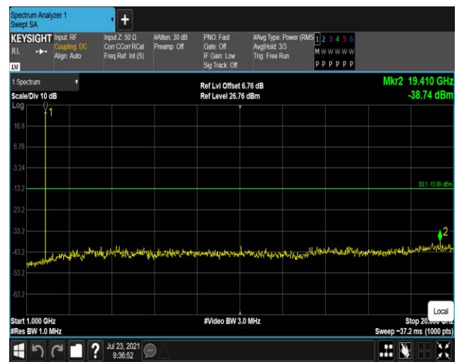
Band2-1.4MHz-QPSK-18900:1000~20000MHz
