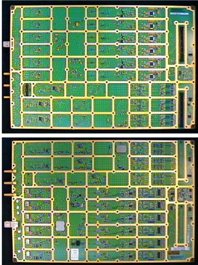
TRM Radio Board
