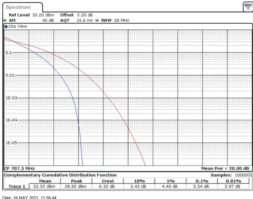
Band12-10MHz-QPSK-23095-50RB#0
