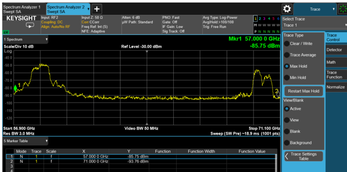
Frequency Stability -40 degrees 1 GHz Bandwidth
