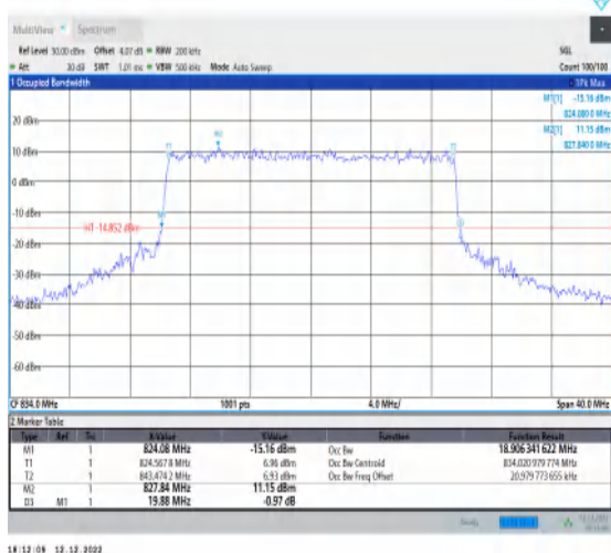
1-N5-15-20-L-6-CP-QPSK-Outer_Full-106@0-Ant1- 18.906-19.880-≤20-PASS
