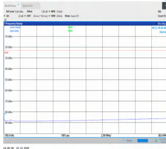
1-N5-15-20-L-1-DFT-PI2BPSK-Inner_1RB_Left-1@1 -0.15-30-Ant1-0.15--85.26--23-PASS
