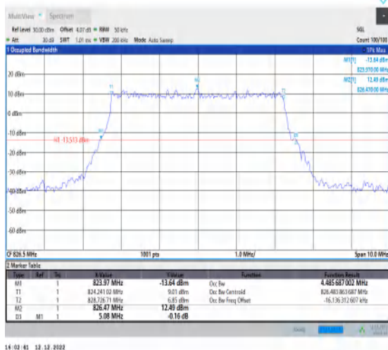
1-N5-15-5-L-3-DFT-16QAM-Outer_Full-25@0-Ant1- 4.486-5.080-≤5-PASS
