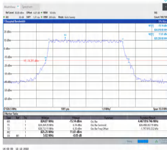
1-N5-15-5-L-4-DFT-64QAM-Outer_Full-25@0-Ant1-4 .468-5.020-≤5-PASS
