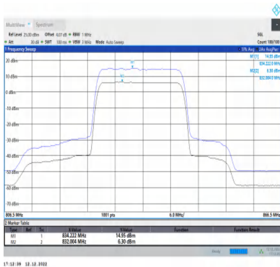
1-N5-15-20-M-1-DFT-256QAM-Outer_Full-100@0-A nt1-8.65-100%-0.00-8.65-PASS-≤13
