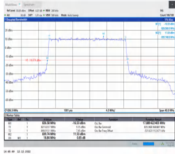
1-N5-15-20-M-4-DFT-64QAM-Outer_Full-100@0-Ant 1-17.889-18.840-≤20-PASS
