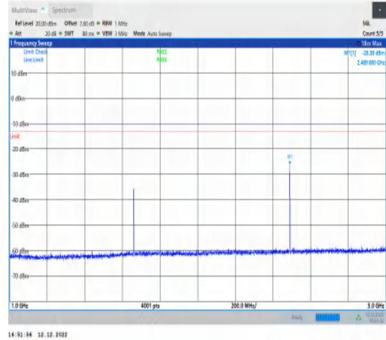
1-N5-15-20-H-1-DFT-PI2BPSK-Inner_1RB_Left-1@1 -1000-3000-Ant1-2489.00--26.38--13-PASS
