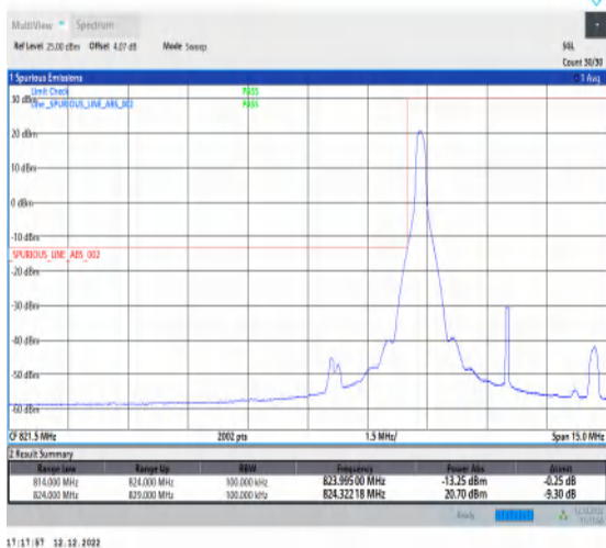
1-N5-15-5-L-1-DFT-PI2BPSK-Edge_1RB_Left-1@0-Ant1-1-seegraph-PASS-see graph
