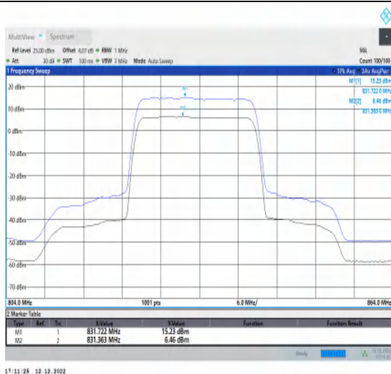
1-N5-15-20-L-1-DFT-256QAM-Outer_Full-100@0-An t1-8.77-100%-0.00-8.77-PASS-≤13
