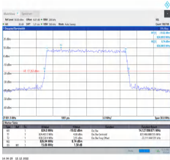
1-N5-15-15-L-9-CP-256QAM-Outer_Full-79@0-Ant1-14.127-15.060≤15-PASS
