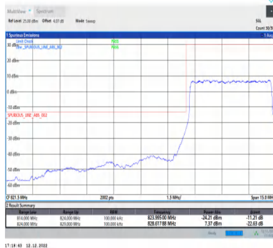
1-N5-15-5-L-3-DFT-PI2BPSK-Outer_Full-25@0-Ant1-1-seegraph-PASS-see graph
