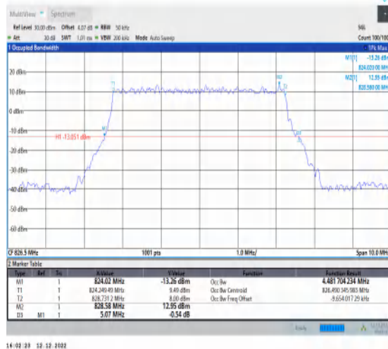
1-N5-15-5-L-2-DFT-PI2BPSK-Outer_Full-25@0-Ant1 -4.482-5.070-≤5-PASS
