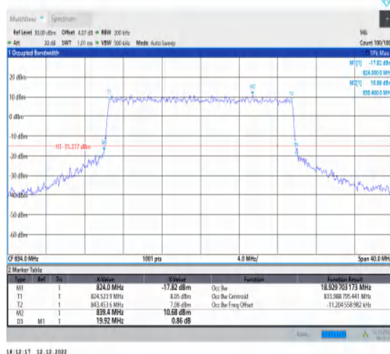
1-N5-15-20-L-7-CP-16QAM-Outer_Full-106@0-Ant1- 18.93-19.920-≤20-PASS
