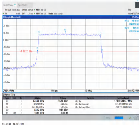
1-N5-15-20-L-5-DFT-256QAM-Outer_Full-100@0-An t1-17.85-18.840-≤20-PASS
