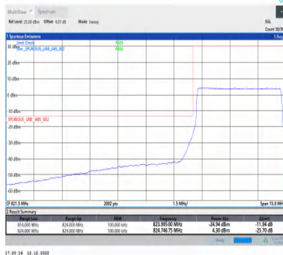
1-N5-15-5-L-6-CP-QPSK-Outer_Full-25@0-Ant1-1-seegraph-PASS-see graph
