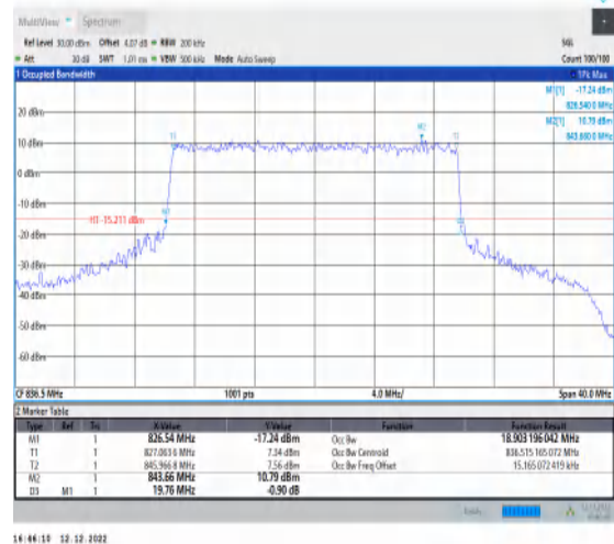
1-N5-15-20-M-6-CP-QPSK-Outer_Full-106@0-Ant1 18.903-19.760-≤20-PASS
