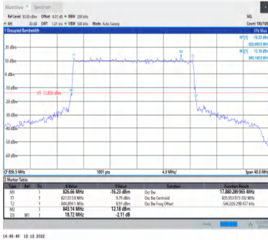
1-N5-15-20-M-3-DFT-16QAM-Outer_Full-100@0-Ant 1-17.88-18.720-≤20-PASS
