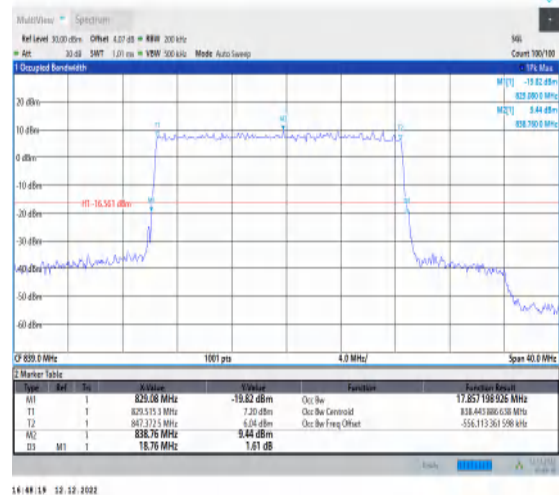
1-N5-15-20-H-5-DFT-256QAM-Outer_Full-100@0-A nt1-17.857-18.760-≤20-PASS
