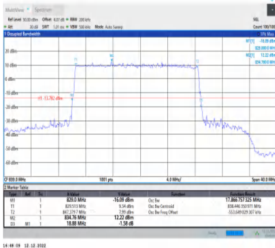
1-N5-15-20-H-4-DFT-64QAM-Outer_Full-100@0-Ant 1-17.867-18.880-≤20-PASS
