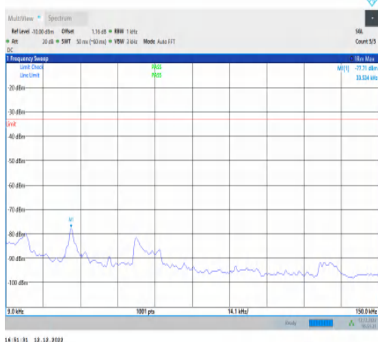
1-N5-15-20-H-1-DFT-PI2BPSK-Inner_1RB_Left-1@1 -0.009-0.15-Ant1-0.03--77.71--33-PASS
