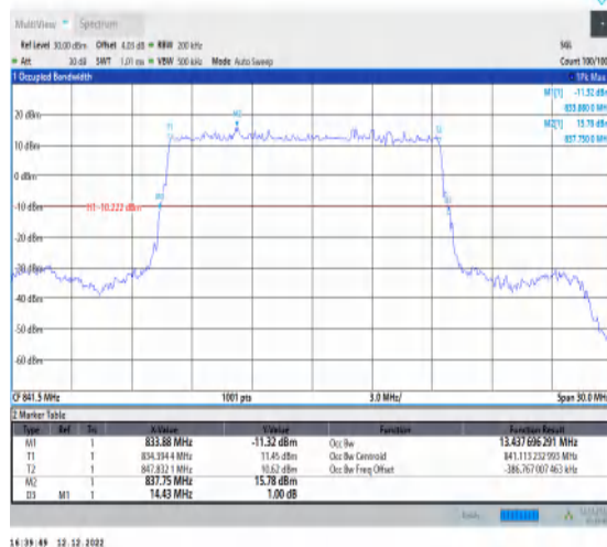
1-N5-15-15-H-2-DFT-PI2BPSK-Outer_Full-75@0-Ant1-13.438-14.430-≤15-PASS
