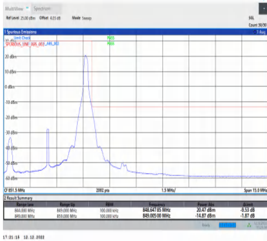
1-N5-15-5-H-2-DFT-PI2BPSK-Edge_1RB_Right-1@24-Ant1-1-seegraph-PASS-see graph
