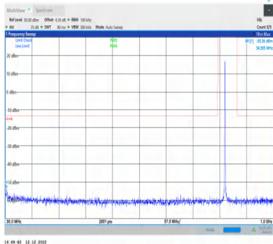
1-N5-15-20-L-1-DFT-PI2BPSK-Inner_1RB_Left-1@1 -30-1000-Ant1-34.37--53.36--13-PASS
