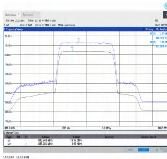
1-N5-15-20-M-2-CP-256QAM-Outer_Full-106@0-Ant t1-9.26-100%-0.00-9.26-PASS-≤13
