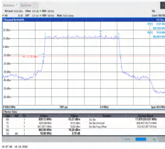
1-N5-15-20-H-2-DFT-PI2BPSK-Outer_Full-100@0-A nt1-17.879-18.680-≤20-PASS
