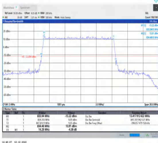
1-N5-15-15-H-3-DFT-16QAM-Outer_Full-75@0-Ant1-13.418-14.280-≤15-PASS
