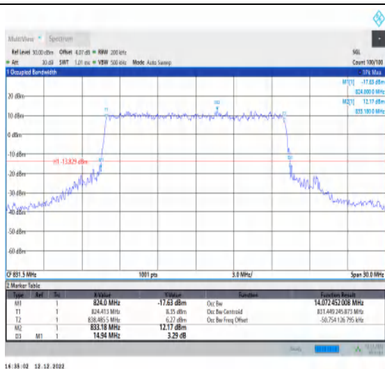
1-N5-15-15-L-7-CP-16QAM-Outer_Full-79@0-Ant1-14.072-14.940≤15-PASS
