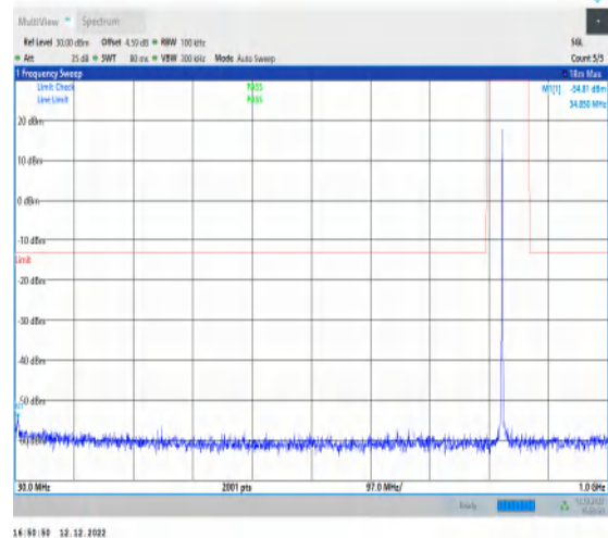
1-N5-15-20-M-1-DFT-PI2BPSK-Inner_1RB_Left-1@ 1-30-1000-Ant1-34.85--54.81--13-PASS
