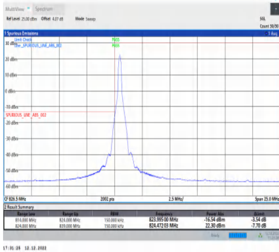
1-N5-15-15-L-1-DFT-PI2BPSK-Edge_1RB_Left-1@0-Ant1-1-seegraph-PASS-see graph
