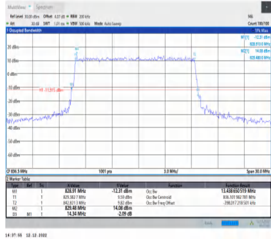
1-N5-15-15-M-3-DFT-16QAM-Outer_Full-75@0-Ant1 -13.439-14.340-≤15-PASS
