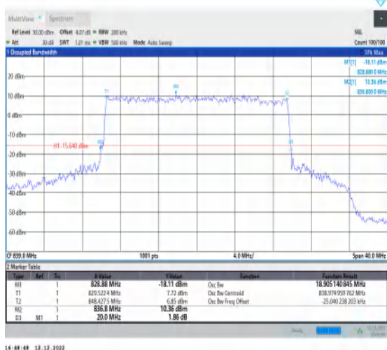
1-N5-15-20-H-8-CP-64QAM-Outer_Full-106@0-Ant1-18.905-20.000-≤20-PASS
