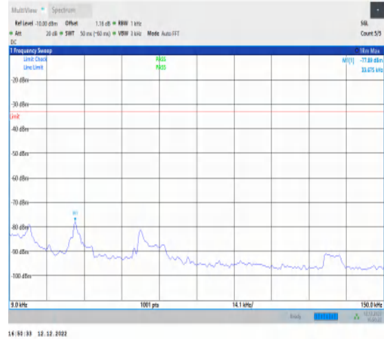
1-N5-15-20-M-1-DFT-PI2BPSK-Inner_1RB_Left-1@ 1-0.009-0.15-Ant1-0.03--77.89--33-PASS
