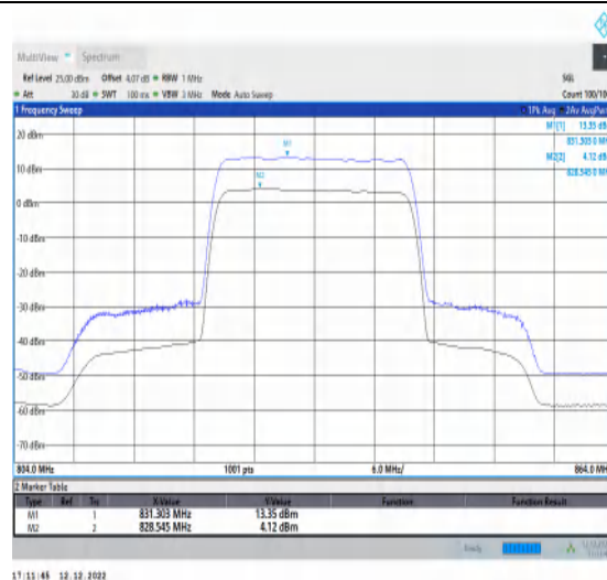
1-N5-15-20-L-2-CP-256QAM-Outer_Full-106@0-Ant t1-9.23-100%-0.00-9.23-PASS-≤13
