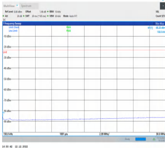
1-N5-15-20-M-1-DFT-PI2BPSK-Inner_1RB_Left-1@ 1-0.15-30-Ant1-0.15--85.25--23-PASS
