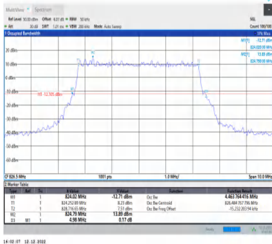
1-N5-15-5-L-1-DFT-QPSK-Outer_Full-25@0-Ant1-4. 464-4.980-≤5-PASS
