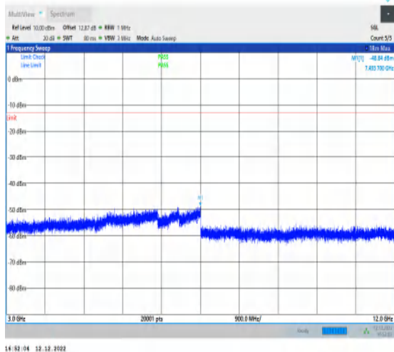
1-N5-15-20-H-1-DFT-PI2BPSK-Inner_1RB_Left-1@1 -3000-12000-Ant1-7493.70--48.84--13-PASS
