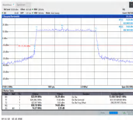
1-N5-15-15-L-1-DFT-QPSK-Outer_Full-75@0-Ant1-1-3.431-14.370-≤15-PASS
