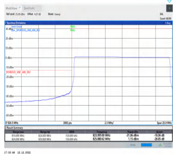
1-N5-15-15-L-6-CP-QPSK-Outer_Full-79@0-Ant1-1-seegraph-PASS-see graph
