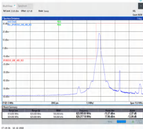
1-N5-15-5-L-4-CP-QPSK-Edge_1RB_Left-1@0-Ant1-1-seegraph-PASS-see graph
