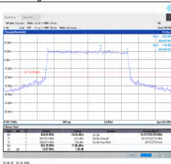
1-N5-15-15-L-8-CP-64QAM-Outer_Full-79@0-Ant1-14.152-14.970≤15-PASS
