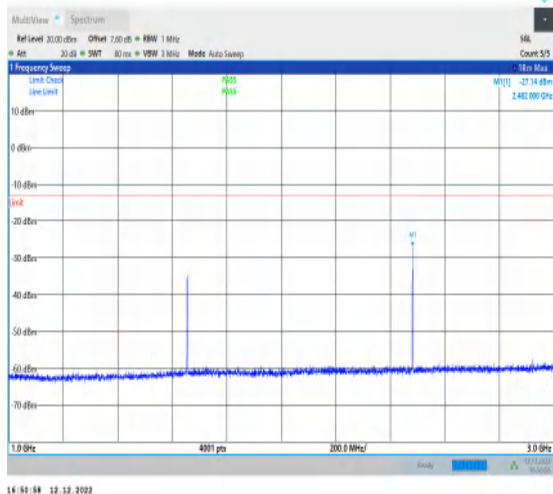
1-N5-15-20-M-1-DFT-PI2BPSK-Inner_1RB_Left-1@ 1-1000-3000-Ant1-2482.00--27.14--13-PASS
