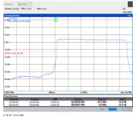
1-N5-15-15-L-3-DFT-PI2BPSK-Outer_Full-75@0-Ant1-1-seegraph-PASS-see graph
