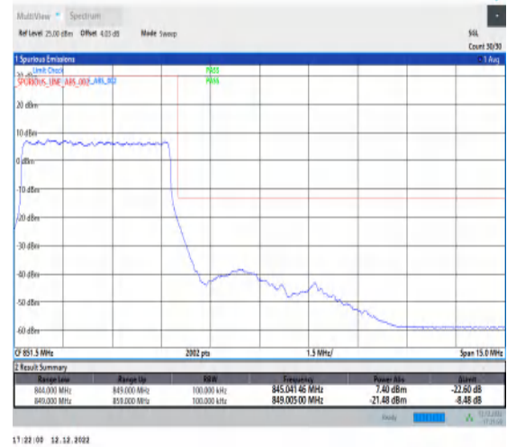
1-N5-15-5-H-3-DFT-PI2BPSK-Outer_Full-25@0-Ant1-1-seegraph-PASS-see graph
