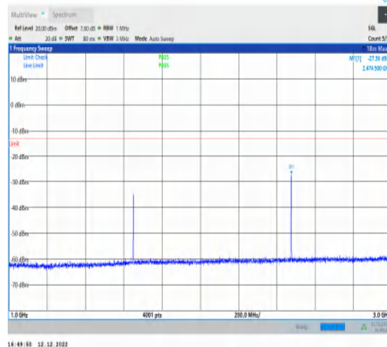
1-N5-15-20-L-1-DFT-PI2BPSK-Inner_1RB_Left-1@1 -1000-3000-Ant1-2474.50--27.36--13-PASS
