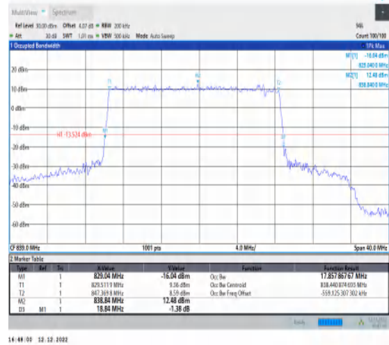
1-N5-15-20-H-3-DFT-16QAM-Outer_Full-100@0-Ant 1-17.858-18.840-≤20-PASS
