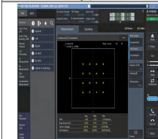
1-N5-15-20-M-7-CP-16QAM-Outer_Full-106@0-Ant1-see graph-PASS
