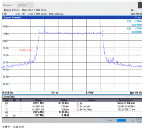
1-N5-15-15-M-4-DFT-64QAM-Outer_Full-75@0-Ant1 -13.455-14.370-≤15-PASS
