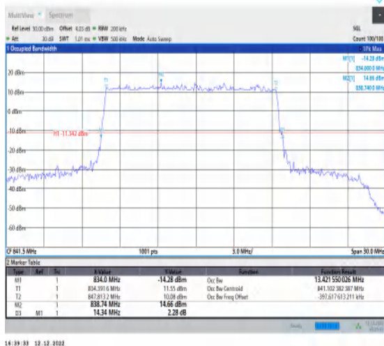
1-N5-15-15-H-1-DFT-QPSK-Outer_Full-75@0-Ant1-13.422-14.340-≤15-PASS
