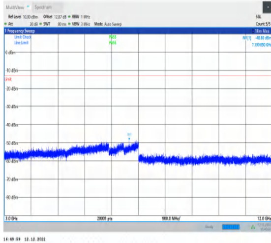
1-N5-15-20-L-1-DFT-PI2BPSK-Inner_1RB_Left-1@ -3000-12000-Ant1-7190.85--48.80--13-PASS
