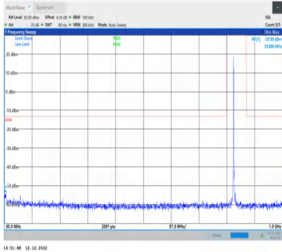
1-N5-15-20-H-1-DFT-PI2BPSK-Inner_1RB_Left-1@1 -30-1000-Ant1-33.88--53.99--13-PASS
