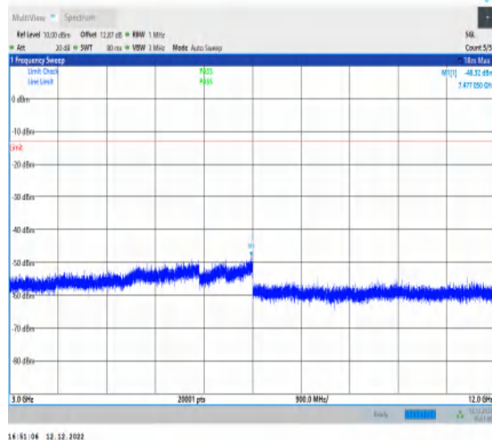
1-N5-15-20-M-1-DFT-PI2BPSK-Inner_1RB_Left-1@ 1-3000-12000-Ant1-7477.05--48.32--13-PASS
