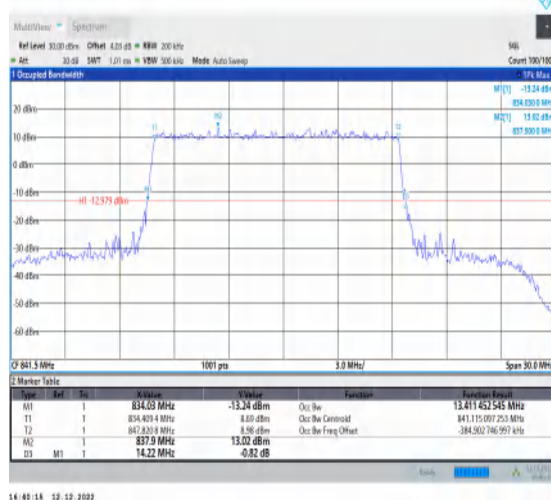
1-N5-15-15-H-4-DFT-64QAM-Outer_Full-75@0-Ant1-13.411-14.220-≤15-PASS
