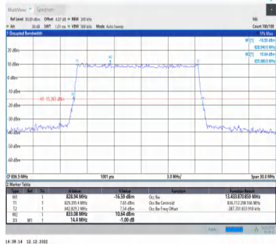
1-N5-15-15-M-5-DFT-256QAM-Outer_Full-75@0-Ant 1-13.434-14.400-≤15-PASS
