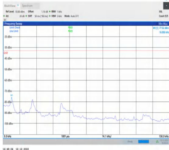
1-N5-15-20-L-1-DFT-PI2BPSK-Inner_1RB_Left-1@1 -0.009-0.15-Ant1-0.02--77.52--33-PASS
