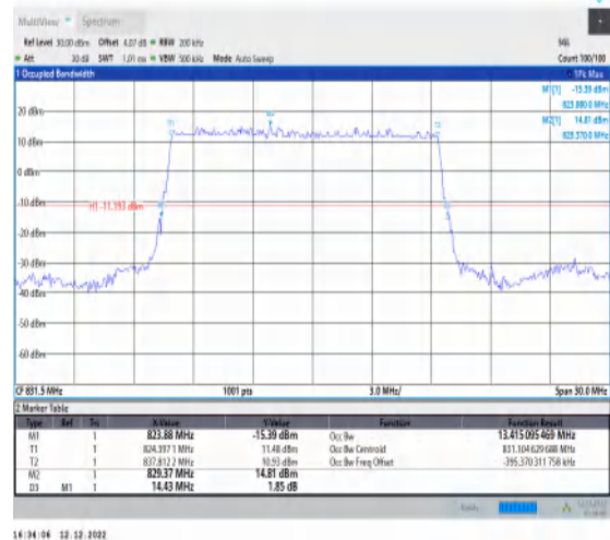
1-N5-15-15-L-2-DFT-PI2BPSK-Outer_Full-75@0-Ant1-1-13.415-14.430-≤15-PASS
