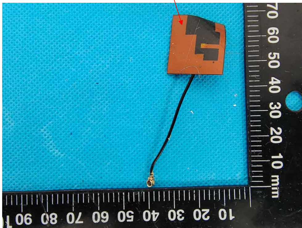
BLE&2.4G WiFi Antenna(FPC)
