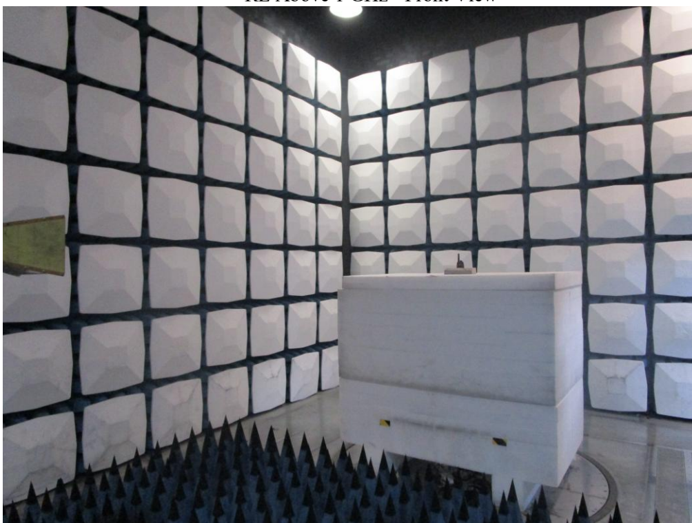
RE Above 1 GHz - Front View
