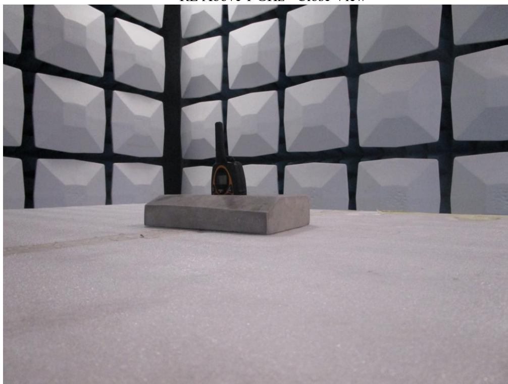
RE Above 1 GHz - Close View
