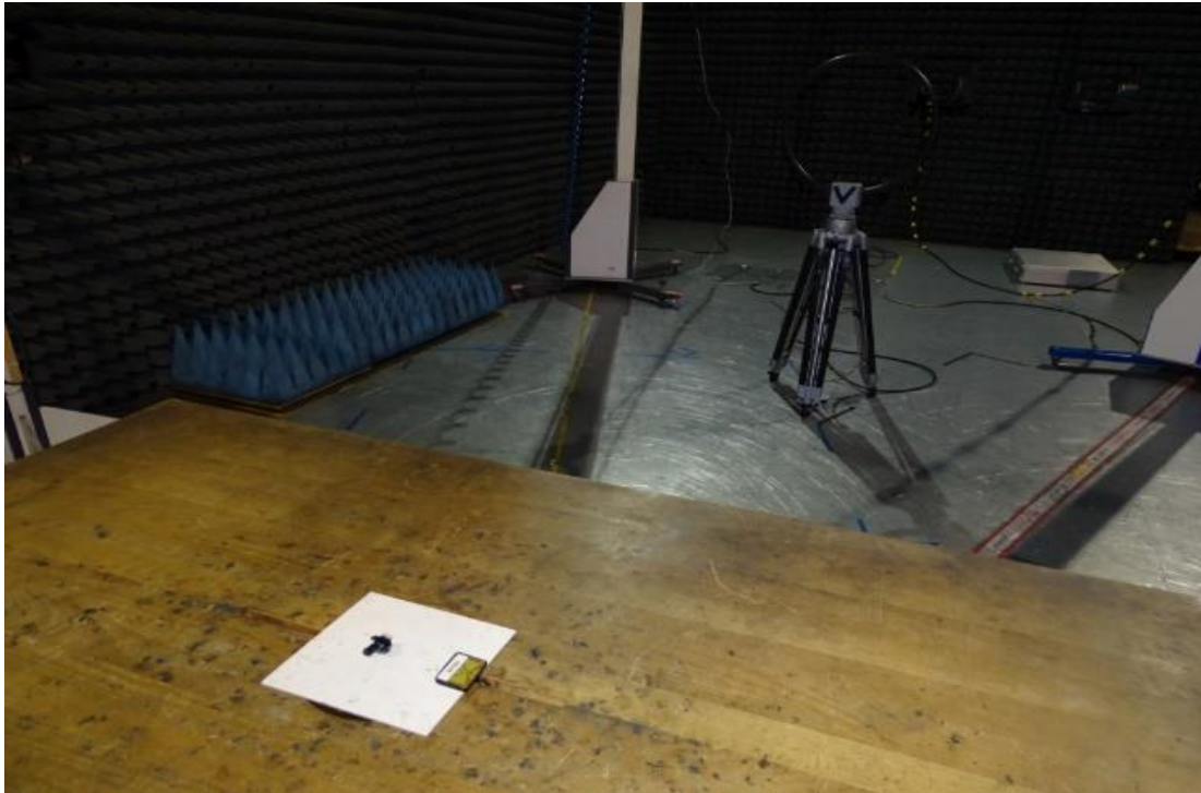
Photo 1: Test setup for radiated measurements (Enclosure, below 30 MHz, intentional radiator §15, ANSI C63.10)
