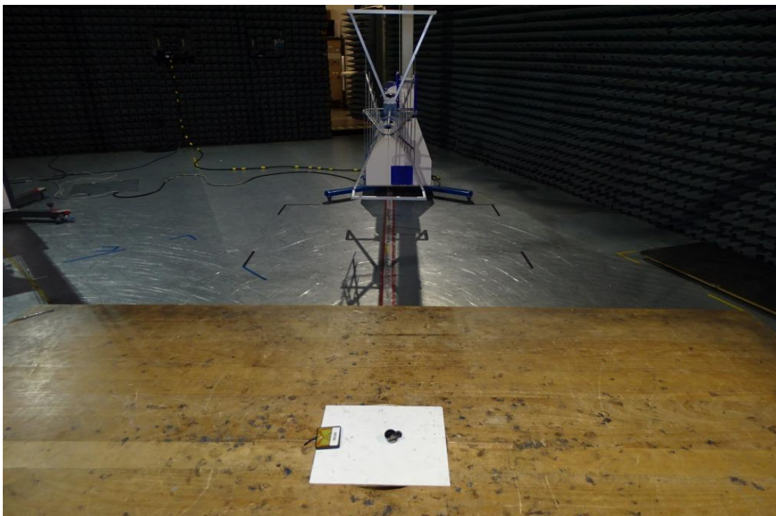
Photo 2: Test setup for radiated measurements (Enclosure, semi-anechoic chamber, 30 MHz to 1 GHz, intentional radiator §15, ANSI C63.10)
