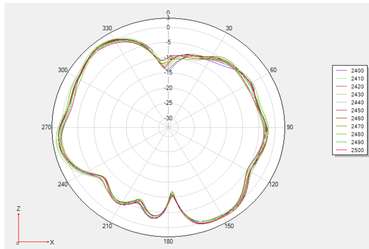
Phi 90 2D
