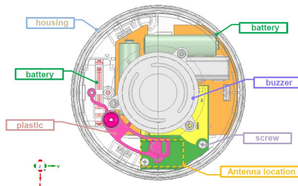
▲ Antenna Simulation Structure
