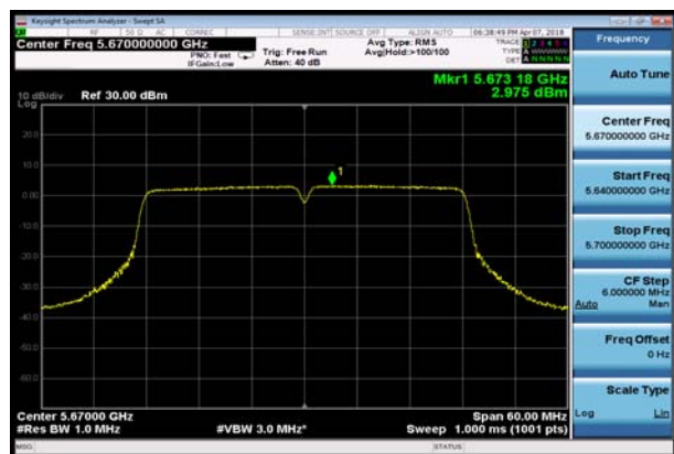
U-NII-2C, 802.11n HT40, Channel No.: 134
