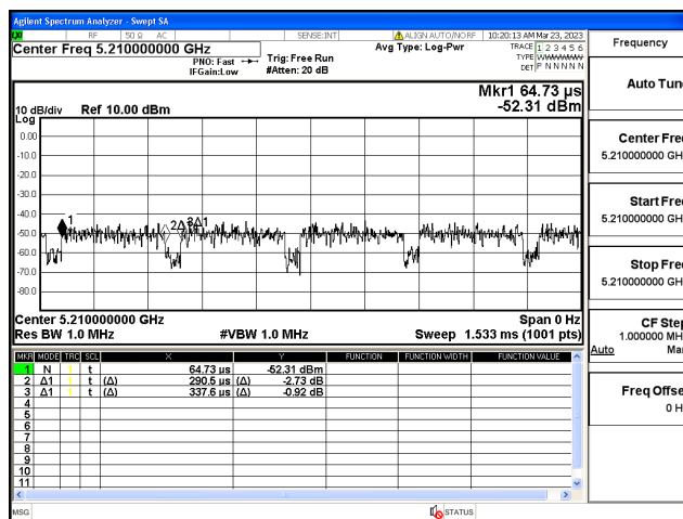
802.11ac (80 MHz)
