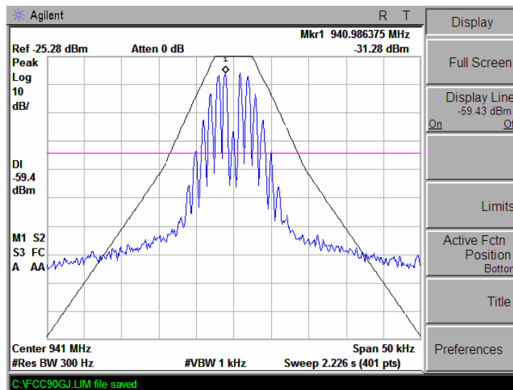
Plot 7.3.13 Emission mask measurements according to §90. 210(g) at high frequency carrier. Port 3
