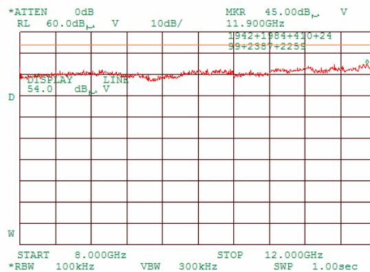
Plot 8.1.8 Radiated emission measurements in 8000- 12000 MHz range, horizontal antenna polarization, SMR uplink mode
