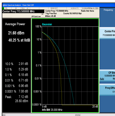
Band12-5MHz-QPSK-23155-1RB#0-PASS
