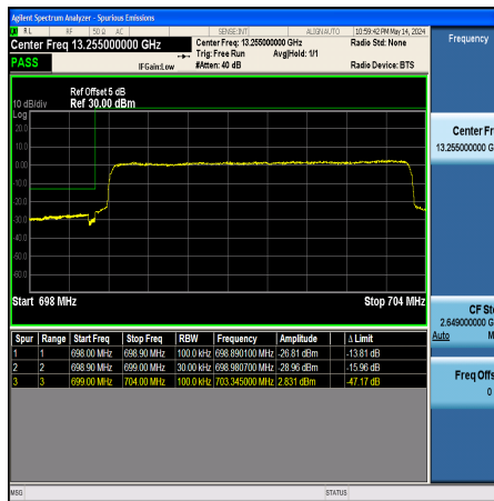
Band12_5MHz_QPSK_23035_25RB#0
