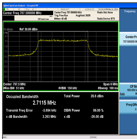
Band12-3MHz-QPSK-23095-15RB#0-PASS
