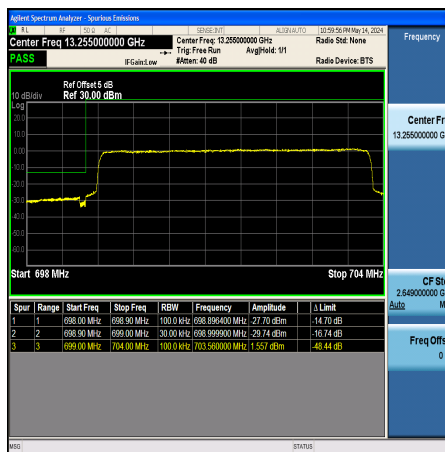
Band12_5MHz_16QAM_23035_25RB#0
