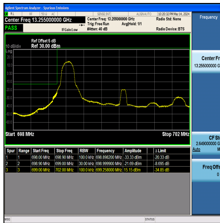
Band12_3MHz_16QAM_23025_1RB#0
