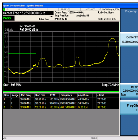
Band12_3MHz_QPSK_23025_1RB#14
