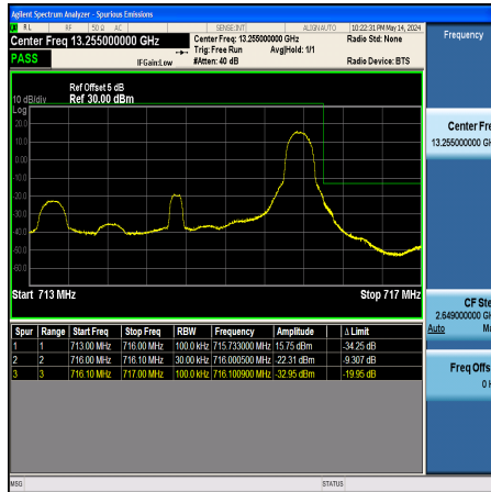
Band12_3MHz_16QAM_23165_1RB#14
