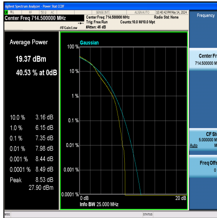
Band12-3MHz-16QAM-23165-1RB#0-PASS
