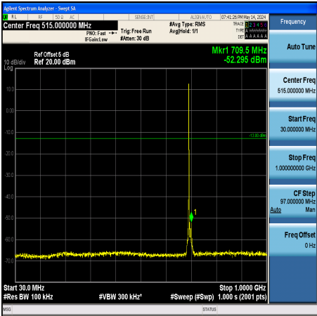
Band12_1.4MHz_QPSK_23017_1RB#0_30~1000_30~1000
