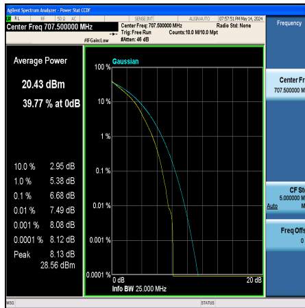
Band12-1.4MHz-QPSK-23095-6RB#0-PASS
