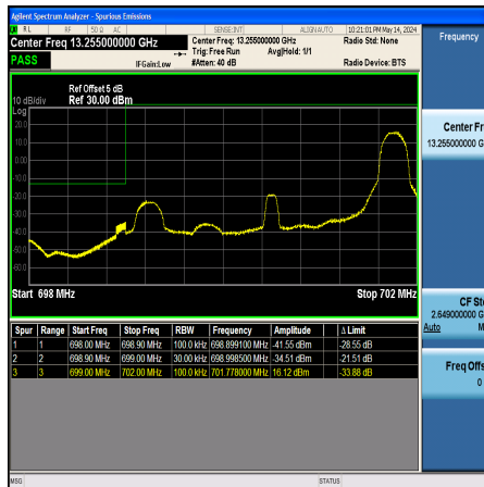
Band12_3MHz_16QAM_23025_1RB#14
