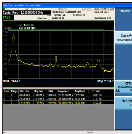
Band12_10MHz_QPSK_23130_1RB#0
