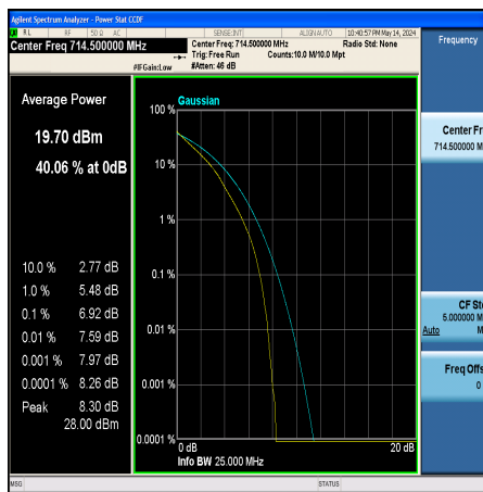
Band12-3MHz-QPSK-23165-15RB#0-PASS
