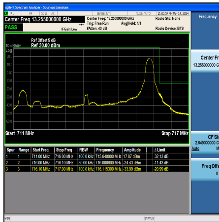
Band12_5MHz_16QAM_23155_1RB#24
