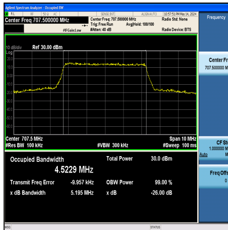
Band12-5MHz-16QAM-23095-25RB#0-PASS
