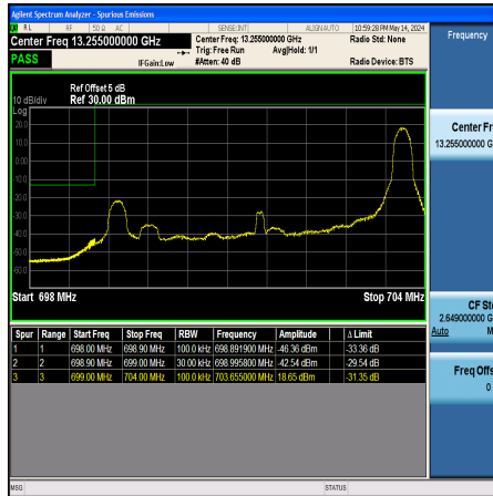
Band12_5MHz_16QAM_23035_1RB#24
