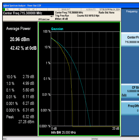
Band12-1.4MHz-QPSK-23173-1RB#0-PASS
