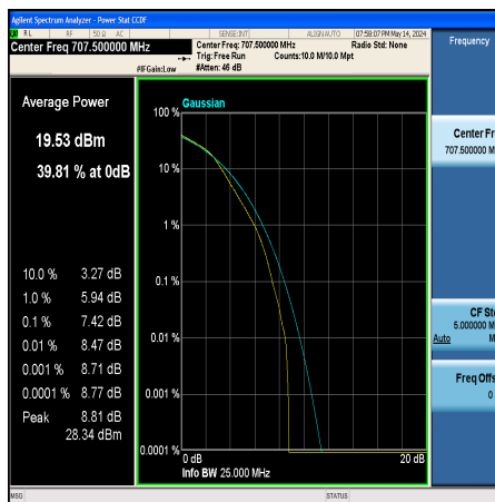
Band12-1.4MHz-16QAM-23095-6RB#0-PASS
