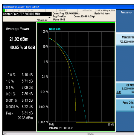
Band12-5MHz-16QAM-23095-25RB#0-PASS
