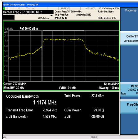
Band12-1.4MHz-16QAM-23095-6RB#0-PASS
