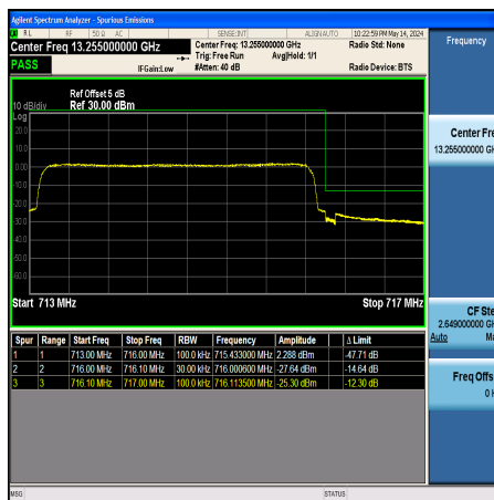
Band12_3MHz_16QAM_23165_15RB#0
