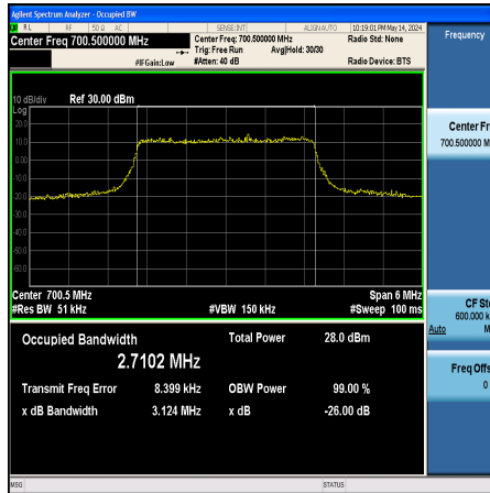
Band12-3MHz-QPSK-23025-15RB#0-PASS
