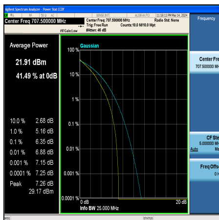
Band12-5MHz-QPSK-23095-25RB#0-PASS
