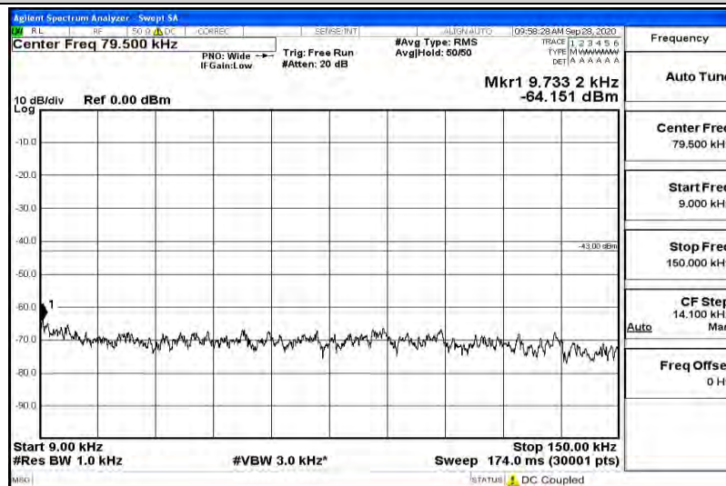
Band66-5MHz-16QAM-132322-1RB#0-Range2:0.15~30MHz
