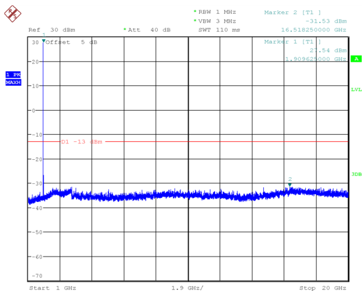
Channel 810: 1GHz~20GHz
