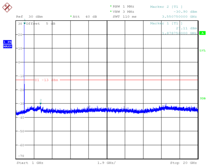
Channel 661: 1GHz~20GHz
