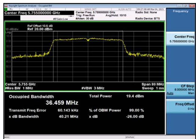
U-NII-3 99% Bandwidth-802.11n(40MHz) ,5755MHz
