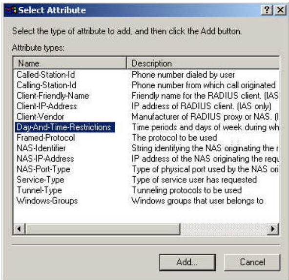
Figure 30: Attribute Screen
