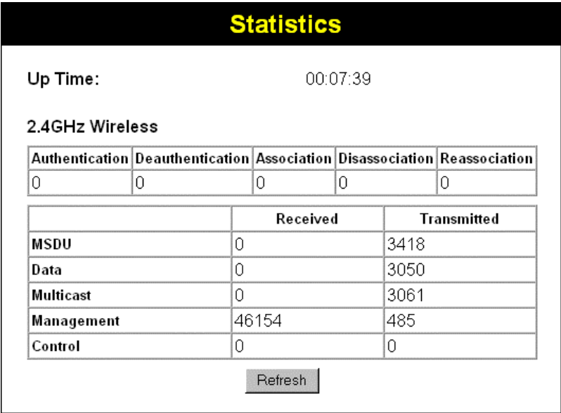
Figure 46: Statistics Screen
