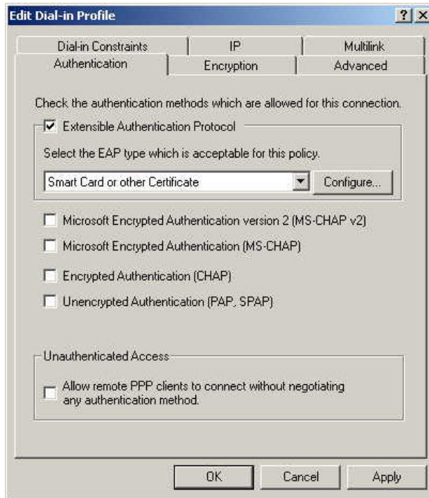
Figure 31: Authentication Screen
