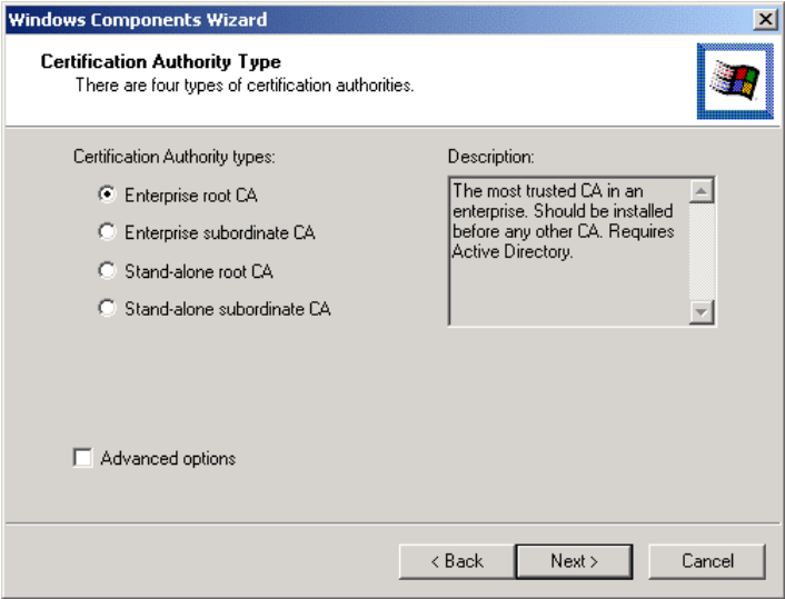
Figure 18: Certification Screen
