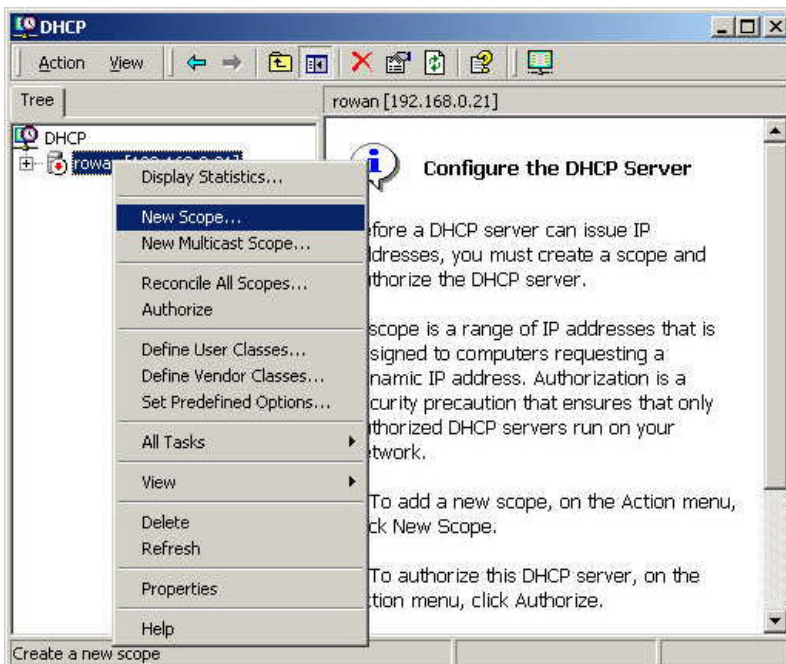
Figure 20: DHCP Screen
