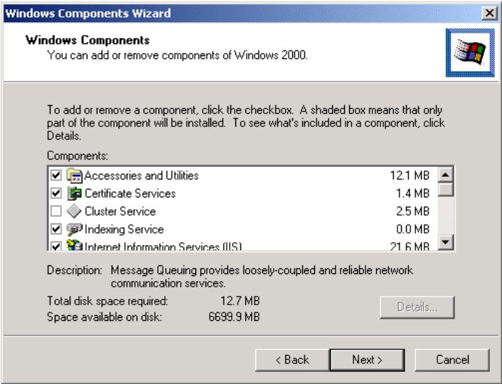
Figure 17: Components Screen
