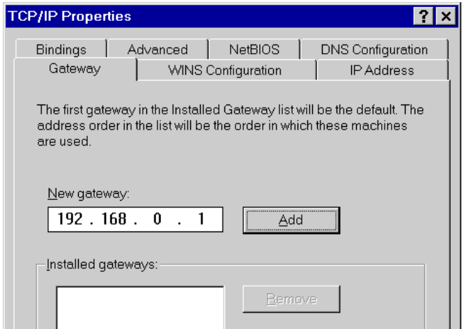
Figure 54: Gateway Tab
