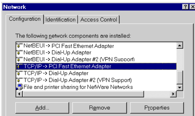
Figure 52: Network Configuration
