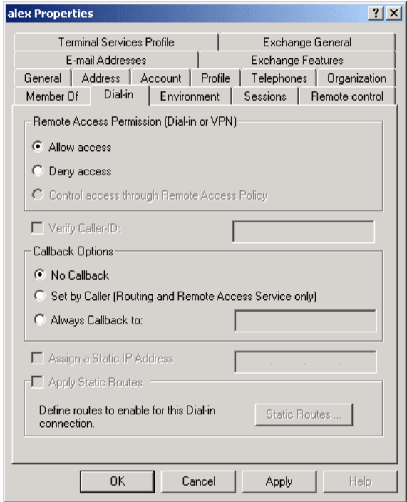
Figure 32: Dial-in Screen
