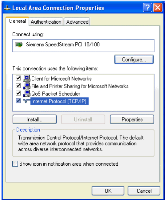
Figure 62: Network Configuration (Windows XP)
