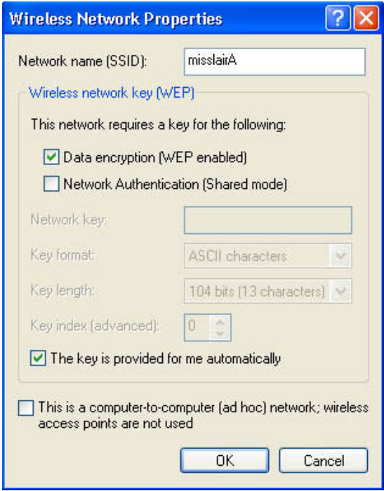
Figure 41: Properties Screen
