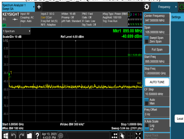
Plot 8-427. Conducted Spurious Emission Plot 895 MHz to 1 GHz
