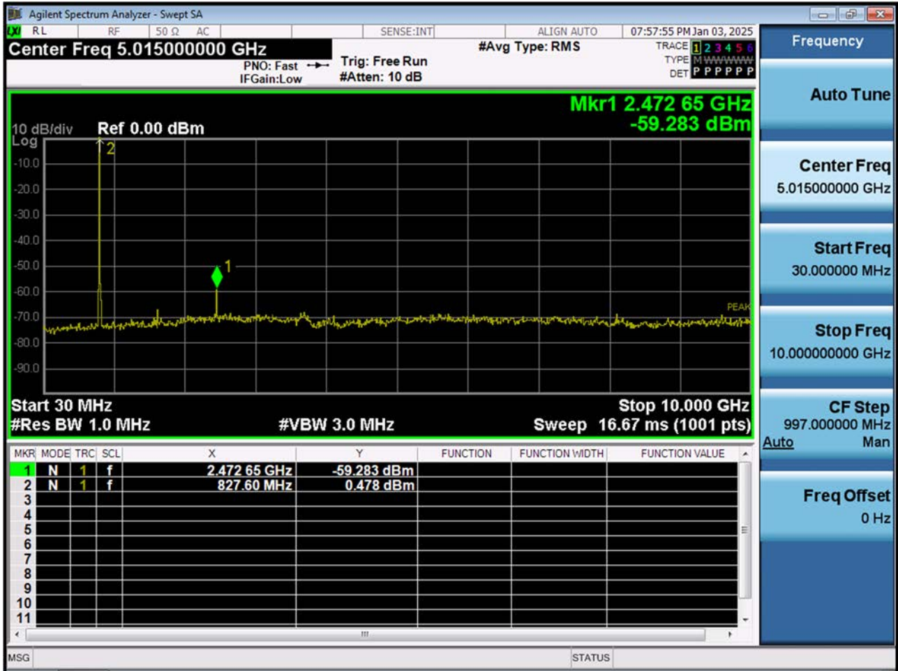
BAND 26. Conducted Spurious Plot (26815ch_5 MHz_QPSK_RB 1_0)
