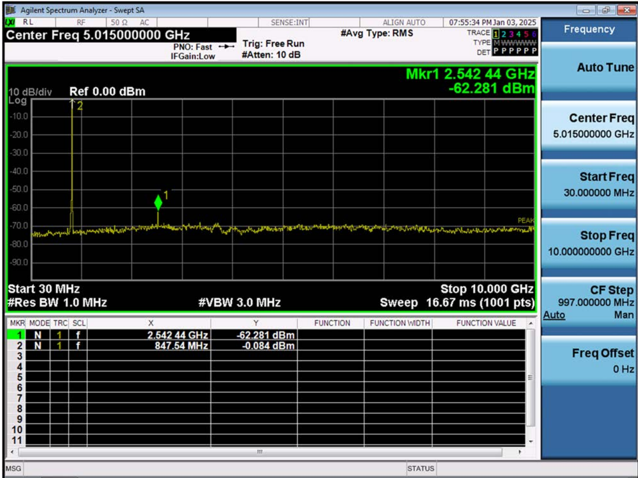
BAND 26. Conducted Spurious Plot (27025ch_3 MHz_QPSK_RB 1_0)
