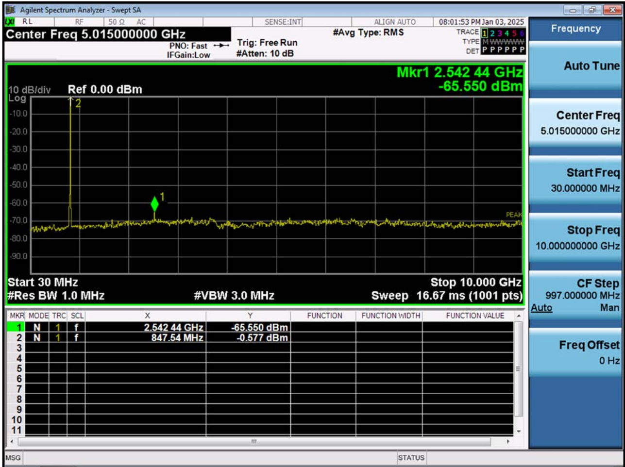
BAND 26. Conducted Spurious Plot (27015ch_5 MHz_QPSK_RB 1_0)
