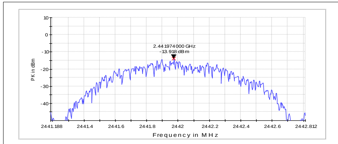
Channel 20 / 2442 MHz
