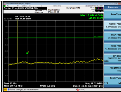
LTE Band 4_5MHz_CH20175 Spectrum Plot
