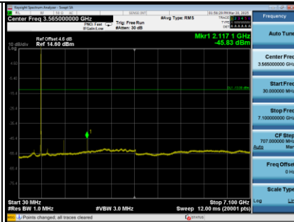
LTE Band 17_10MHz_CH23790 Spectrum Plot
