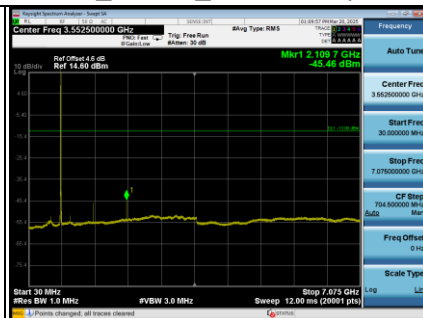
LTE Band 12_10MHz_CH23095 Spectrum Plot
