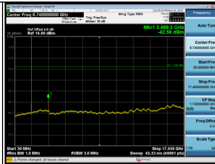
LTE Band 66_5MHz_CH132322 Spectrum Plot
