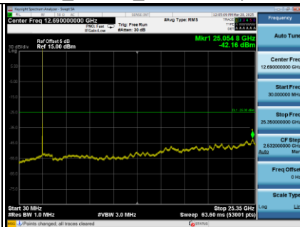
LTE Band 7_20MHz_CH21100 Spectrum Plot
