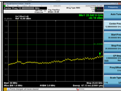
LTE Band 41_20MHz_CH40620 Spectrum Plot
