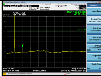
LTE Band 71_20MHz_CH133322 Spectrum Plot
