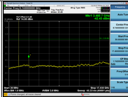
LTE Band 66_20MHz_CH132322 Spectrum Plot
