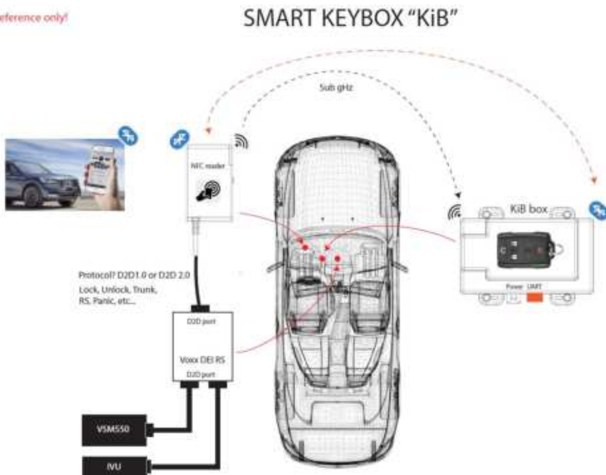
Figure 1 EKey System Diagram
