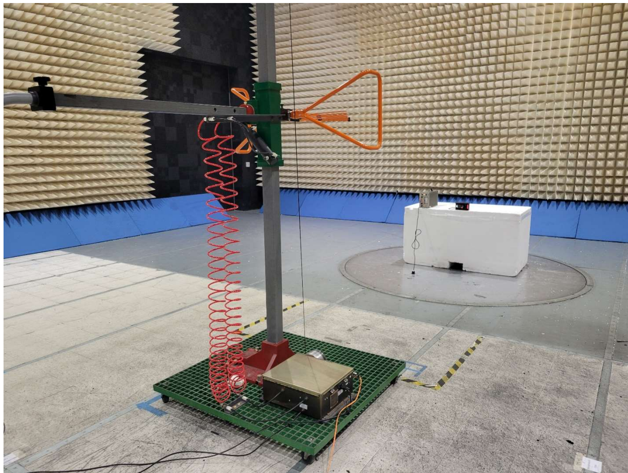
RSE 30MHz – 1GHz
