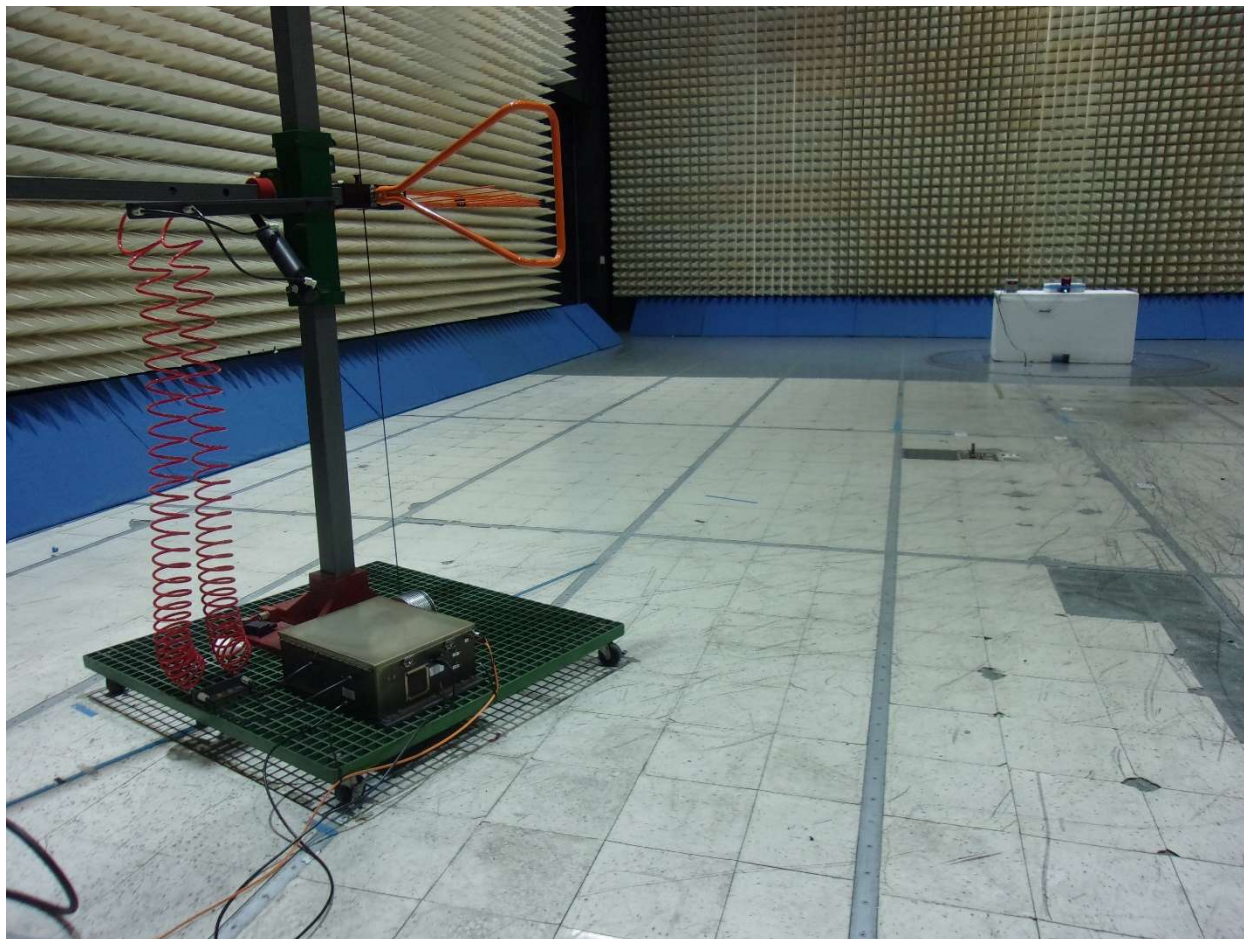
Unintentional Emissions 30MHz – 1GHz
