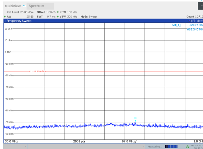
BLE_1M_Ant6_2402_30~1000
