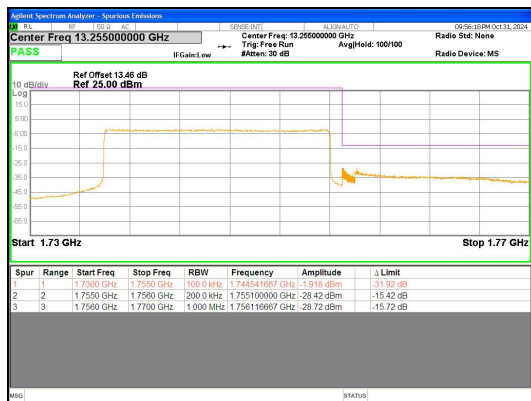
Band 4 20MHz/1745.0/High QPSK 1@0
