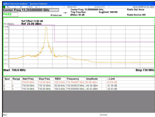
Band 12 1.4MHz/715.3/High QPSK 1@0
