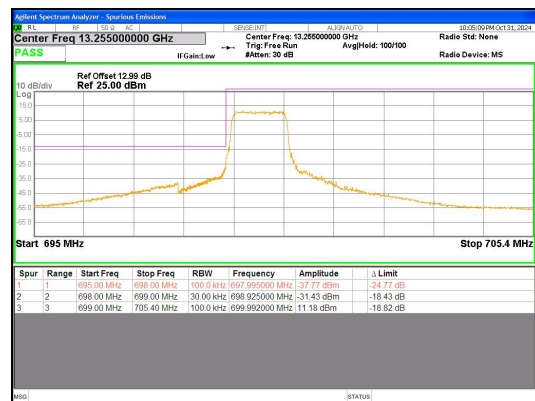
Band 12 1.4MHz/699.7/Low 16QAM 1@0
