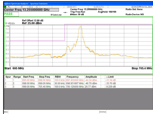
Band 12 1.4MHz/699.7/Low QPSK 1@5
