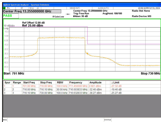
Band 12 10MHz/711.0/High QPSK 1@0
