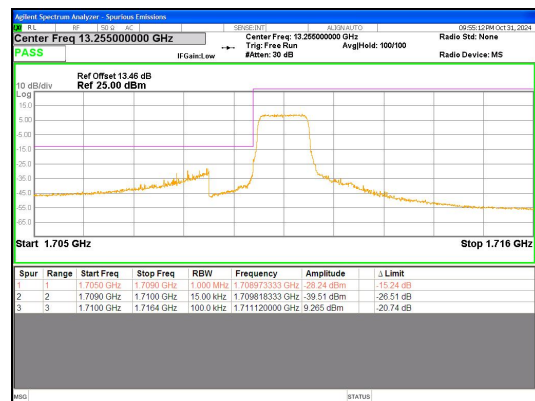
Band 4 1.4MHz/1710.7/Low 16QAM 1@0
