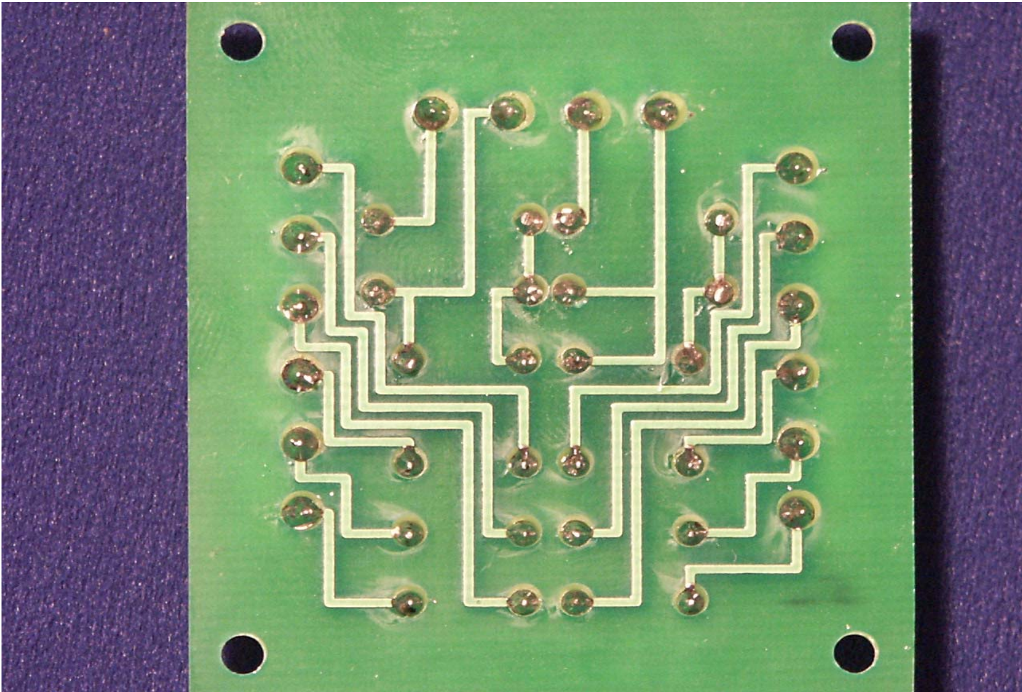
20-001602 (24 V Relay Board Back)
