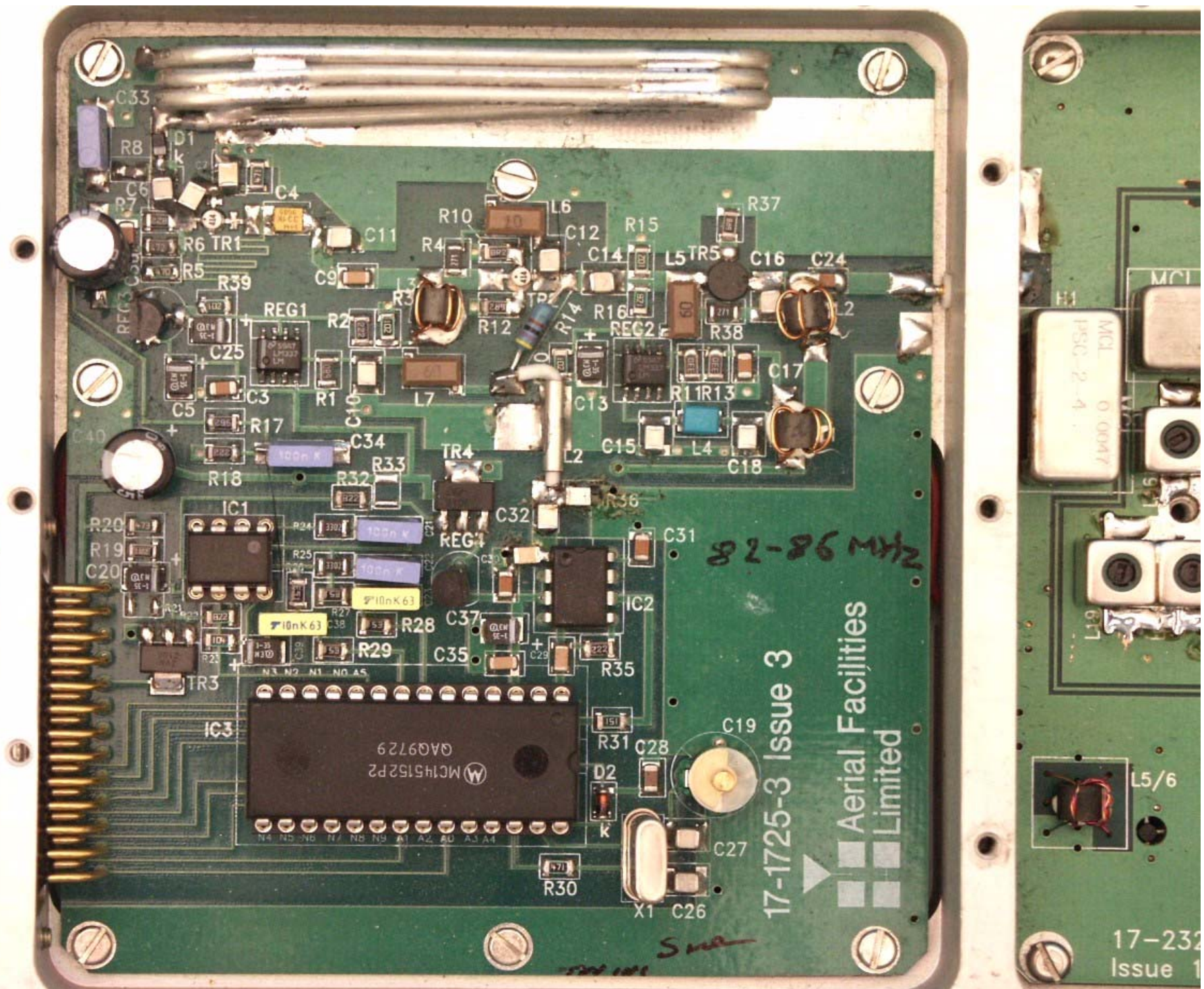
17-003006 (Channel Module Synth Side)
