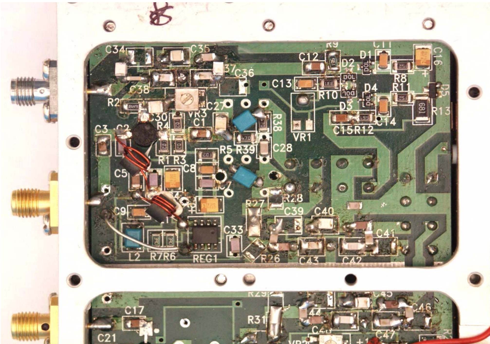
17-003006 (Channel Module Input Back Side)
