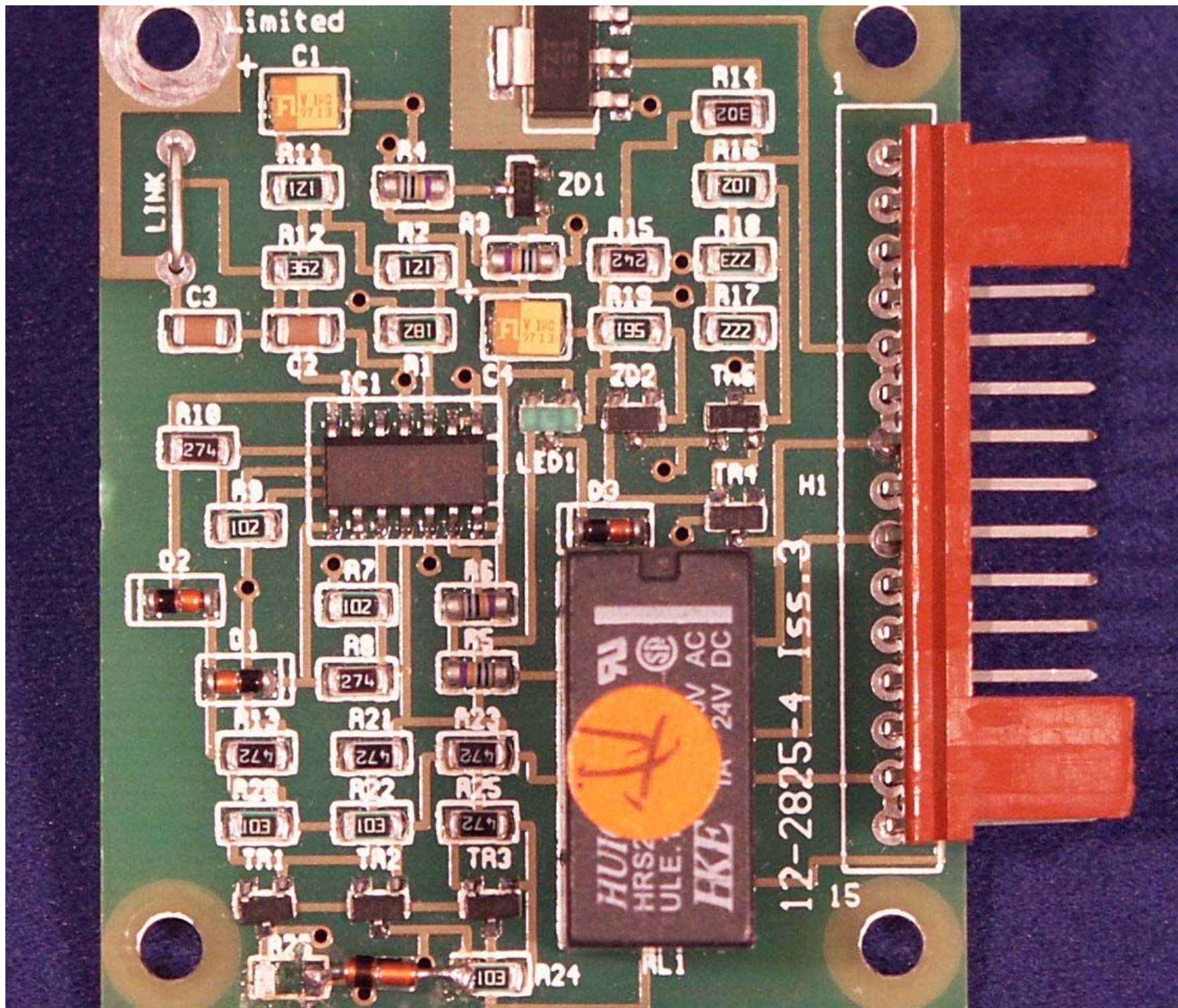
12-002801 (Single Alarm)
