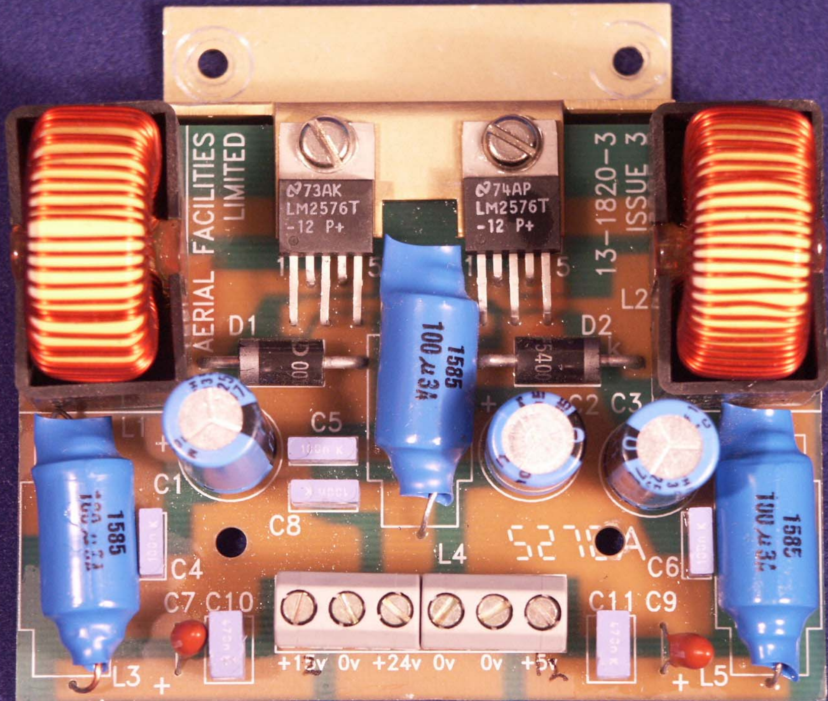
13-001803 (DC/DC Converter Front)
