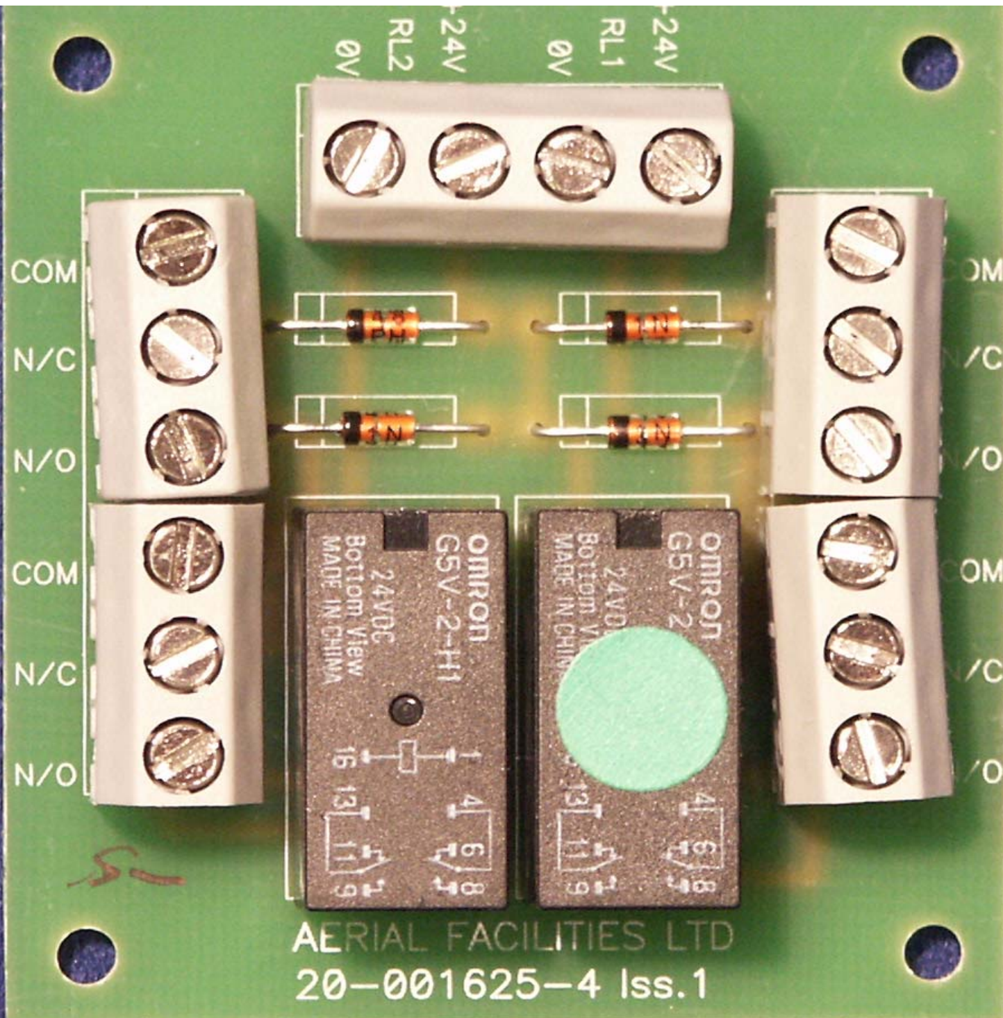
20-001602 (24V Relay board Front)
