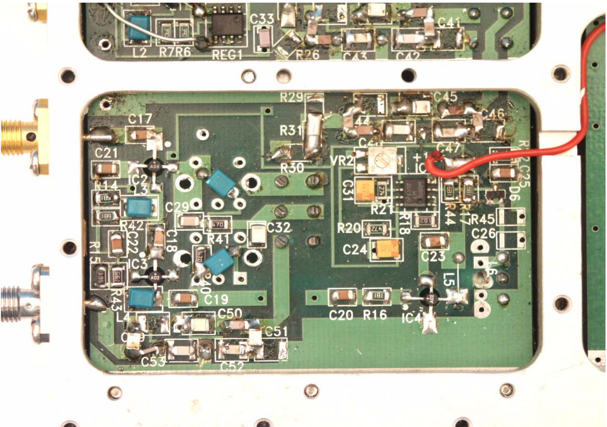
17-003006 (Channel Module Output Back Side)
