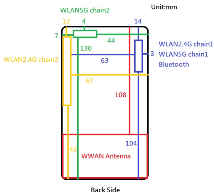
Fig.23 Antenna position of EUT
