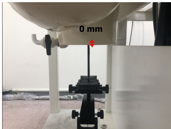
Fig.20 EUT Top side to flat phantom
