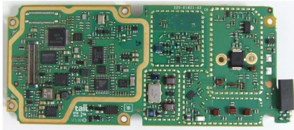
Photograph 03: Rx-Tx PCB - top (without shields)
