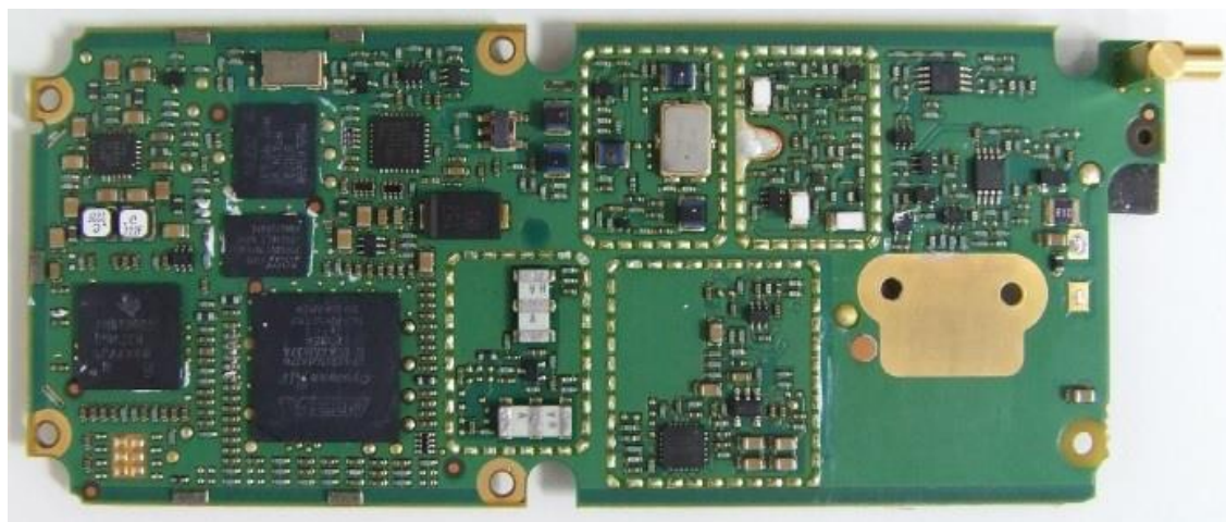
Photograph 05: Rx-Tx PCB - bottom (without shields)
