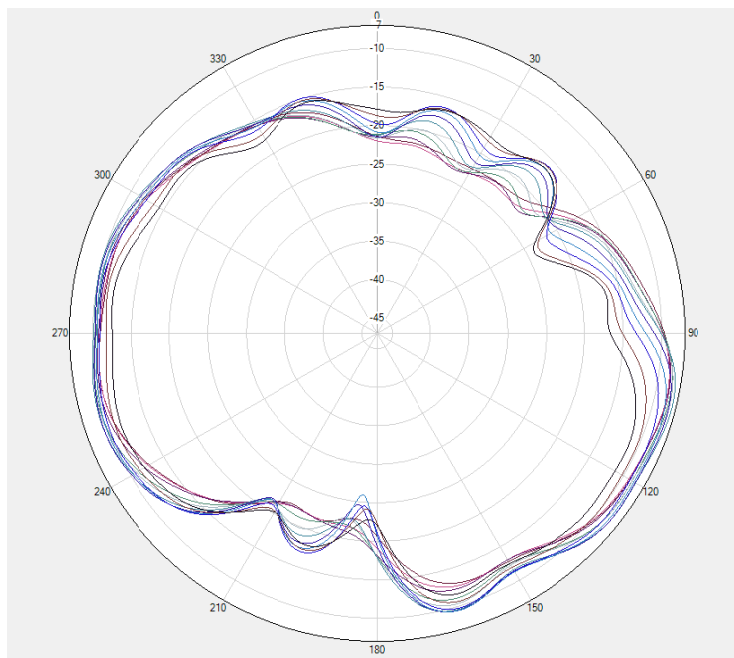
LTE B12/B17/B13/B26/B28 \Phi=90^\circ
