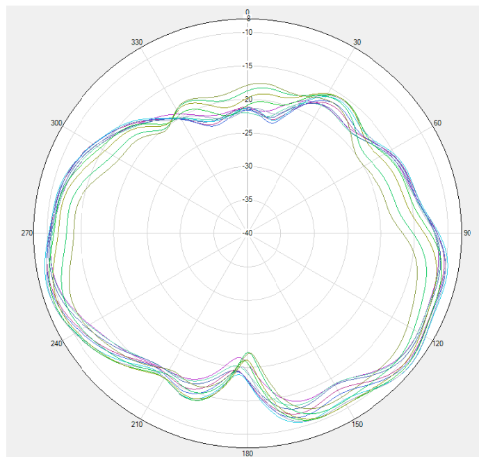
LTEB12/B17/B13/B26/B28 \Phi=0^\circ
