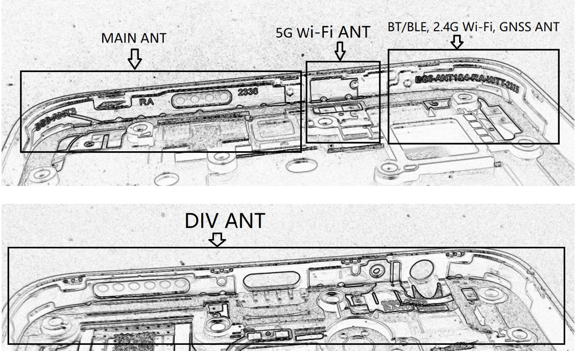
Antenna Photo:
