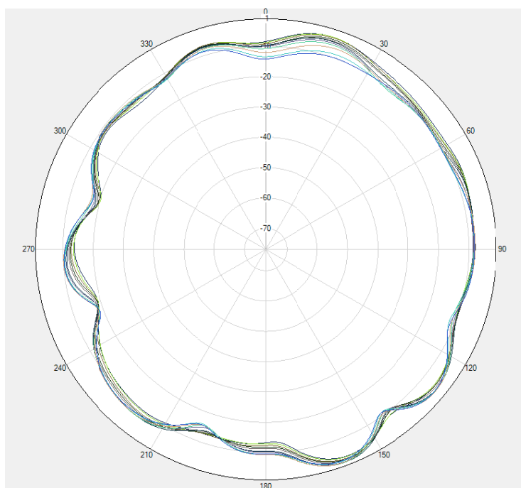
LTE B7/B38/41 \Phi=0^\circ
