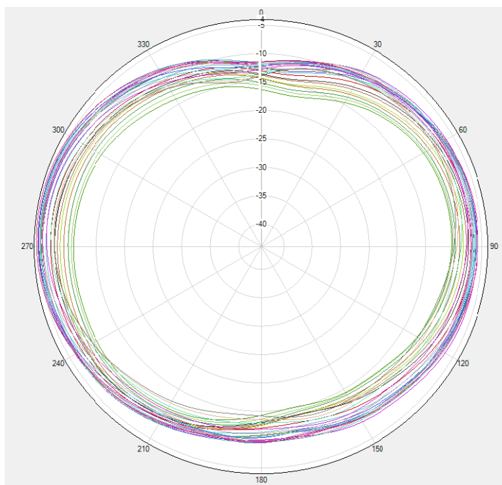
DCS1800/PCS1900/WCDMA B1/B2LTE B1/B2/B3/B4/B66 \Theta=90^\circ
