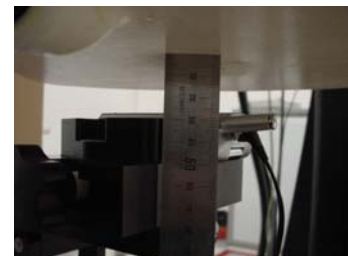
Fig. 20. Body SAR Test Setup with Holster
