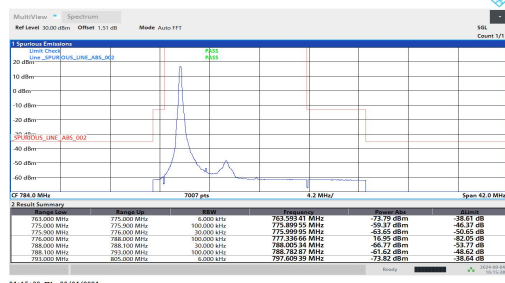
Band13-5MHz-QPSK-23205-1RB#0-PASS
