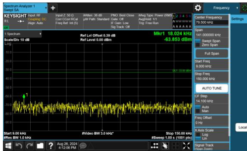
Band13-10MHz-QPSK-23230-1RB#49-0.009~0.15-PASS
