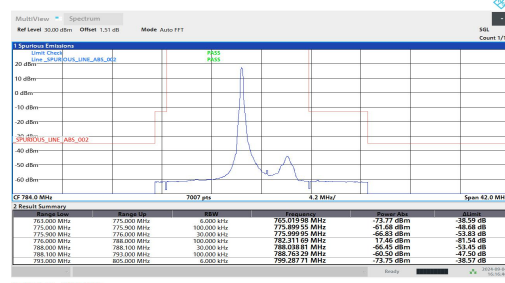
Band13-5MHz-QPSK-23255-1RB#0-PASS
