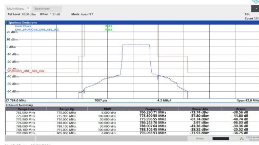
Band13-5MHz-QPSK-23255-25RB#0-PASS
