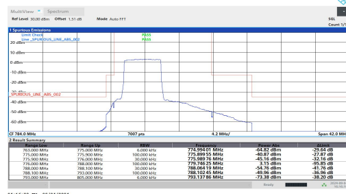
Band13-5MHz-QPSK-23205-25RB#0-PASS
