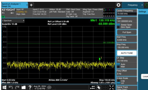
Band13-10MHz-QPSK-23230-50RB#0-0.009~0.15-PASS
