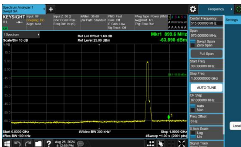
Band13-10MHz-QPSK-23230-50RB#0-30~1000-PASS
