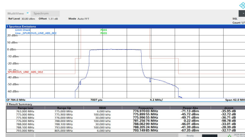
Band13-10MHz-QPSK-23230-50RB#0-PASS
