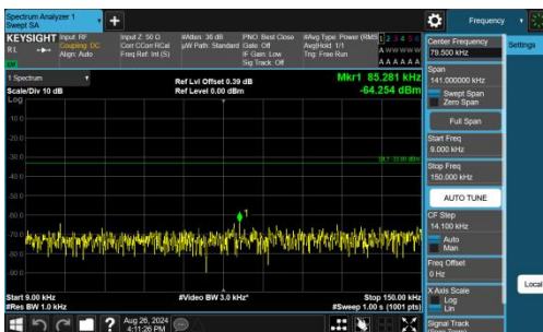
Band13-10MHz-QPSK-23230-1RB#0-0.009~0.15-PASS
