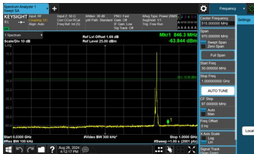
Band13-10MHz-QPSK-23230-1RB#49-30~1000-PASS
