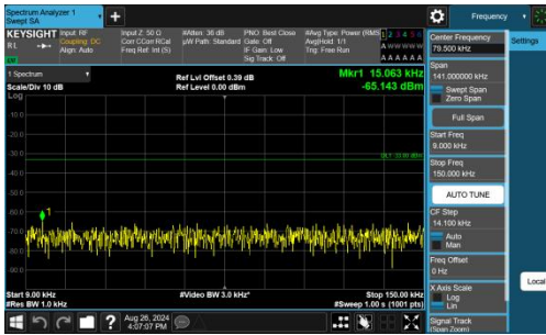
Band13-5MHz-QPSK-23230-1RB#24-0.009~0.15-PASS
