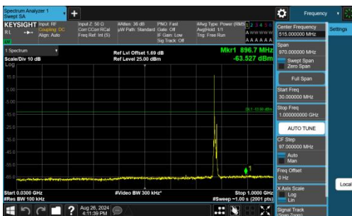
Band13-10MHz-QPSK-23230-1RB#0-30~1000-PASS
