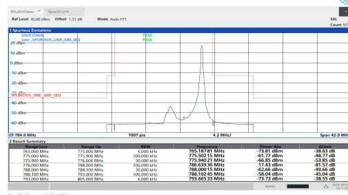
Band13-5MHz-QPSK-23255-1RB#24-PASS
