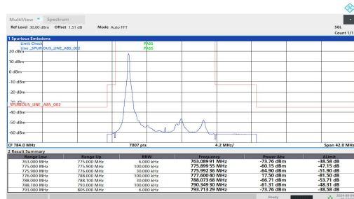
Band13-10MHz-QPSK-23230-1RB#0-PASS
