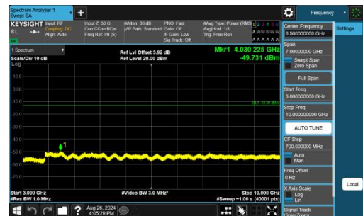
Band13-5MHz-QPSK-23205-1RB#0-3000~10000-PASS
