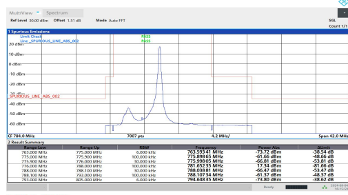
Band13-5MHz-QPSK-23205-1RB#24-PASS
