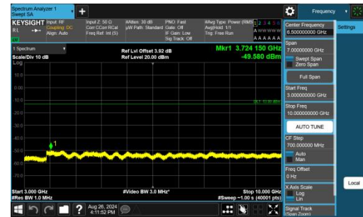
Band13-10MHz-QPSK-23230-1RB#0-3000~10000-PASS
