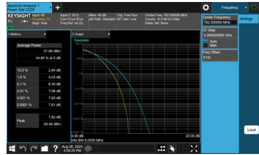
Band13-5MHz-16QAM-23230-25RB#0-PASS
