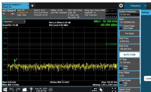
Band13-5MHz-QPSK-23255-1RB#24-0.009~0.15-PASS
