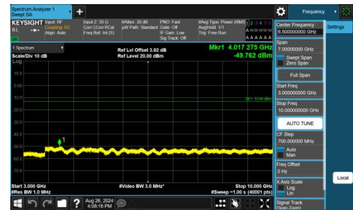
Band13-5MHz-QPSK-23255-1RB#0-3000~10000-PASS
