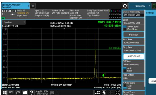
Band13-5MHz-QPSK-23230-1RB#0-30~1000-PASS
