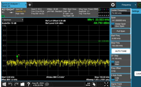
Band13-5MHz-QPSK-23230-1RB#0-0.009~0.15-PASS
