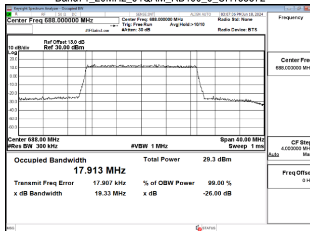
Band71_20MHz_64QAM_RB100_0_CH133372
