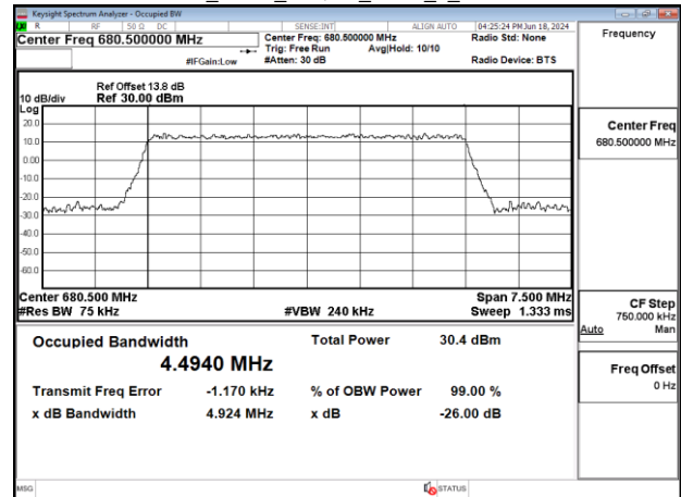
Band71_5MHz_16QAM_RB25_0_CH133447
