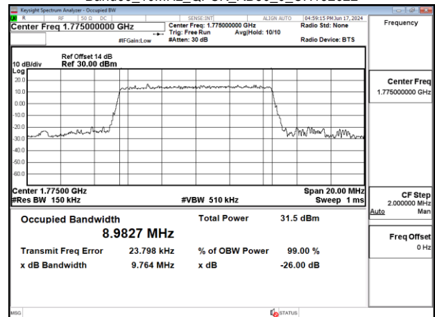
Band66_10MHz_QPSK_RB50_0_CH132622
